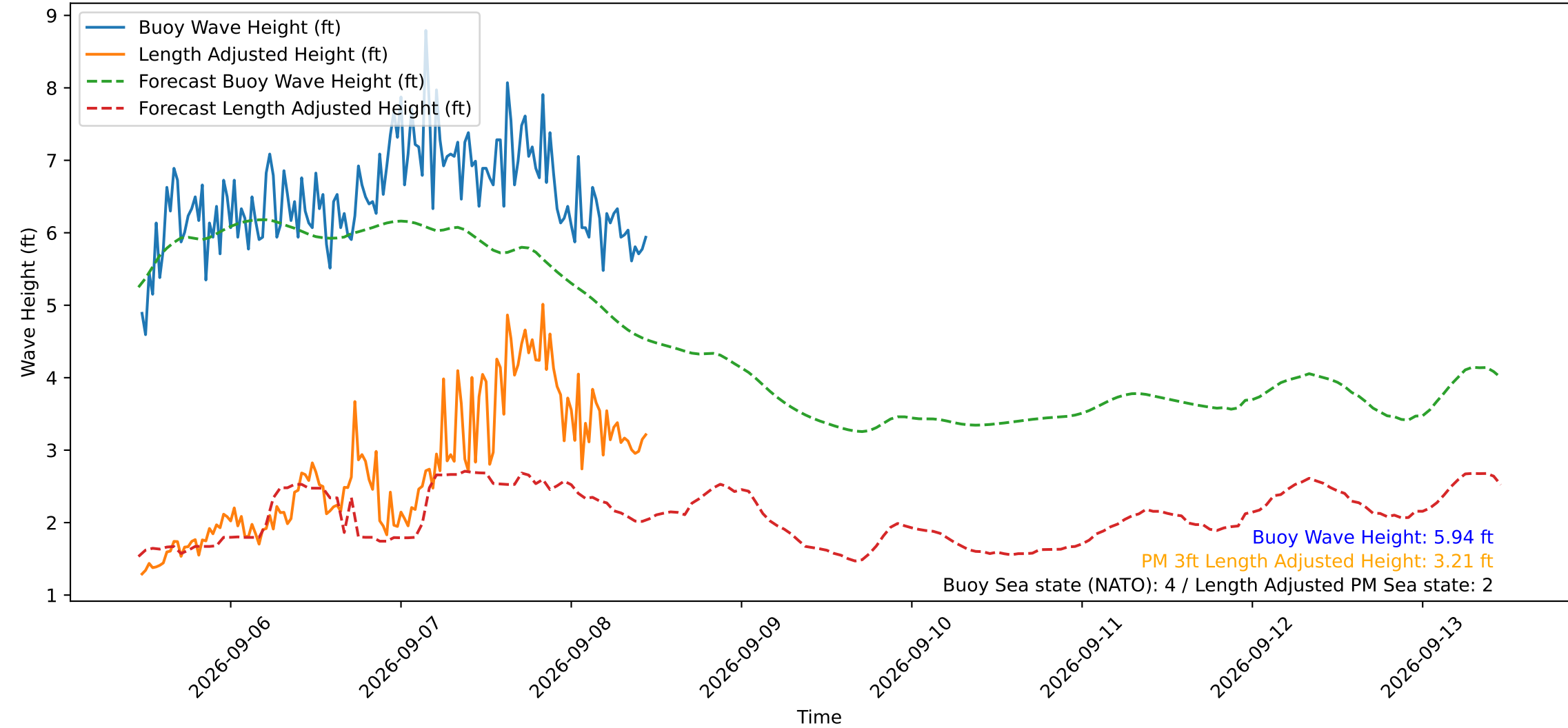
Wave Heights over Time for Green Beach at 2026-09-08 11:21:14
