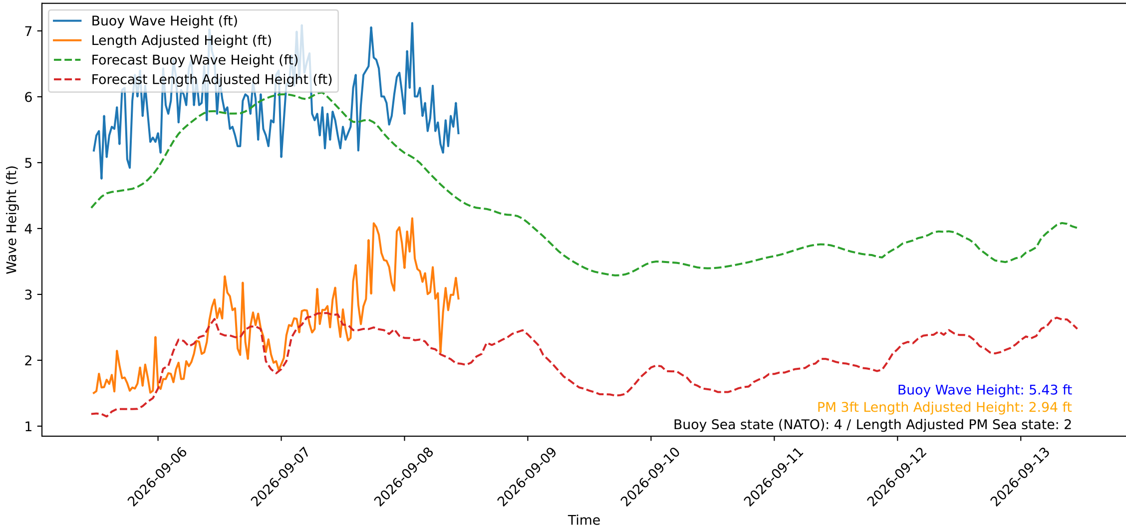
Wave Heights over Time for Oceanside Harbor at 2026-09-08 11:20:30
