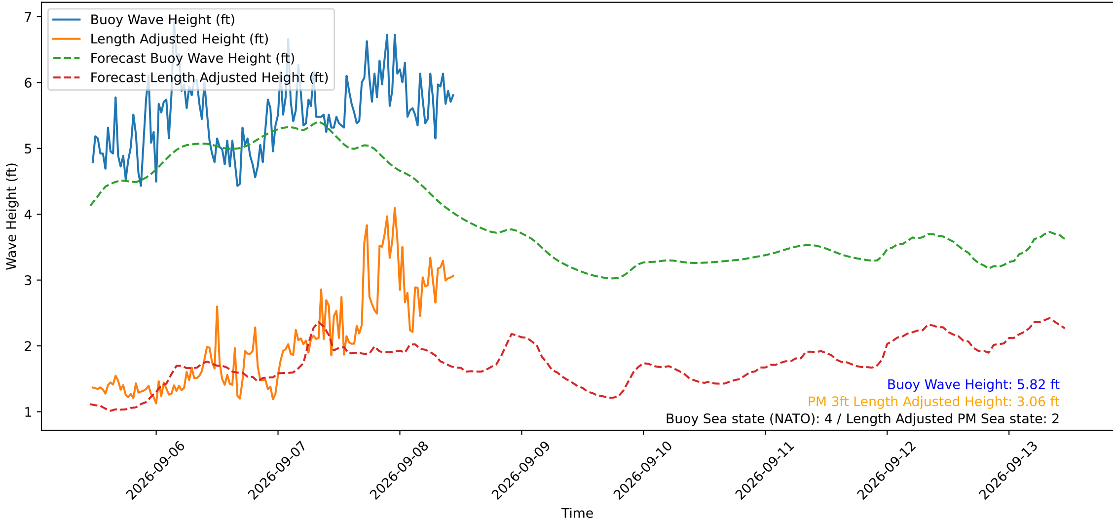
Wave Heights over Time for Red Beach at 2026-09-08 11:20:51
