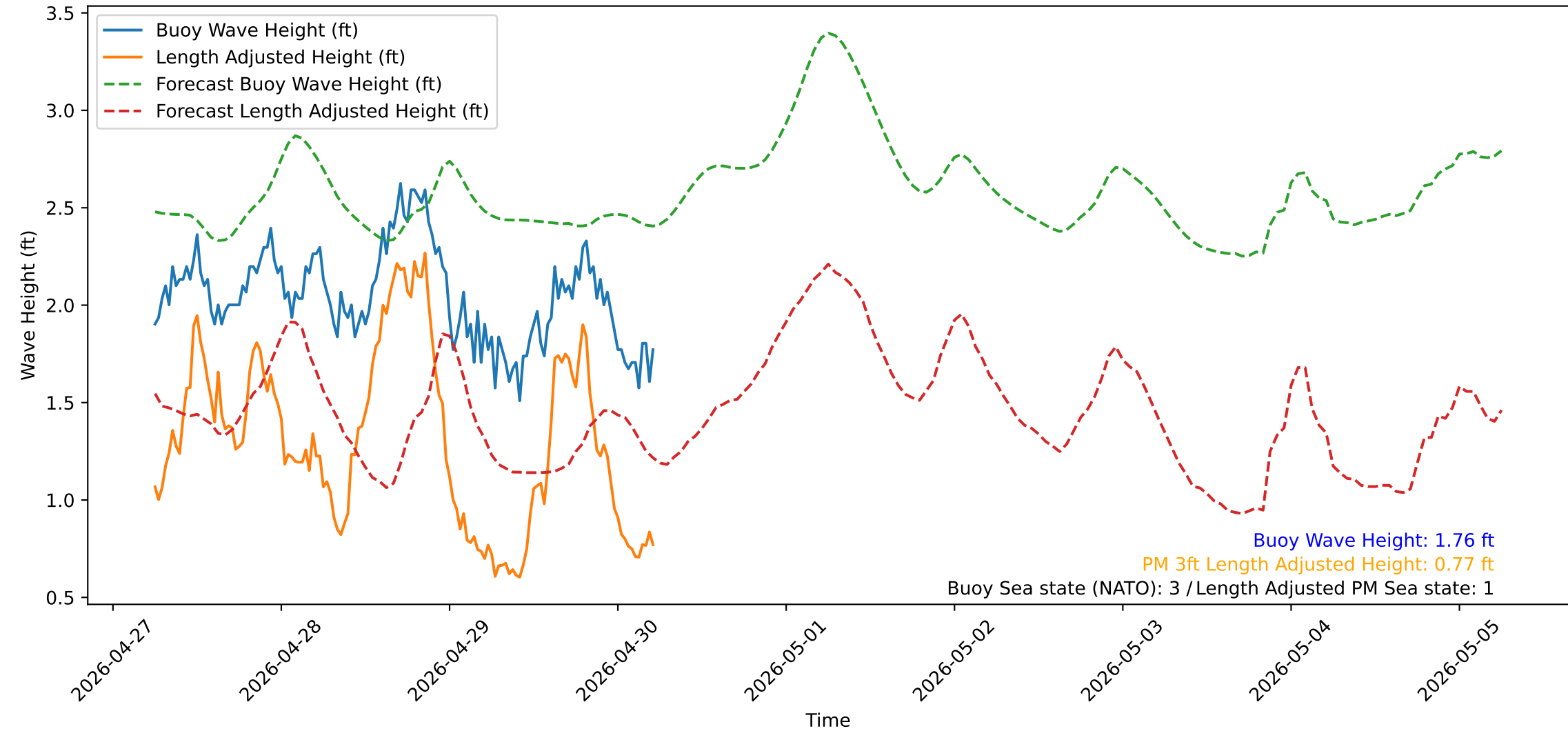
Wave Heights over Time for Red Beach at 2026-04-30 05:50:51
