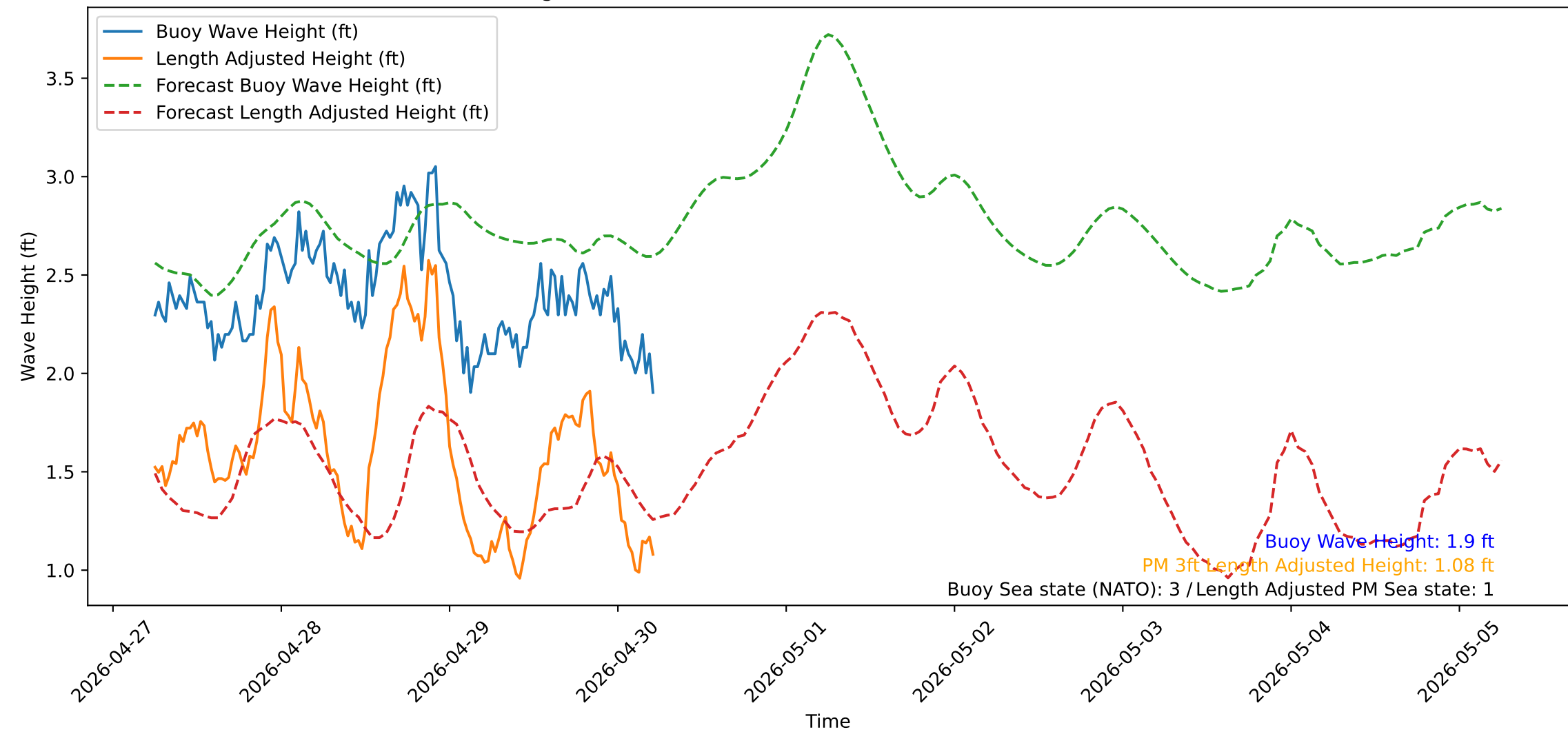
Wave Heights over Time for Oceanside Harbor at 2026-04-30 05:50:30
