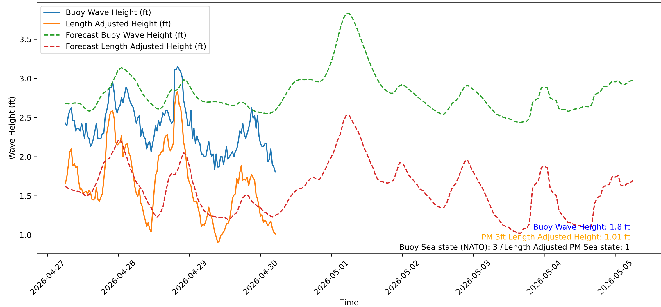
Wave Heights over Time for Green Beach at 2026-04-30 05:51:14
