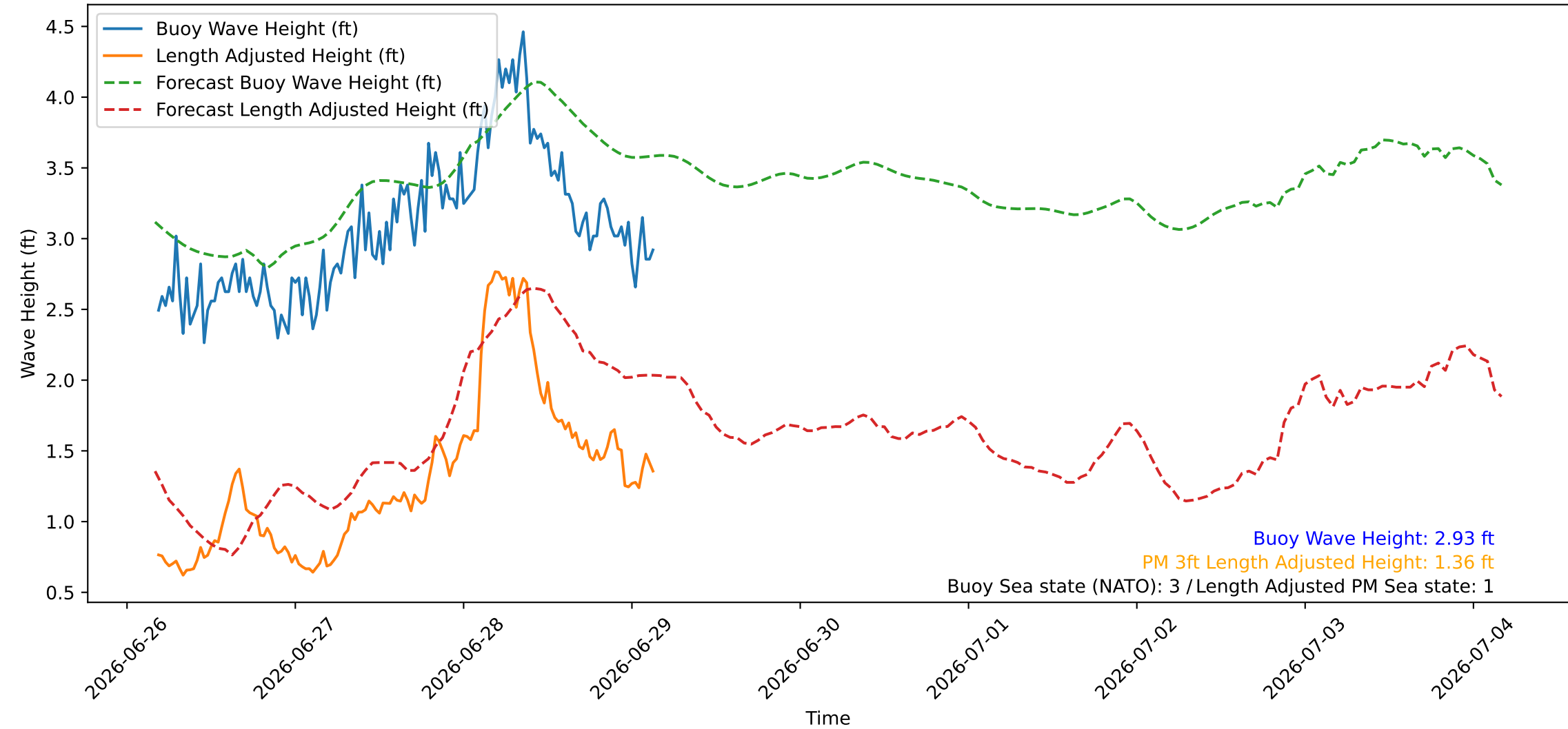
Wave Heights over Time for Red Beach at 2026-06-29 04:00:45
