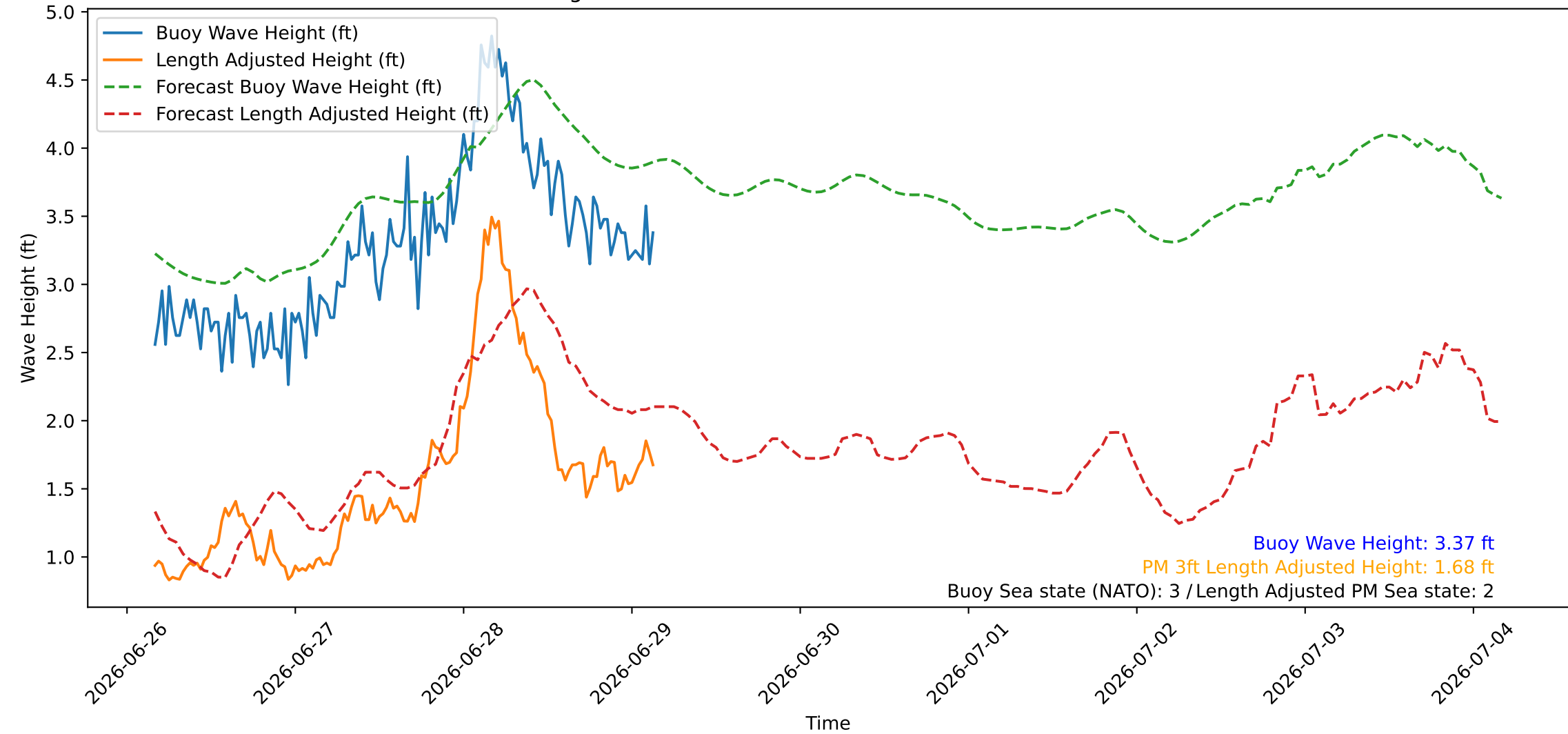
Wave Heights over Time for Green Beach at 2026-06-29 04:01:07
