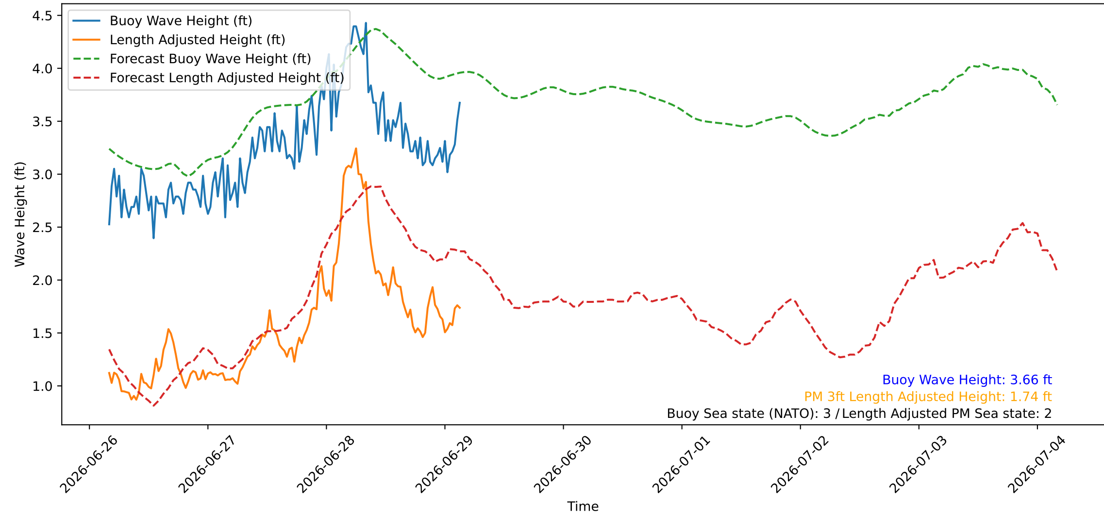
Wave Heights over Time for Oceanside Harbor at 2026-06-29 04:00:26
