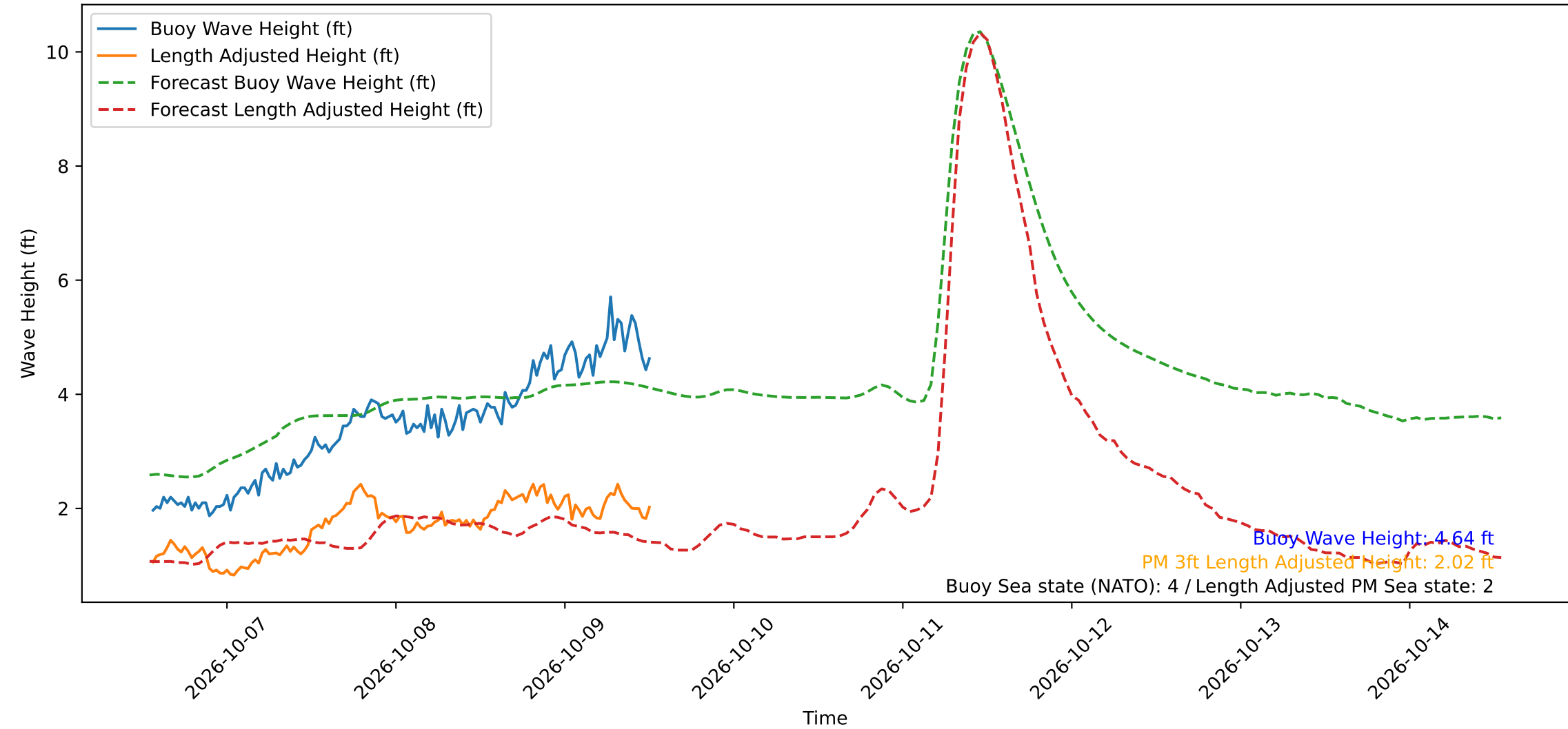
Wave Heights over Time for Red Beach at 2026-10-09 13:00:49
