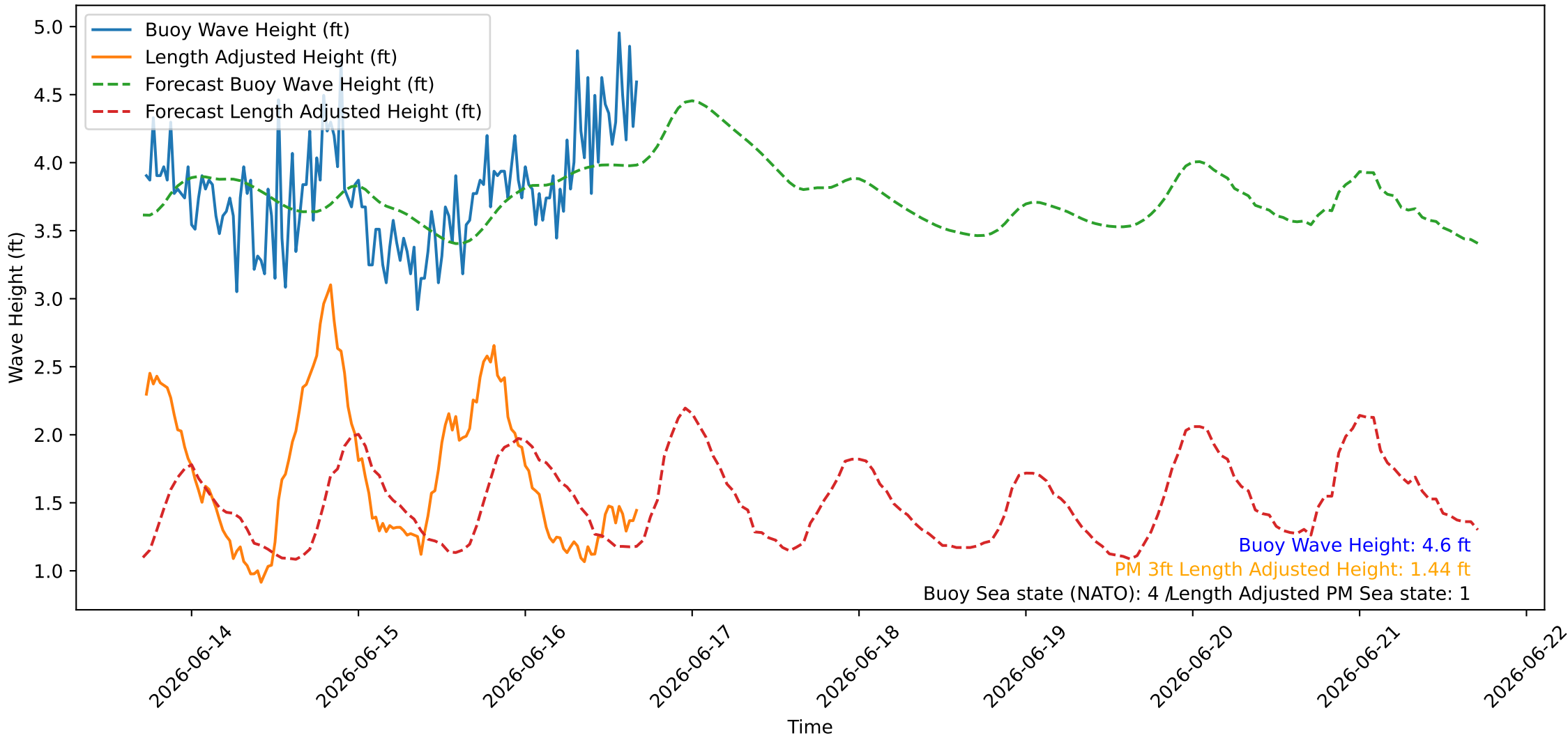
Wave Heights over Time for Red Beach at 2026-06-16 17:00:45
