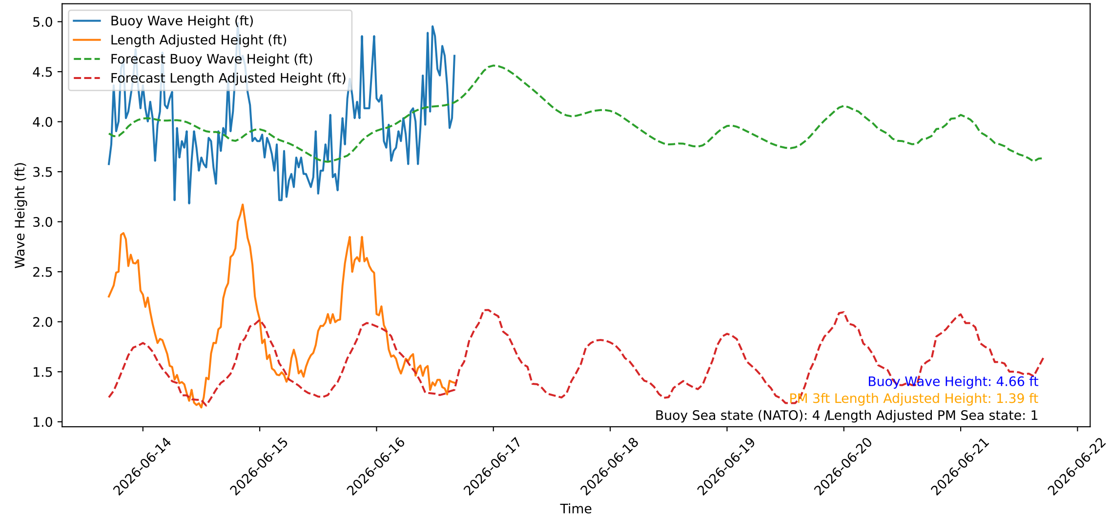
Wave Heights over Time for Oceanside Harbor at 2026-06-16 17:00:26
