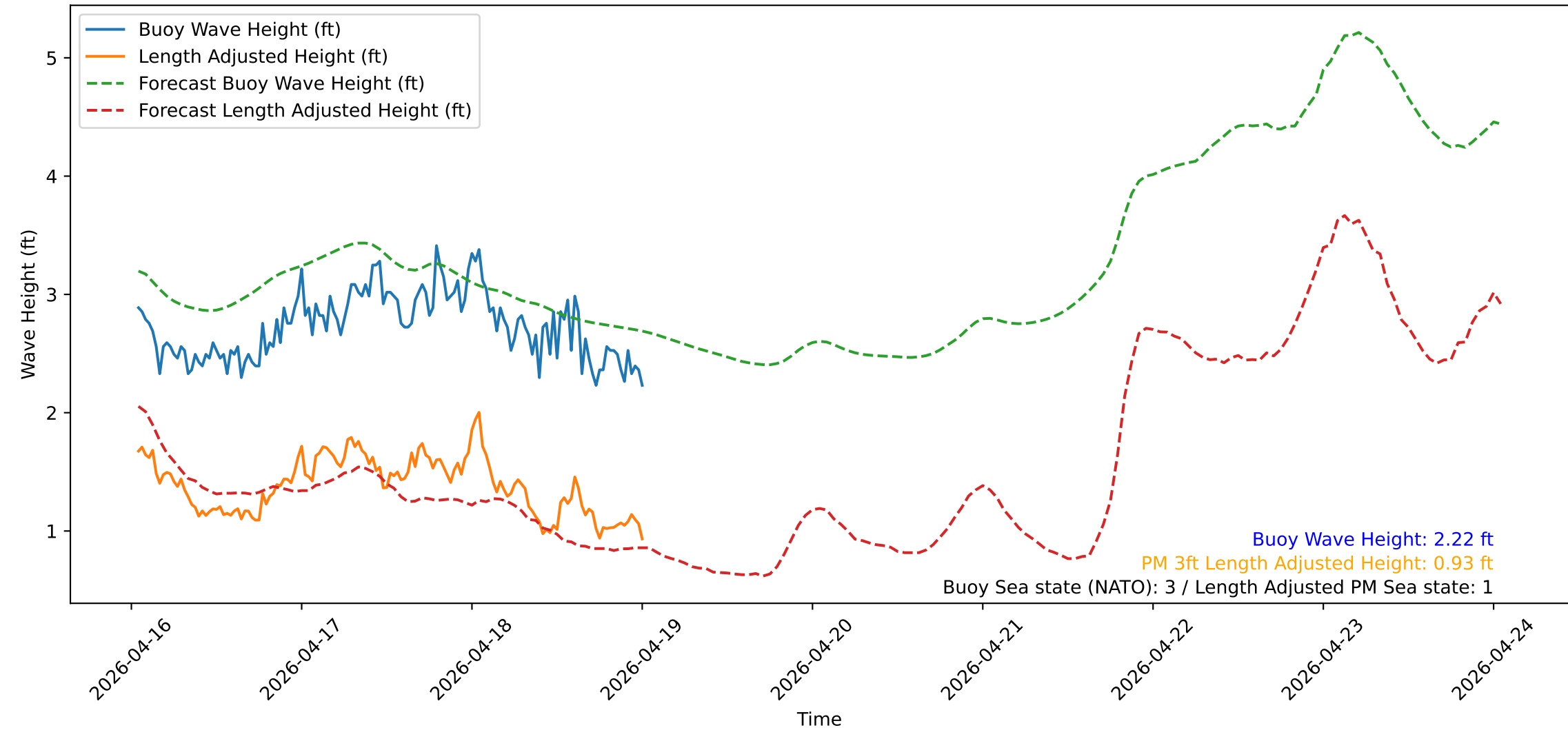
Wave Heights over Time for Oceanside Harbor at 2026-04-19 00:50:30
