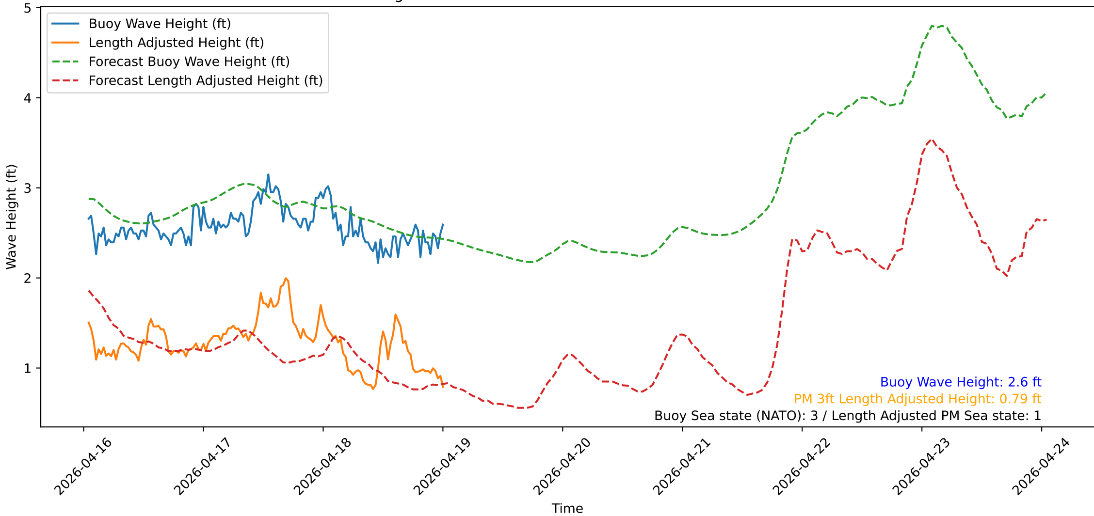
Wave Heights over Time for Red Beach at 2026-04-19 00:50:50
