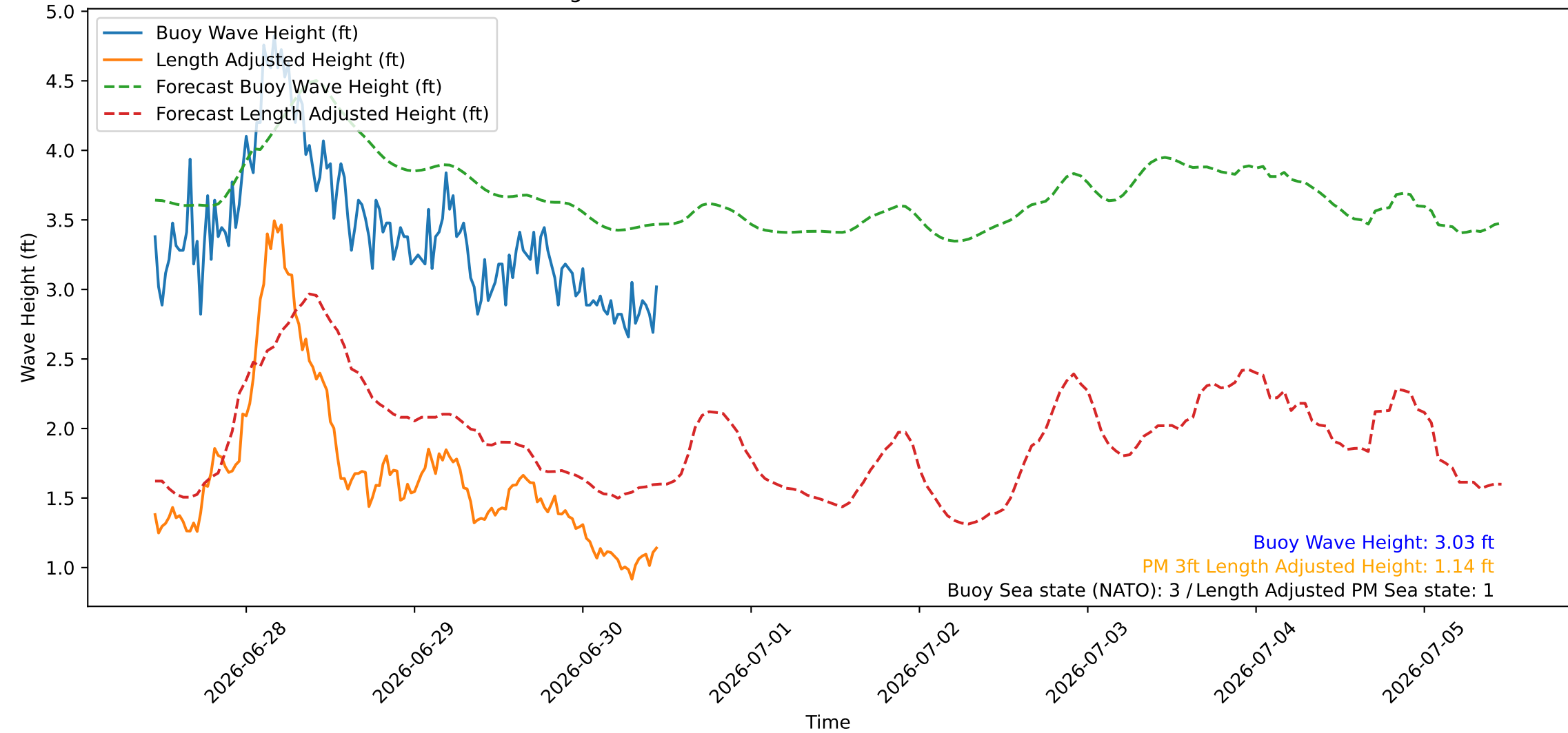
Wave Heights over Time for Green Beach at 2026-06-30 11:11:08
