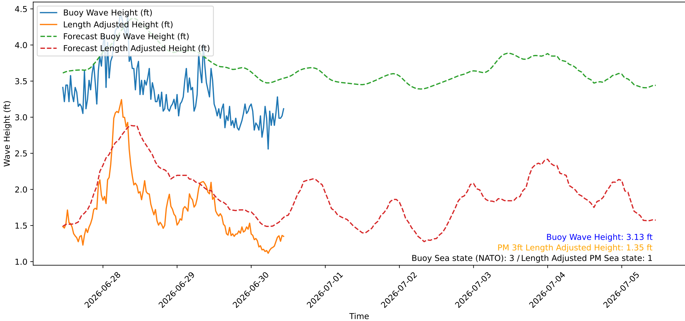
Wave Heights over Time for Oceanside Harbor at 2026-06-30 11:10:26
