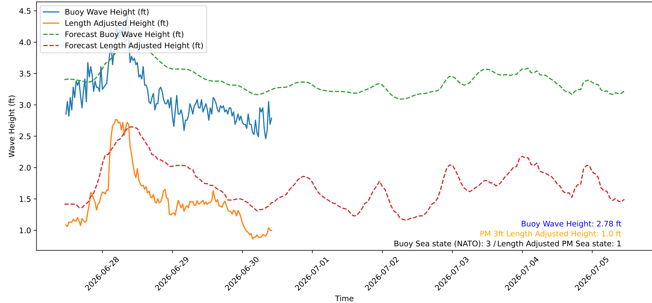
Wave Heights over Time for Red Beach at 2026-06-30 11:10:45
