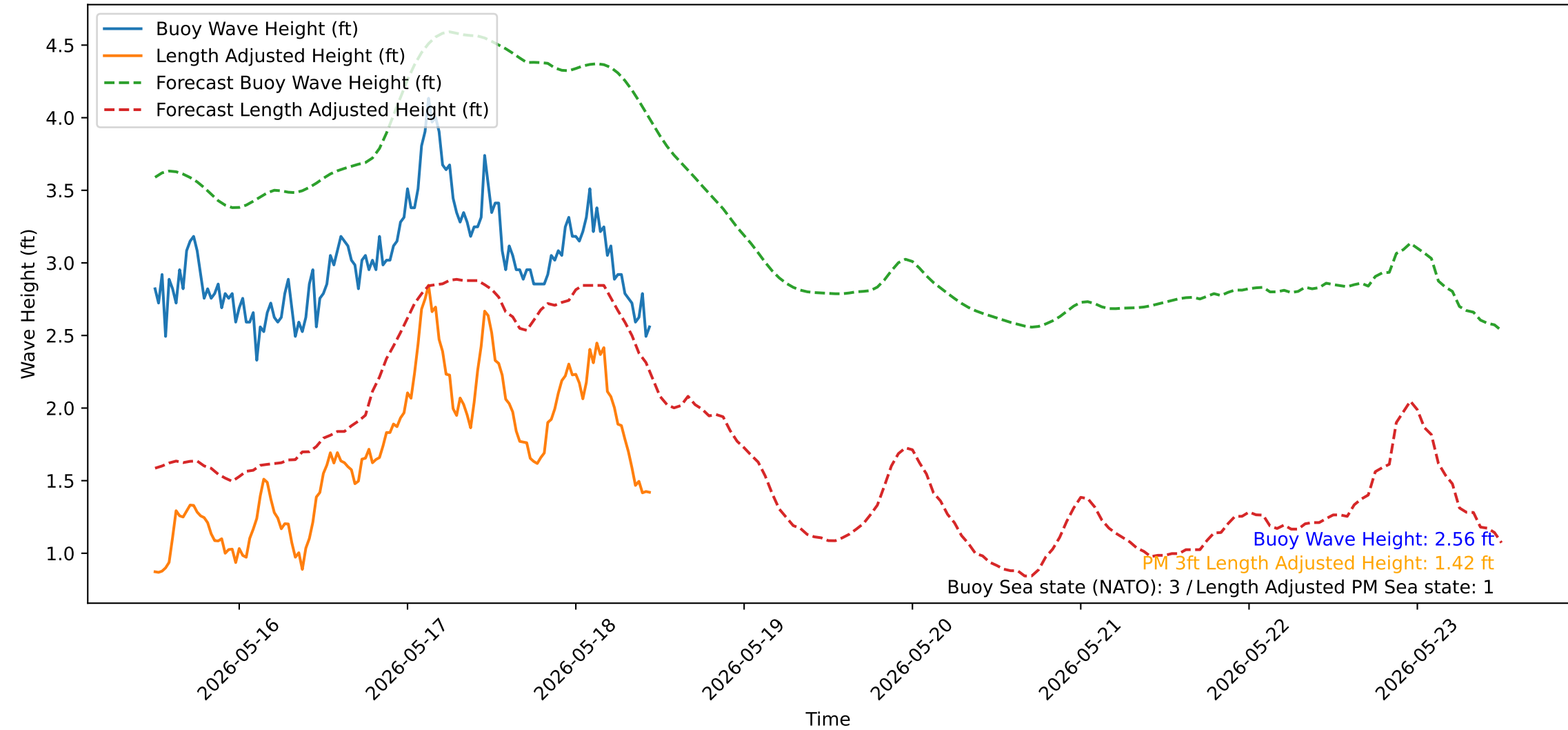
Wave Heights over Time for Red Beach at 2026-05-18 11:30:51
