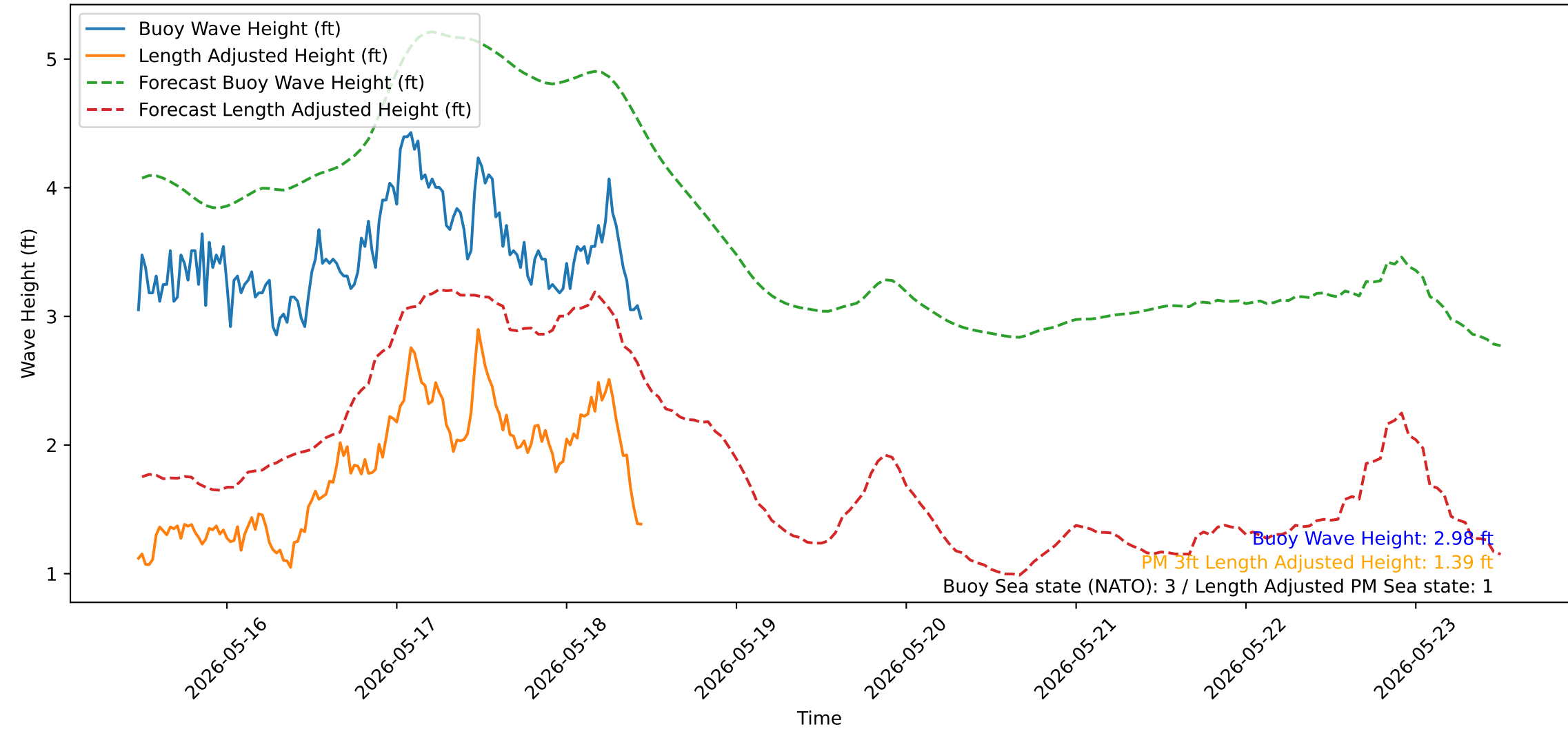
Wave Heights over Time for Green Beach at 2026-05-18 11:31:14
