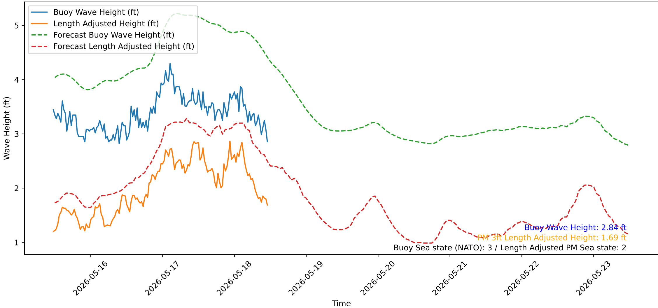
Wave Heights over Time for Oceanside Harbor at 2026-05-18 11:30:32
