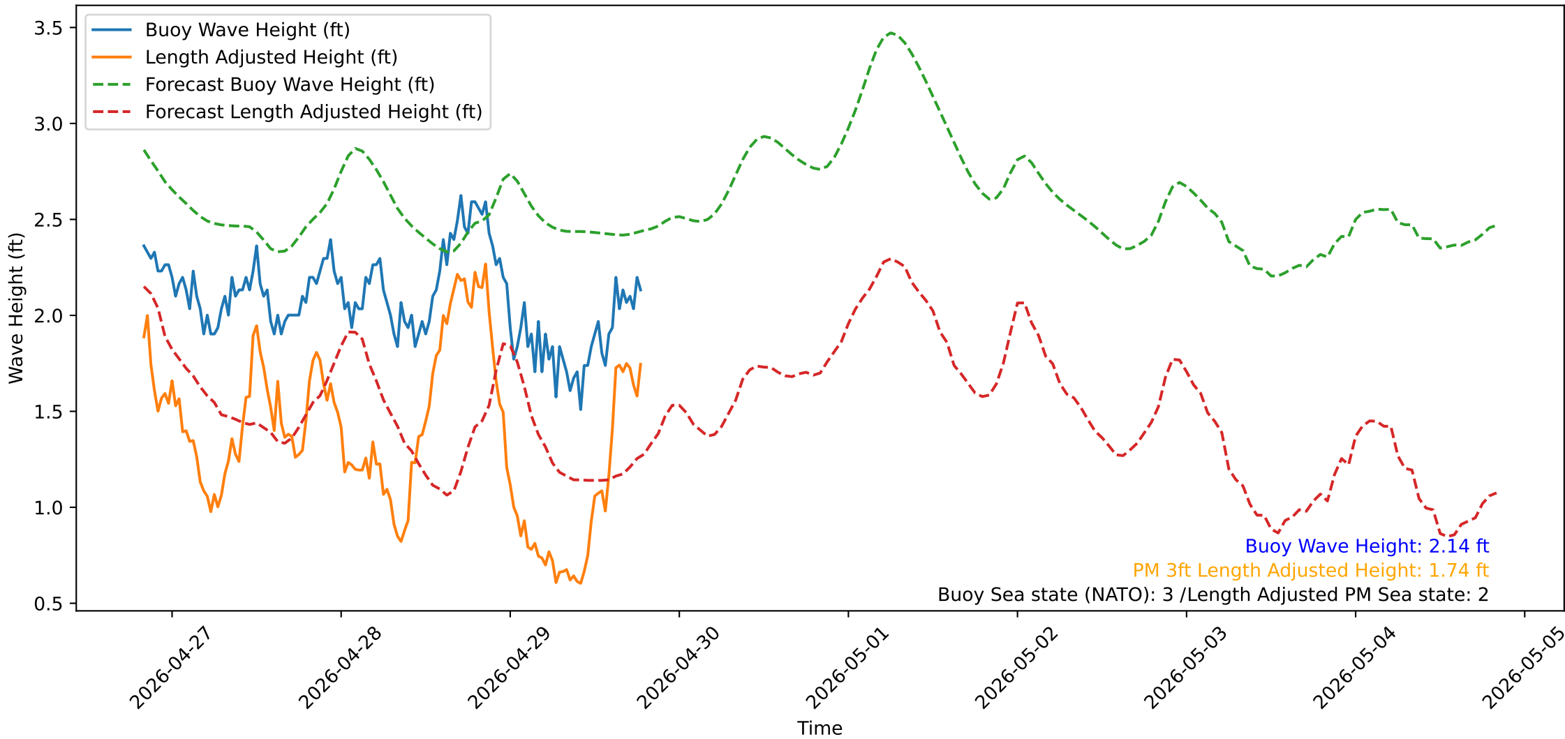
Wave Heights over Time for Red Beach at 2026-04-29 19:30:51
