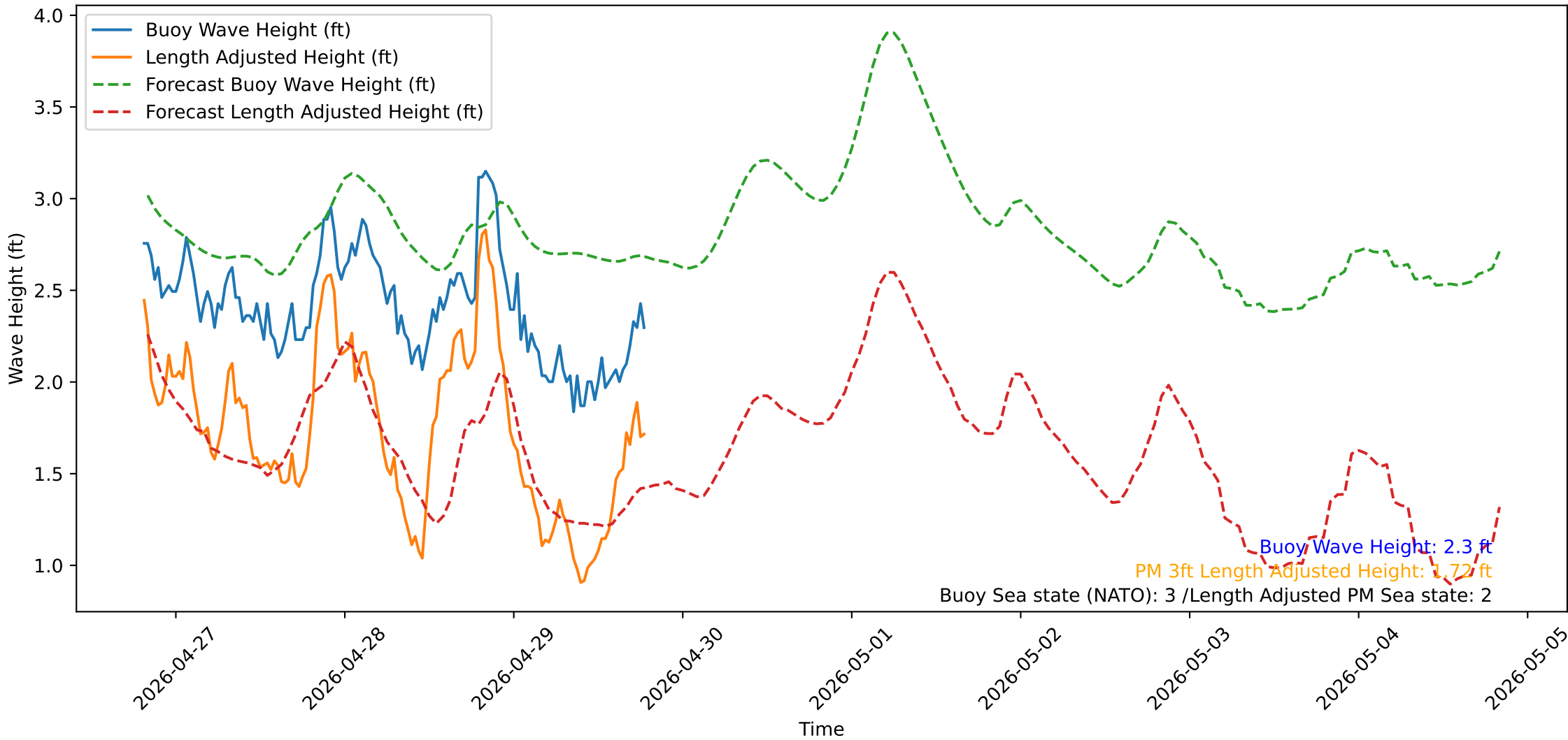
Wave Heights over Time for Green Beach at 2026-04-29 19:31:14
