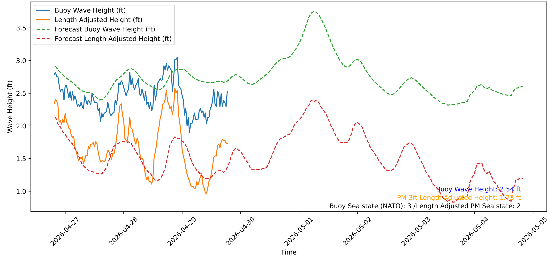
Wave Heights over Time for Oceanside Harbor at 2026-04-29 19:30:32
