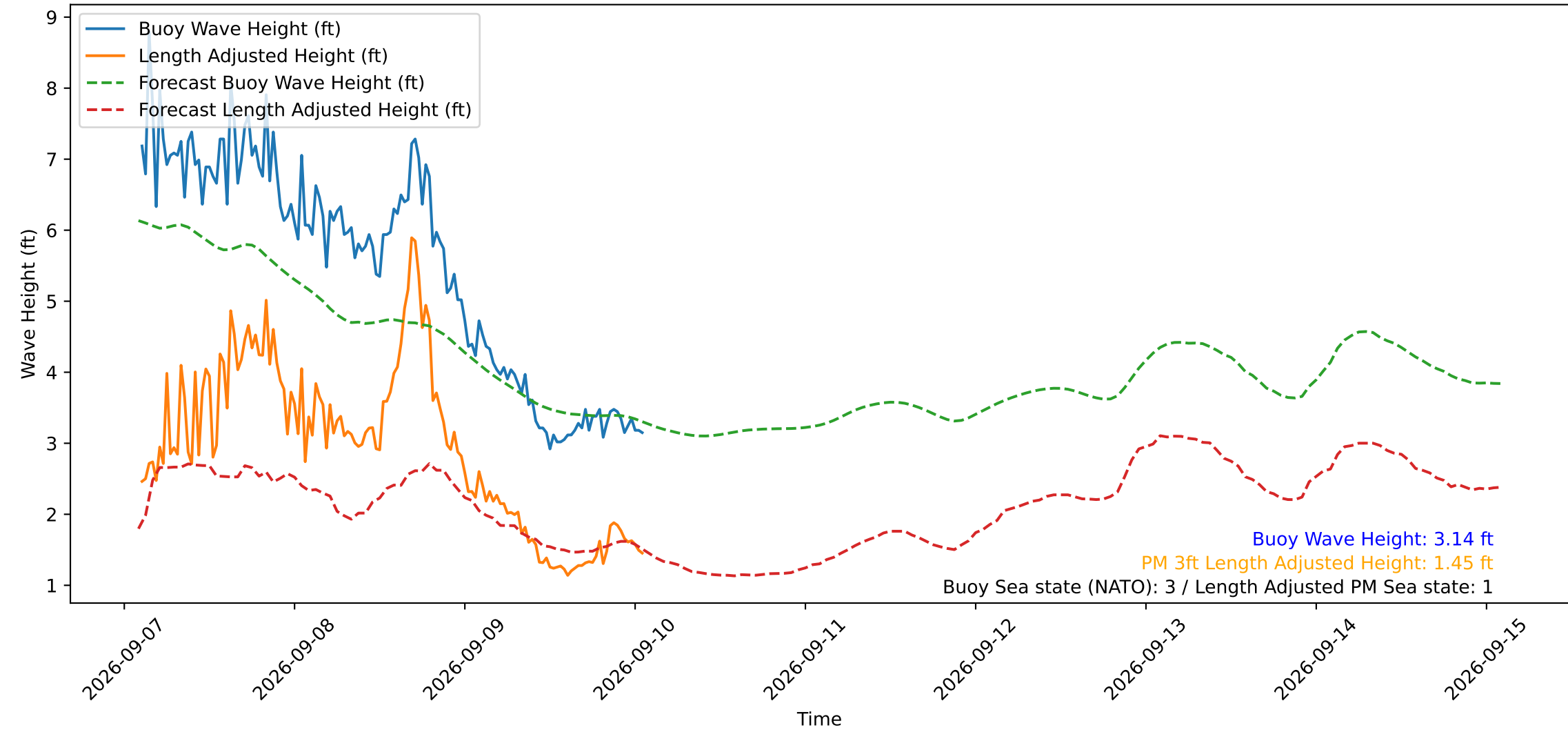
Wave Heights over Time for Green Beach at 2026-09-10 02:01:10
