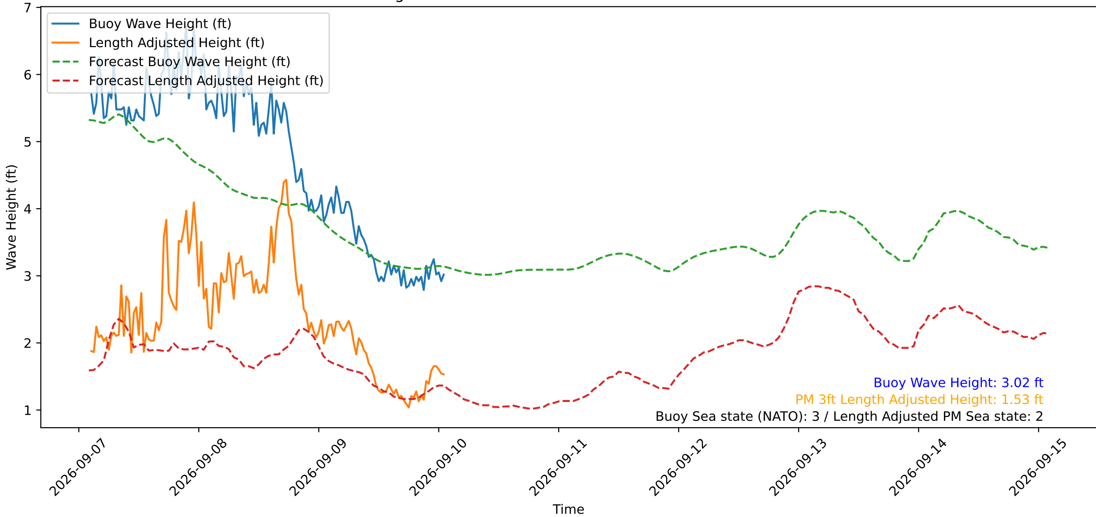
Wave Heights over Time for Red Beach at 2026-09-10 02:00:48
