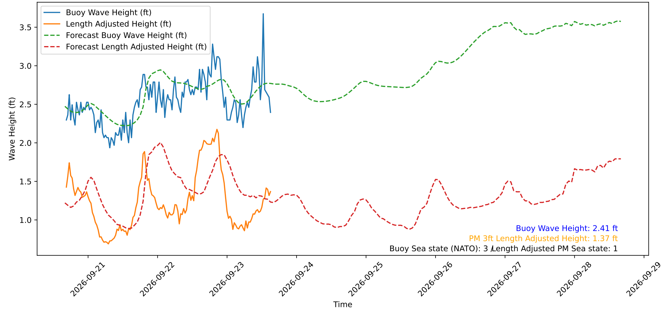
Wave Heights over Time for Red Beach at 2026-09-23 16:00:50
