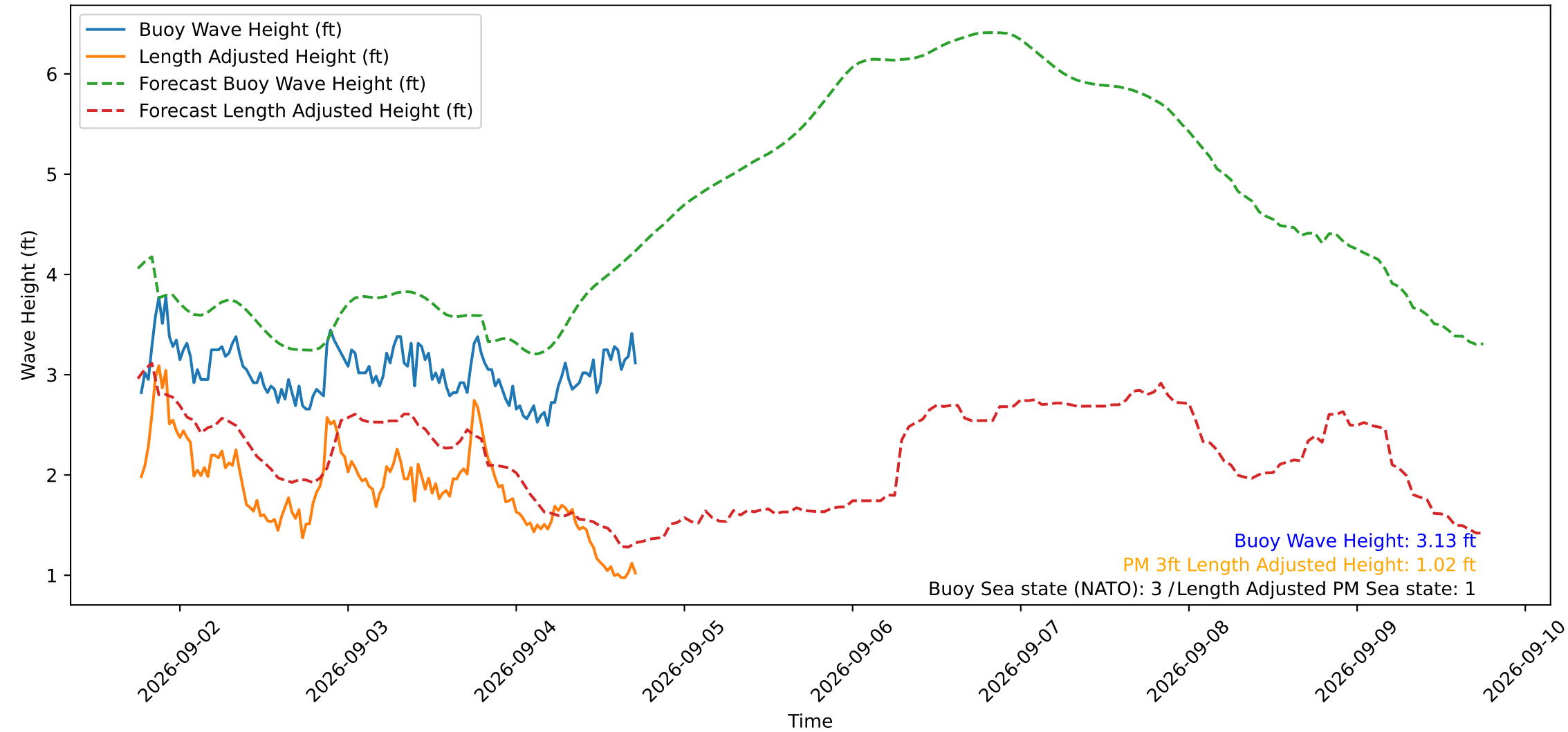
Wave Heights over Time for Green Beach at 2026-09-04 18:01:13
