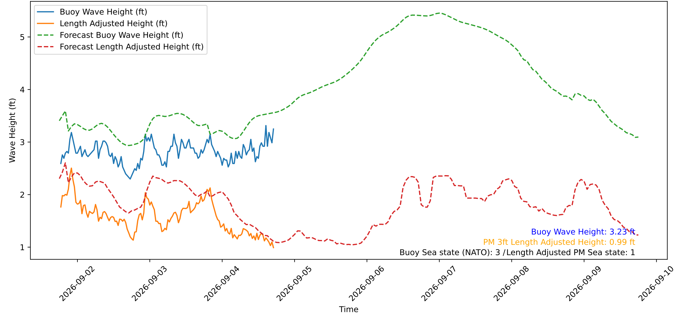
Wave Heights over Time for Red Beach at 2026-09-04 18:00:50
