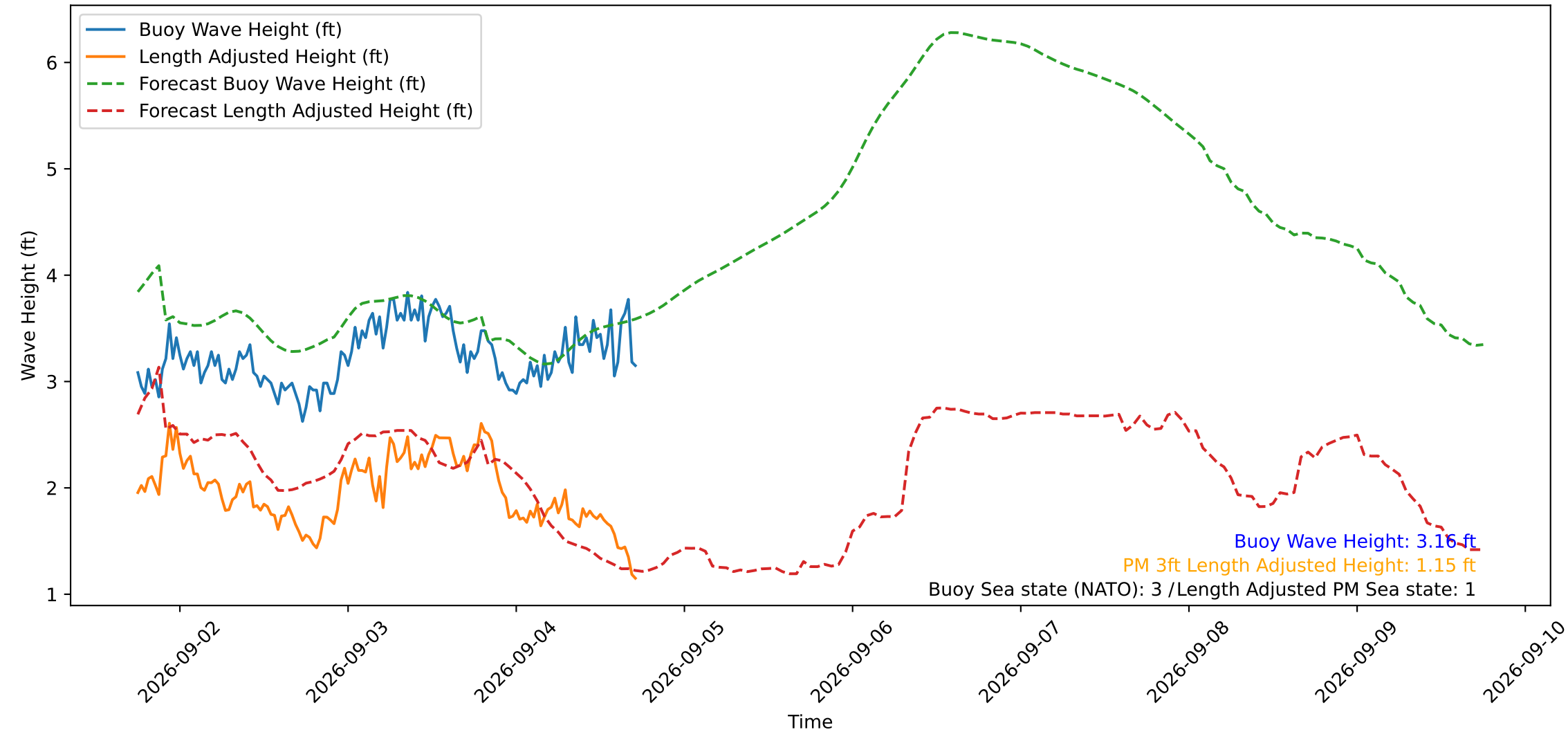
Wave Heights over Time for Oceanside Harbor at 2026-09-04 18:00:30
