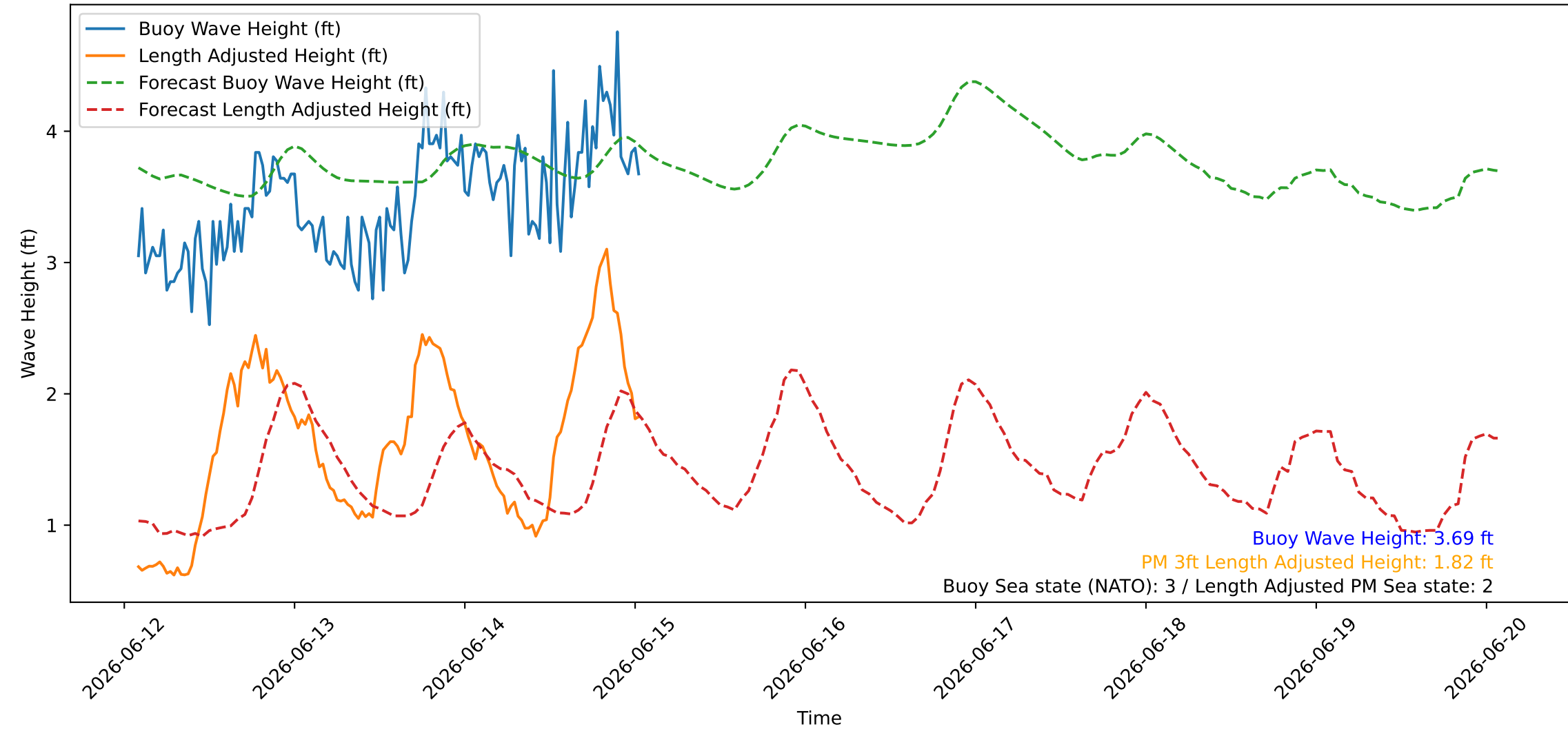
Wave Heights over Time for Red Beach at 2026-06-15 01:30:45
