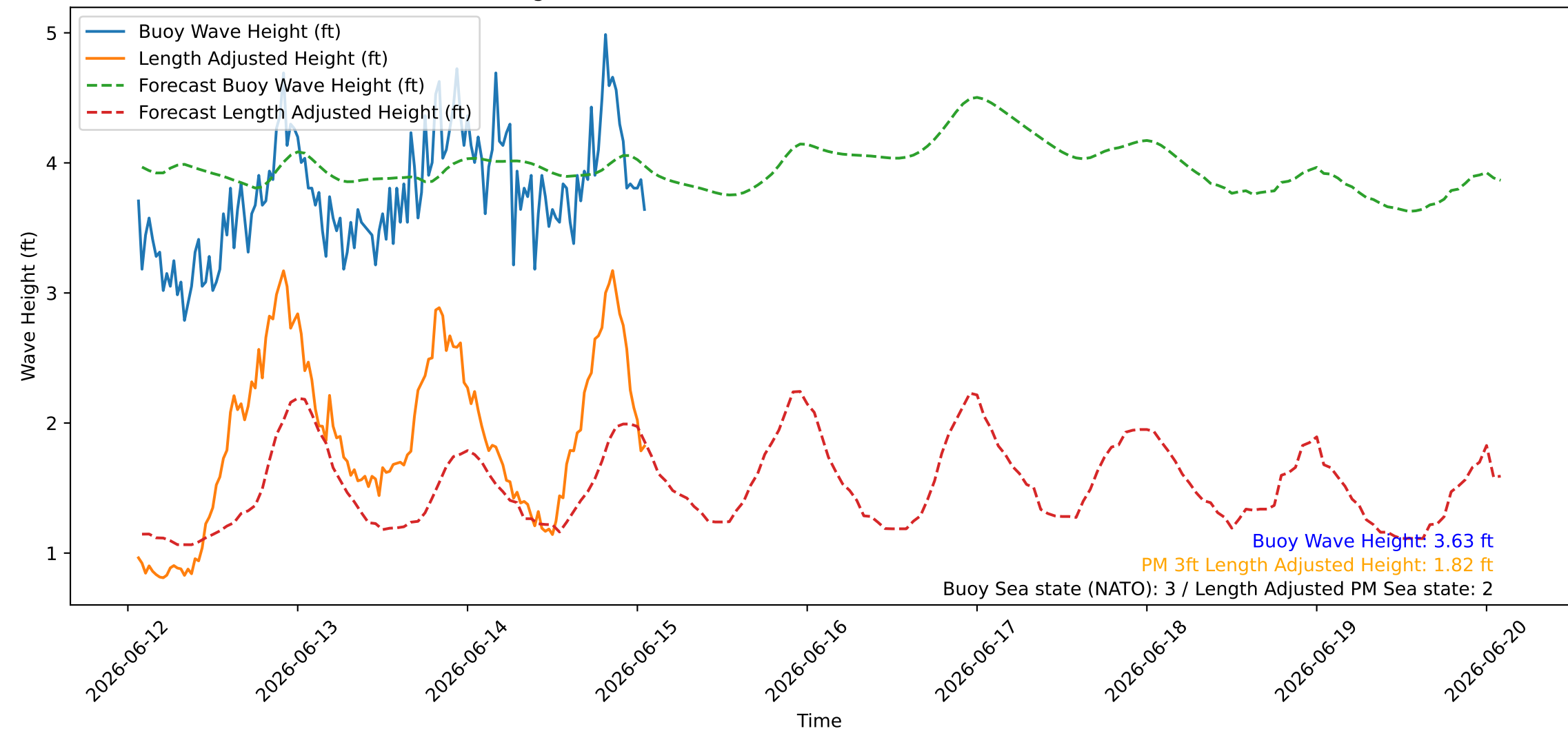
Wave Heights over Time for Oceanside Harbor at 2026-06-15 01:30:26
