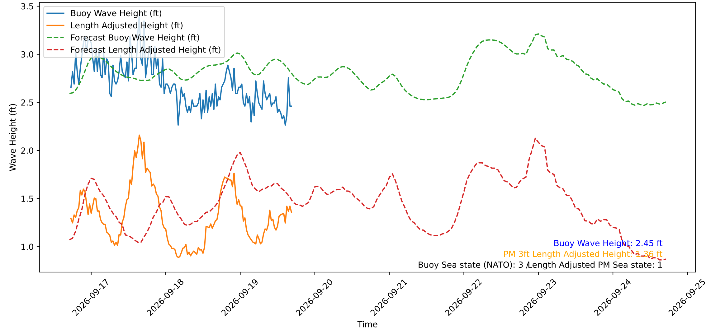
Wave Heights over Time for Red Beach at 2026-09-19 17:20:50
