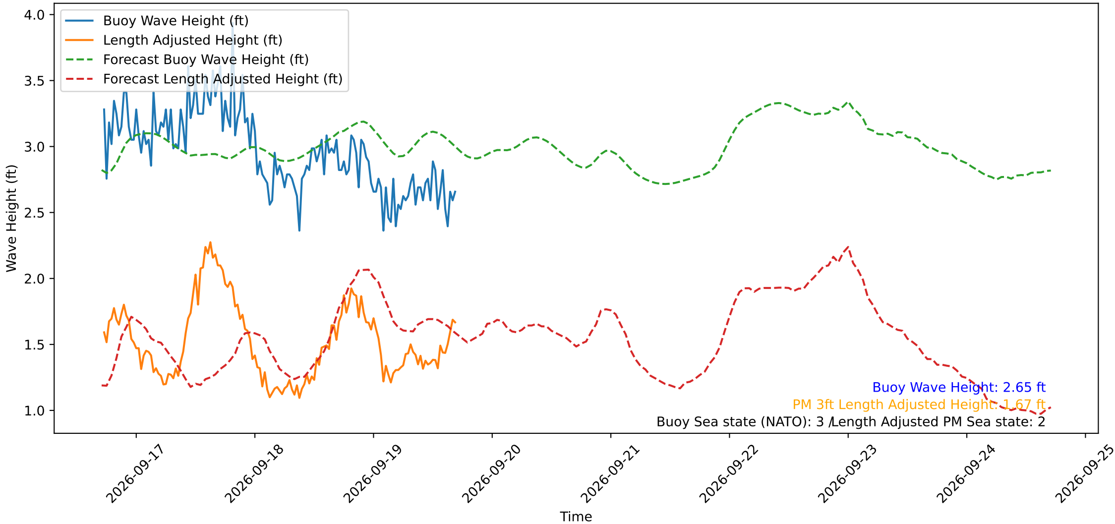
Wave Heights over Time for Oceanside Harbor at 2026-09-19 17:20:29
