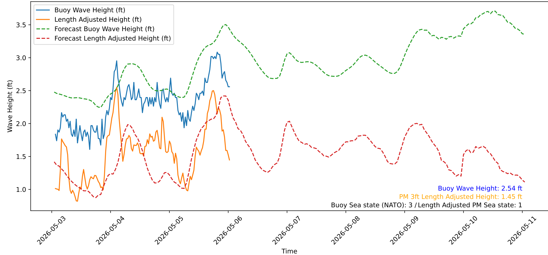
Wave Heights over Time for Red Beach at 2026-05-06 01:20:51
