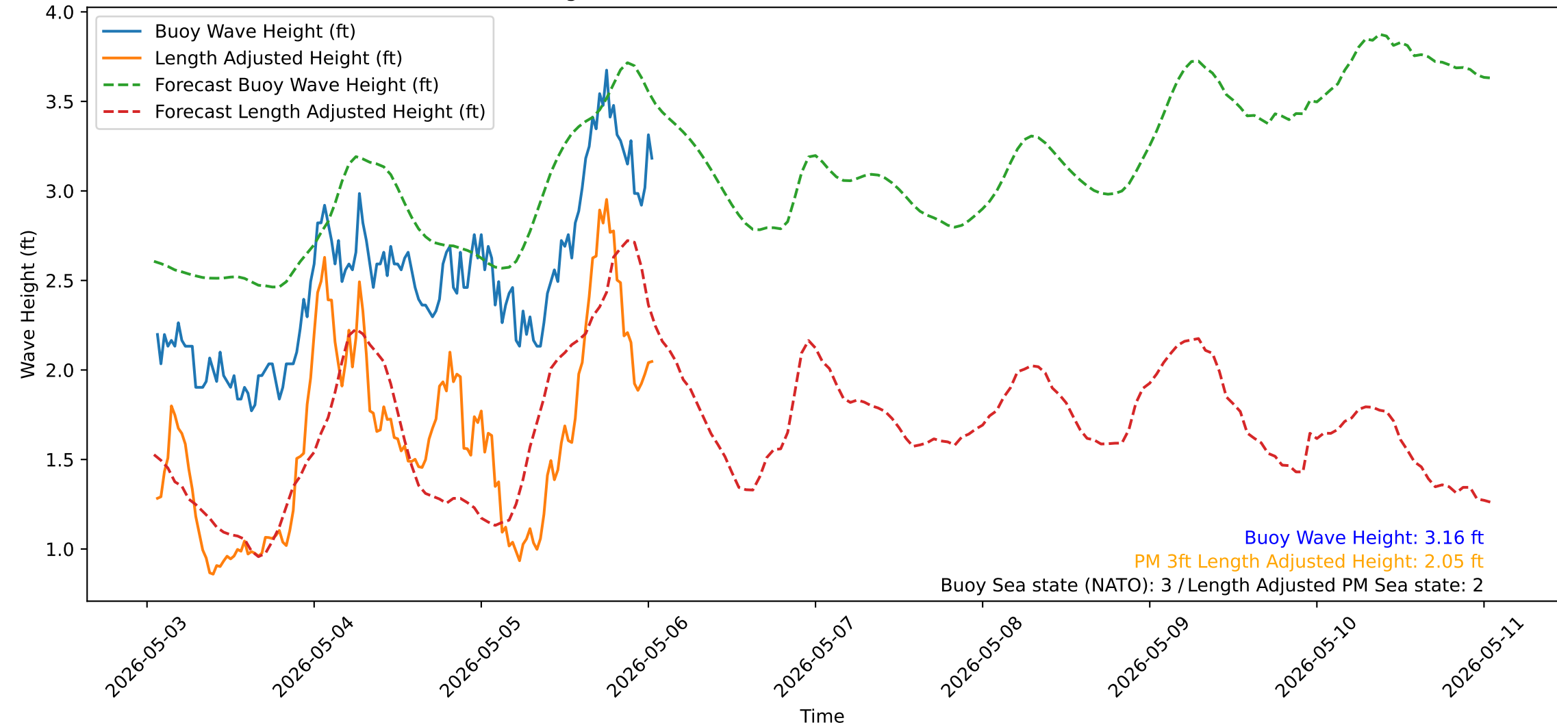
Wave Heights over Time for Green Beach at 2026-05-06 01:21:13
