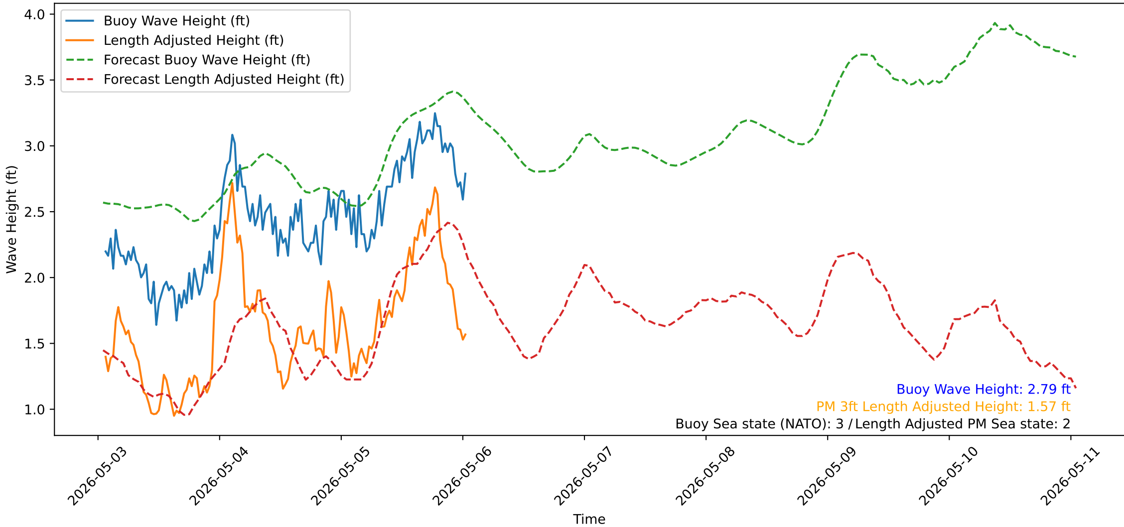
Wave Heights over Time for Oceanside Harbor at 2026-05-06 01:20:31
