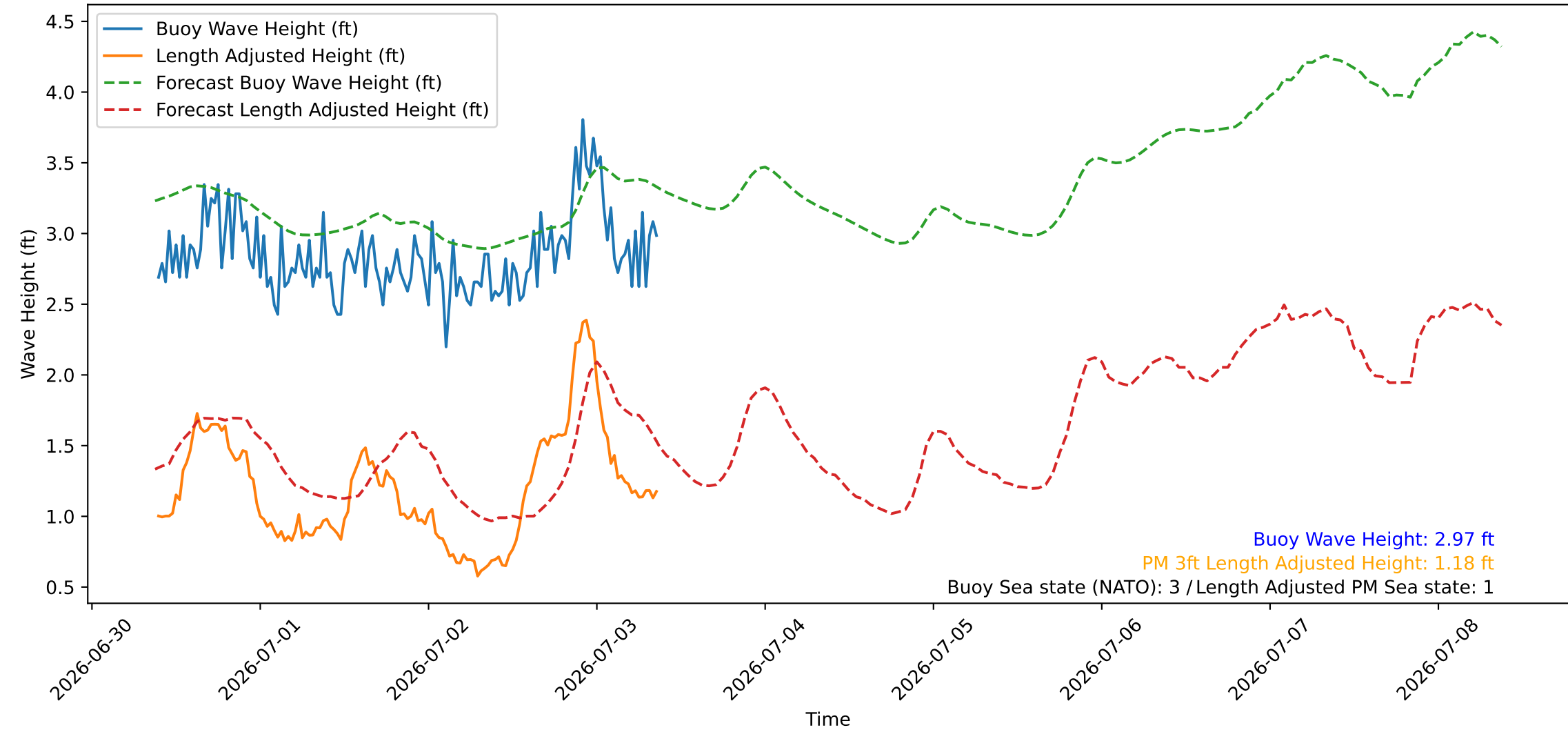
Wave Heights over Time for Red Beach at 2026-07-03 09:10:45
