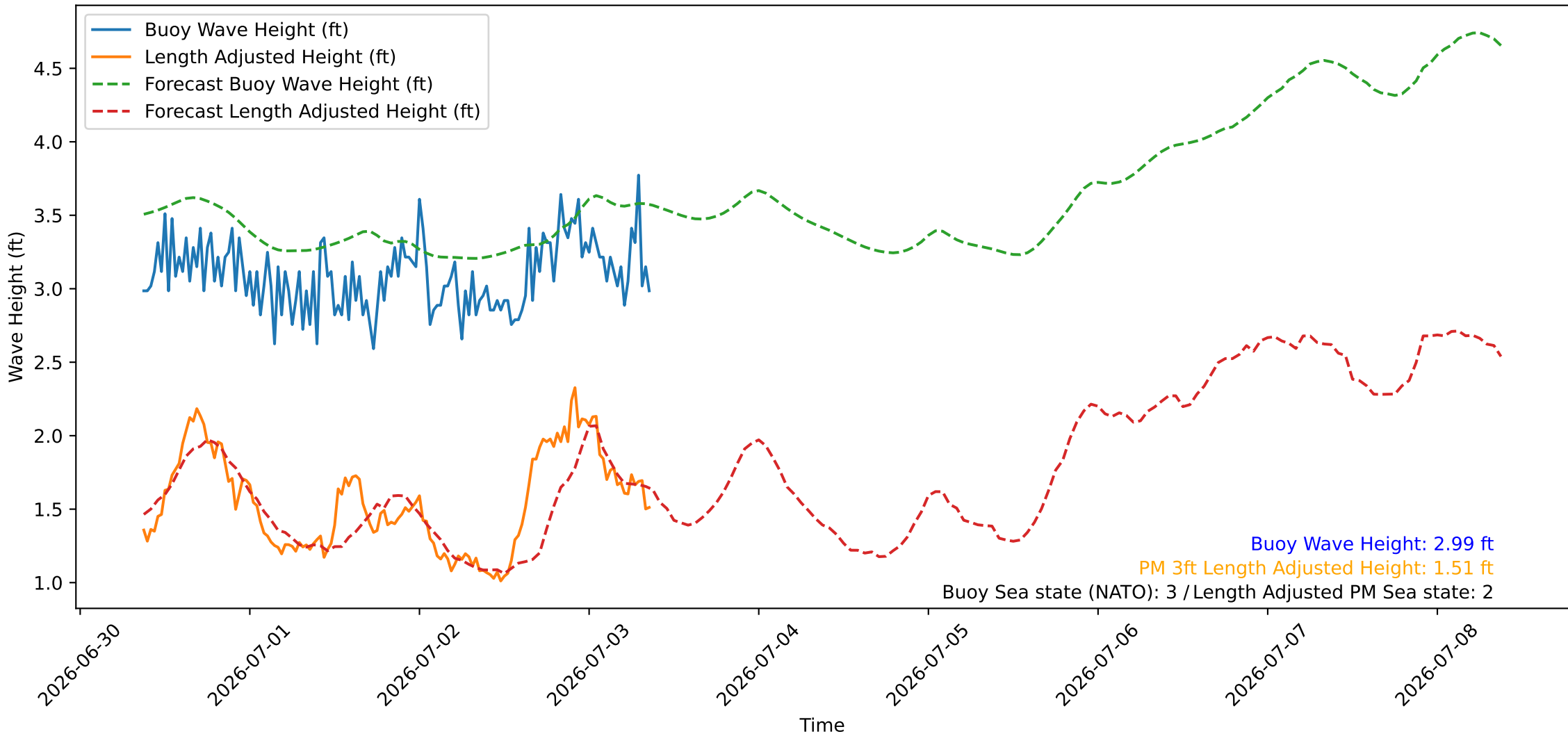
Wave Heights over Time for Oceanside Harbor at 2026-07-03 09:10:26
