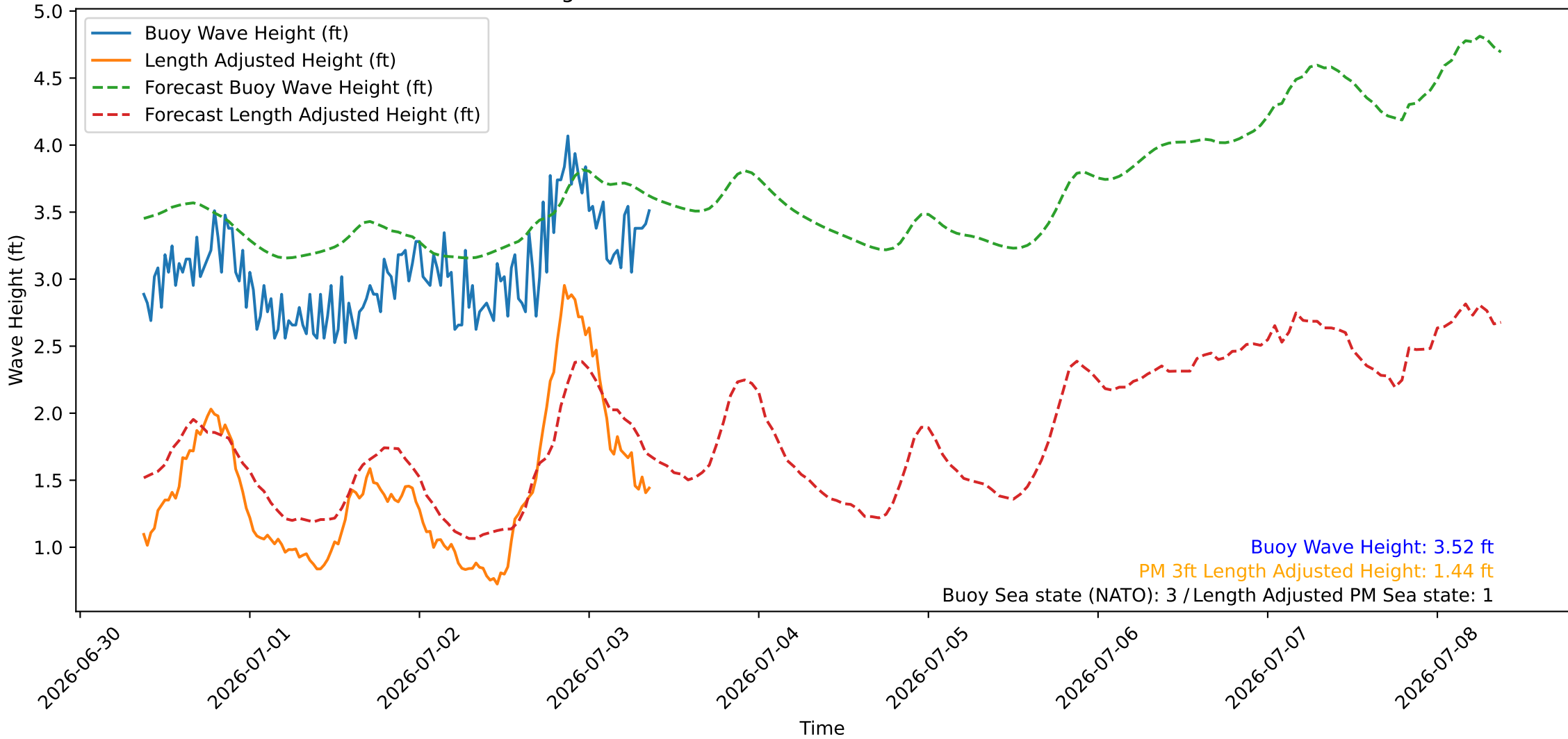
Wave Heights over Time for Green Beach at 2026-07-03 09:11:07
