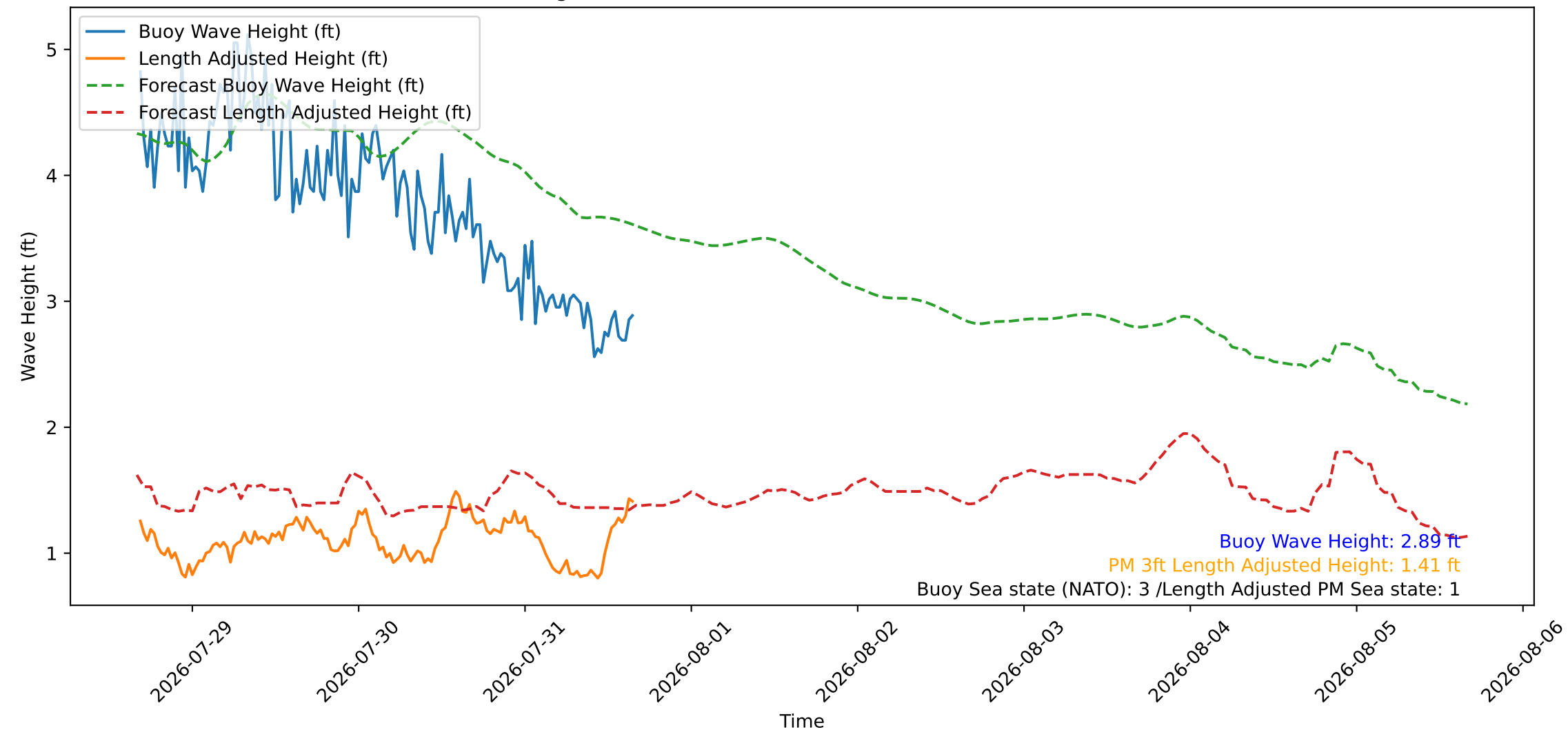
Wave Heights over Time for Red Beach at 2026-07-31 16:10:46
