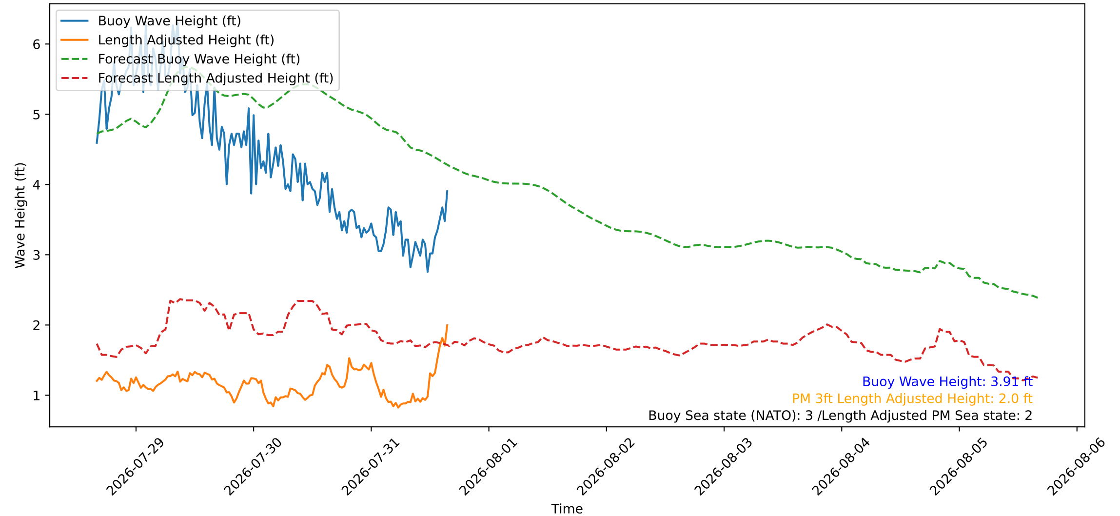
Wave Heights over Time for Green Beach at 2026-07-31 16:11:09
