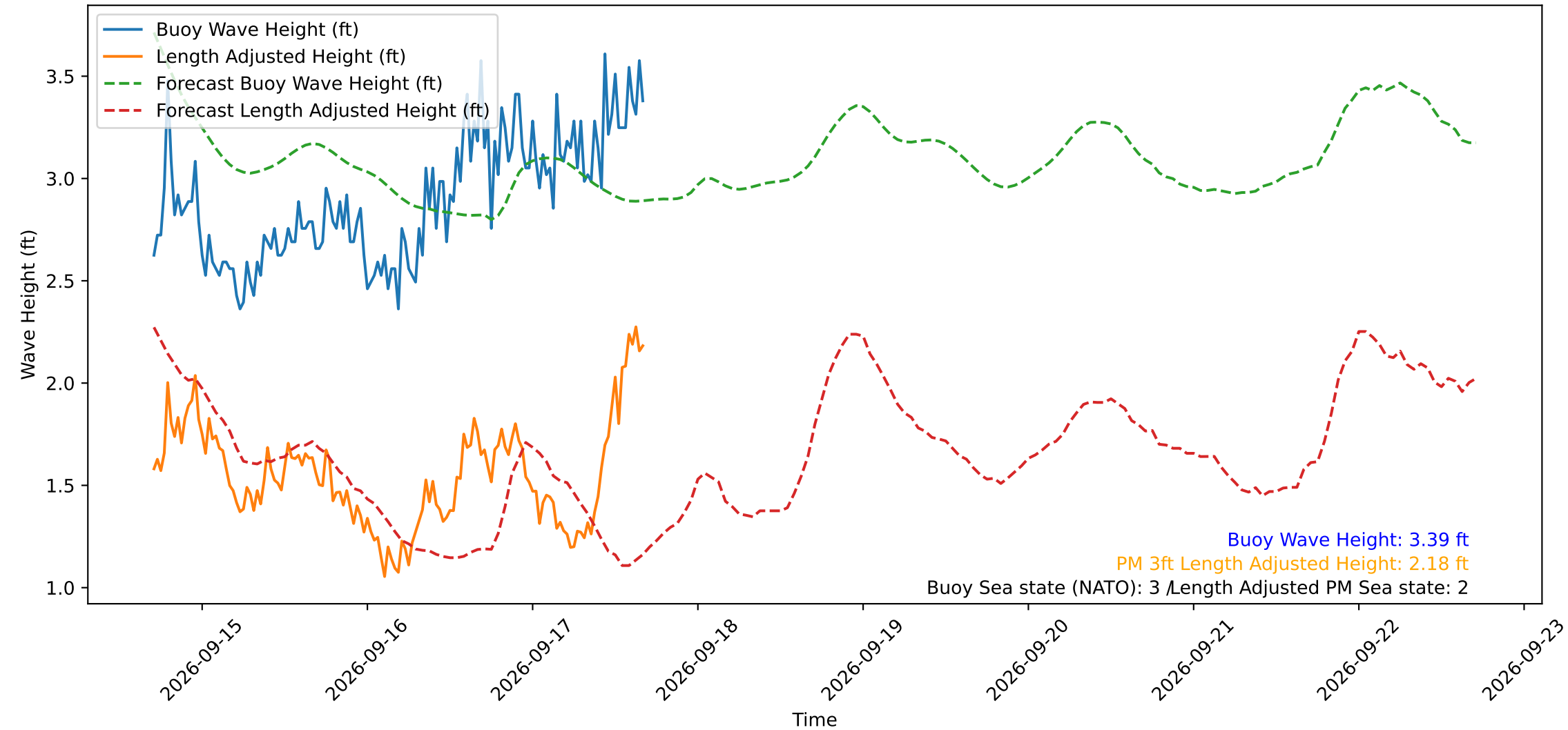
Wave Heights over Time for Oceanside Harbor at 2026-09-17 17:00:30
