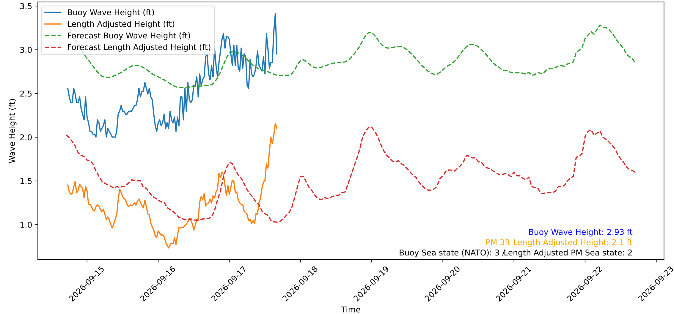
Wave Heights over Time for Red Beach at 2026-09-17 17:00:49
