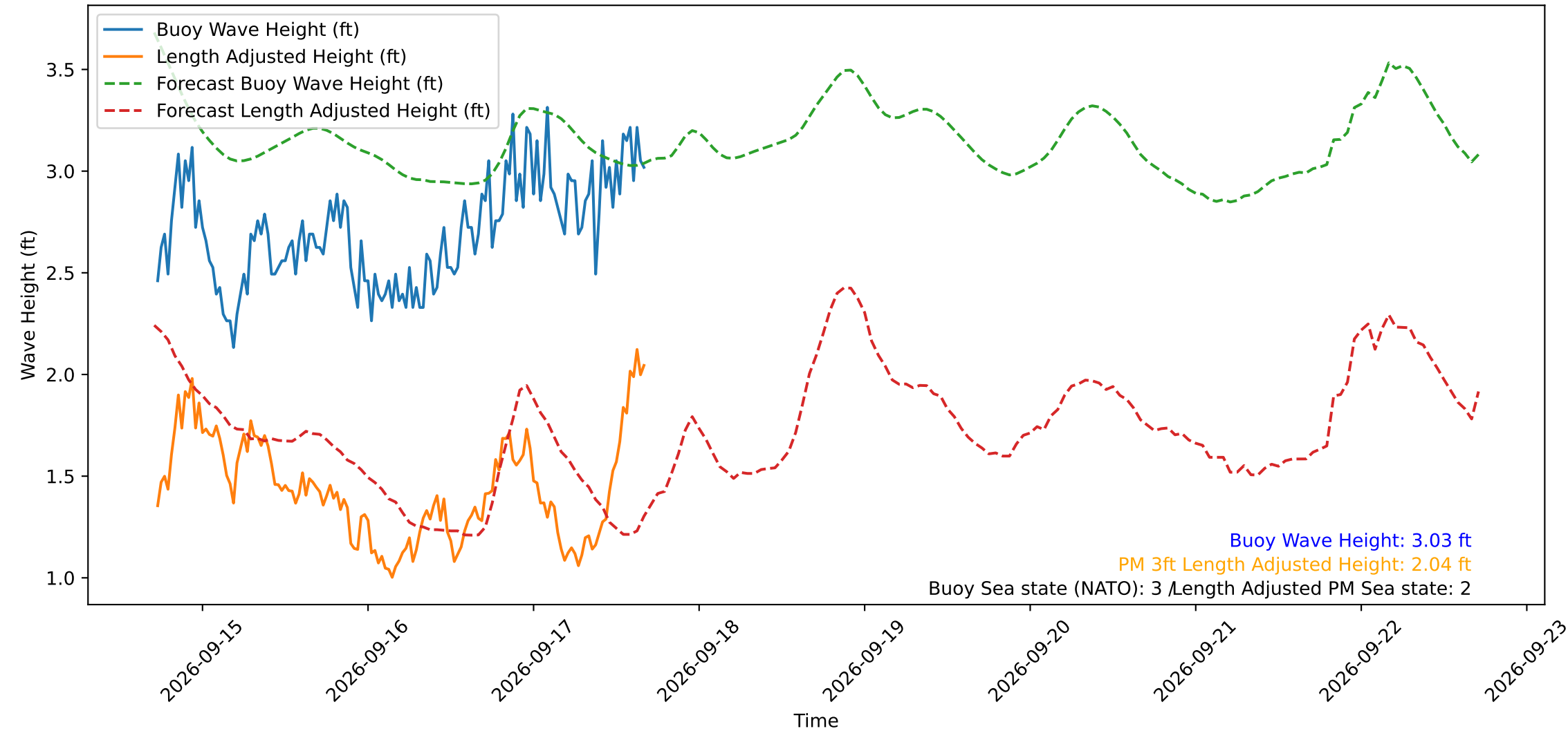
Wave Heights over Time for Green Beach at 2026-09-17 17:01:12
