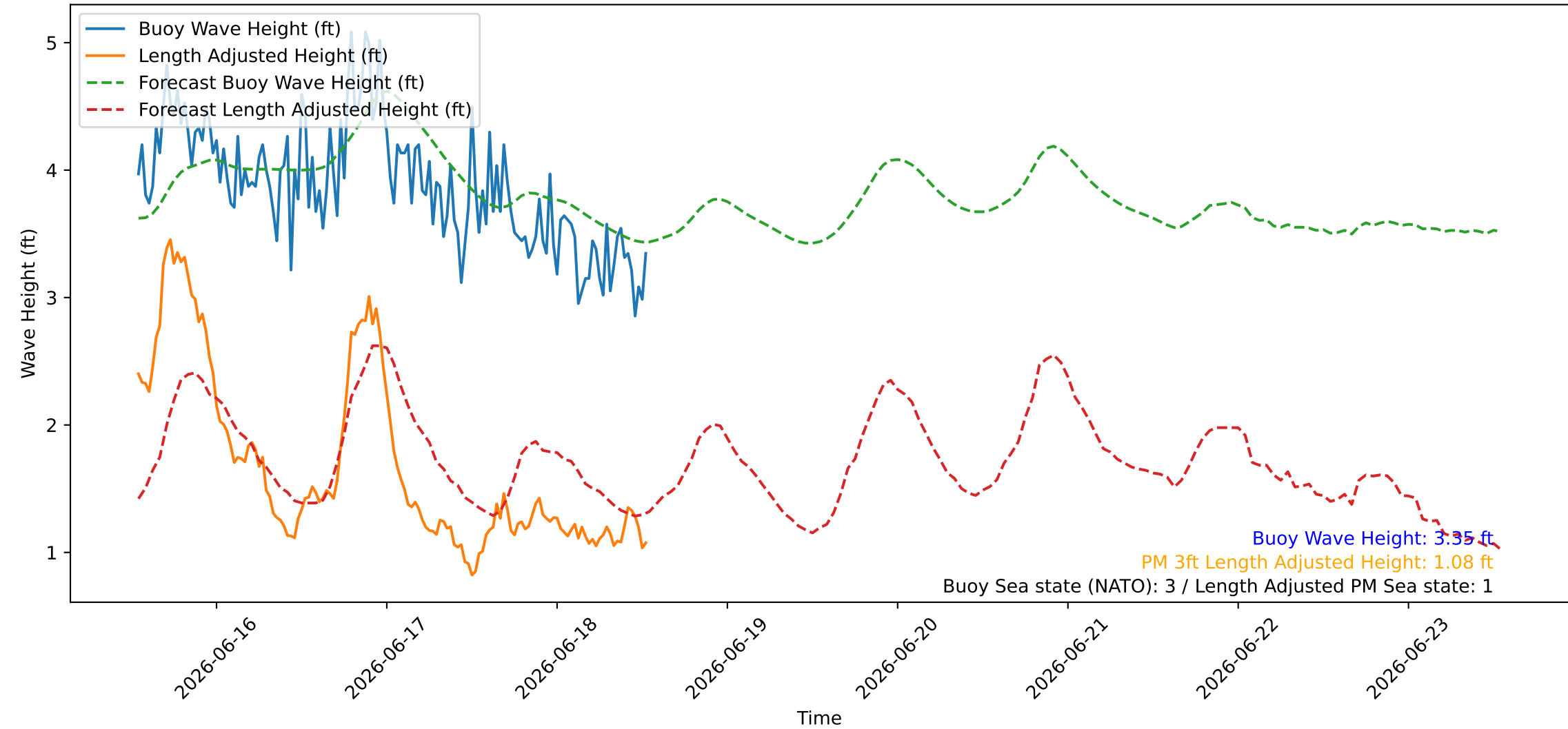
Wave Heights over Time for Green Beach at 2026-06-18 13:11:08
