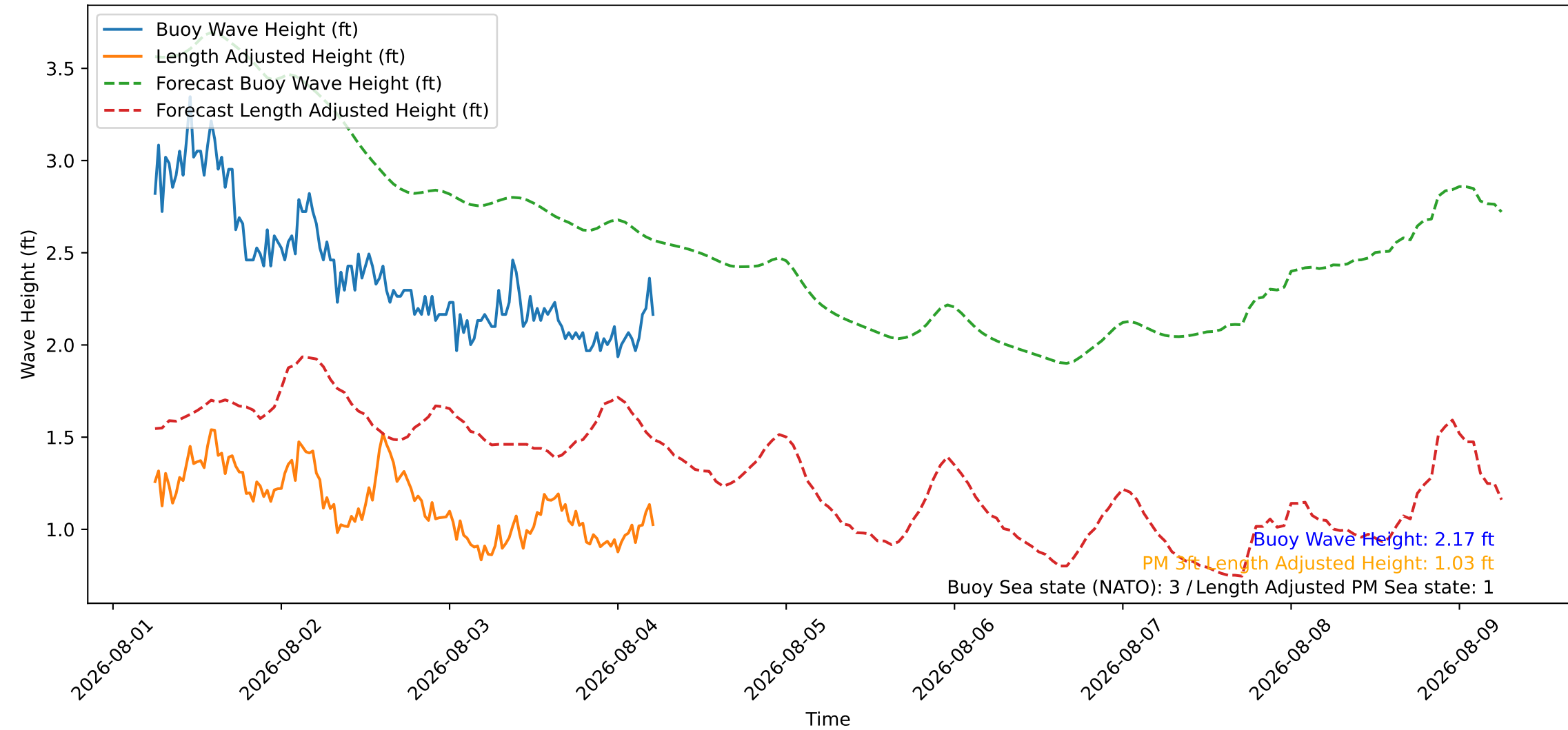
Wave Heights over Time for Red Beach at 2026-08-04 05:40:45
