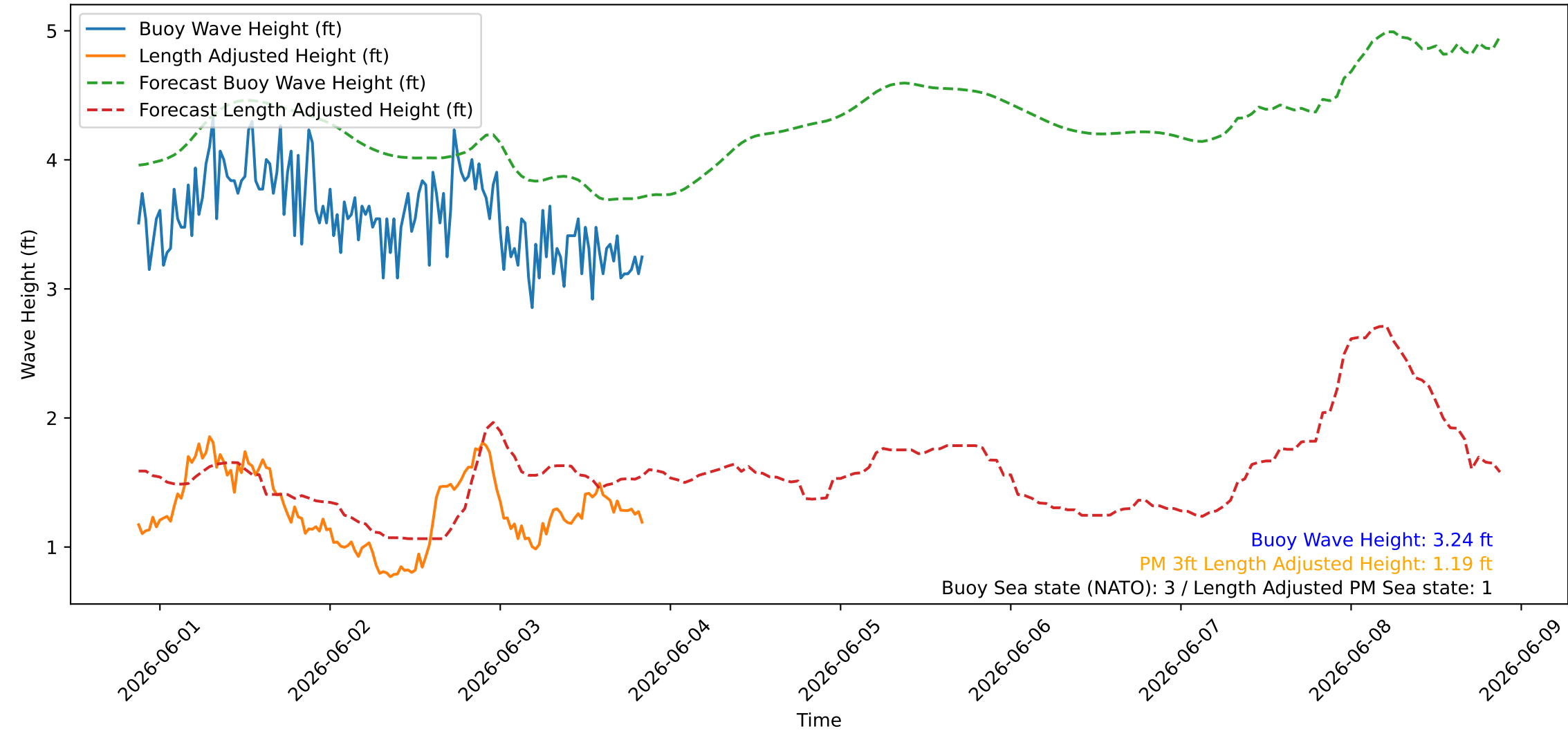
Wave Heights over Time for Green Beach at 2026-06-03 21:01:08
