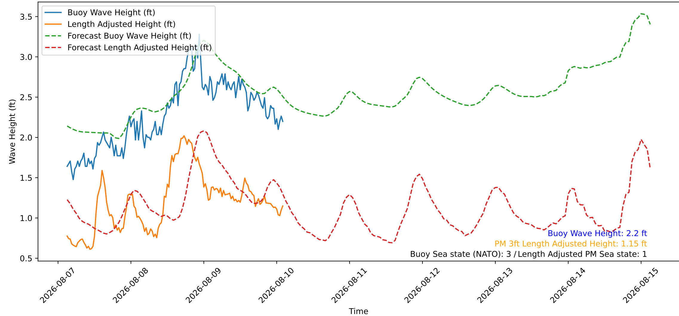
Wave Heights over Time for Red Beach at 2026-08-10 02:50:48
