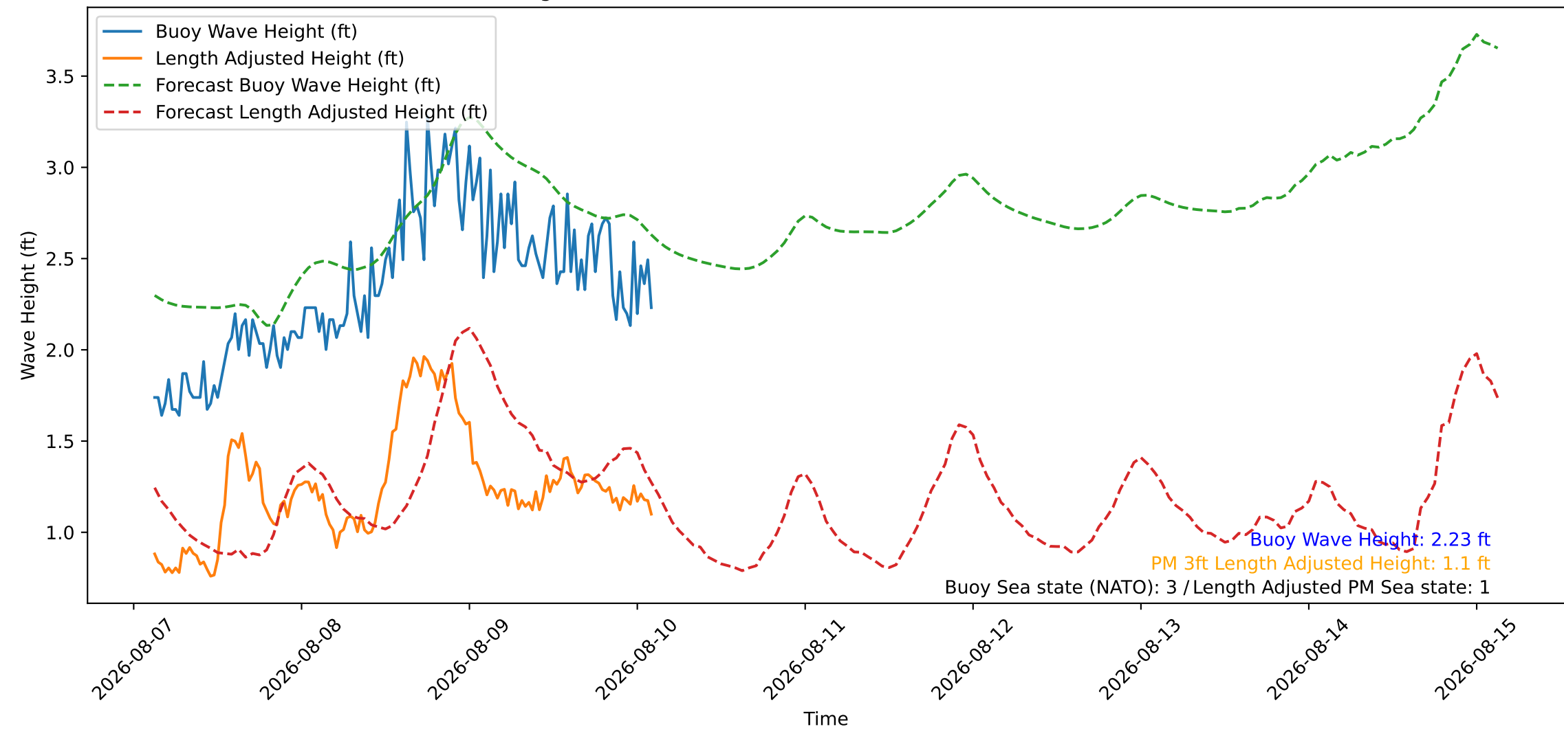
Wave Heights over Time for Oceanside Harbor at 2026-08-10 02:50:27
