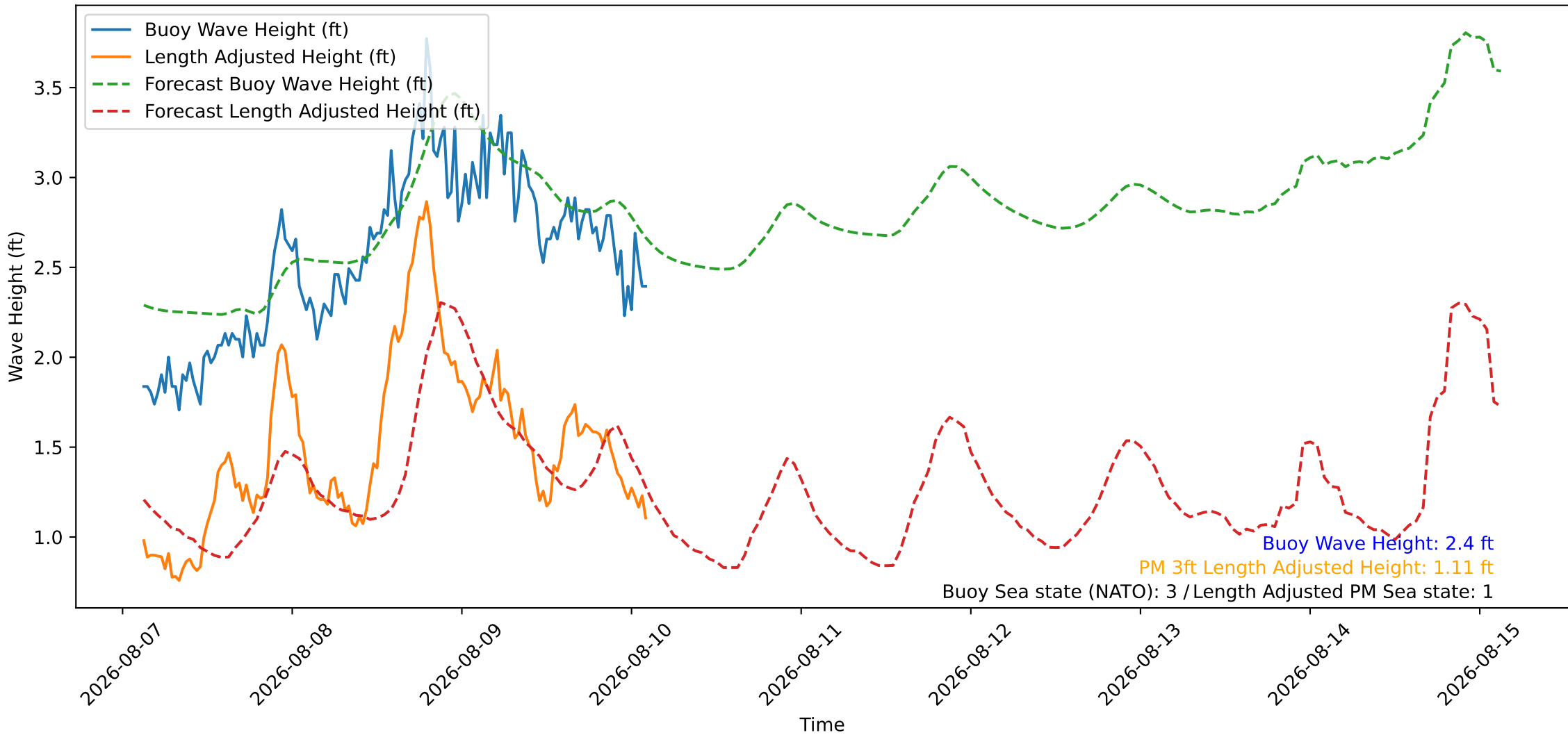
Wave Heights over Time for Green Beach at 2026-08-10 02:51:10
