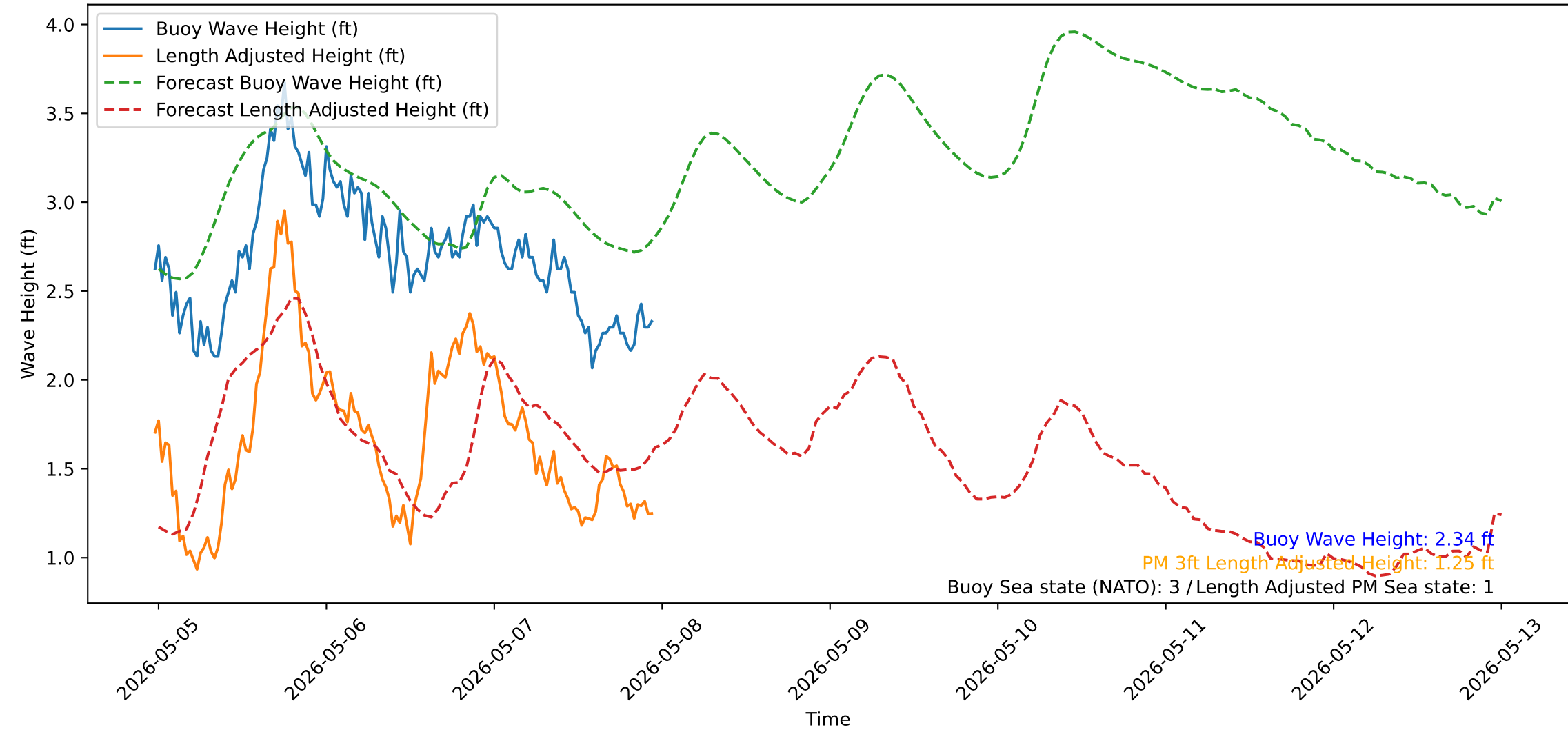
Wave Heights over Time for Green Beach at 2026-05-07 23:31:12
