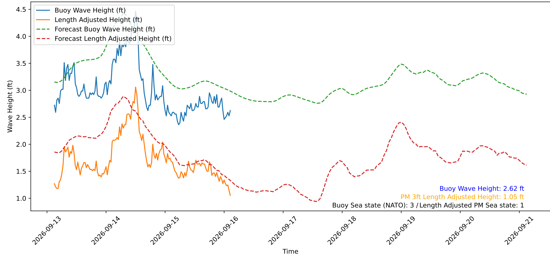
Wave Heights over Time for Oceanside Harbor at 2026-09-16 03:10:29
