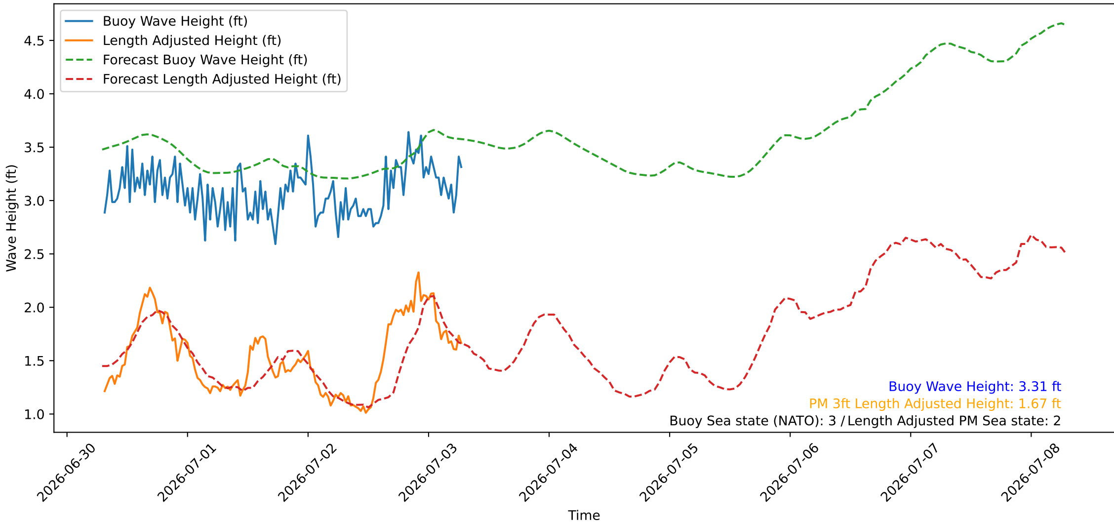
Wave Heights over Time for Oceanside Harbor at 2026-07-03 07:20:26
