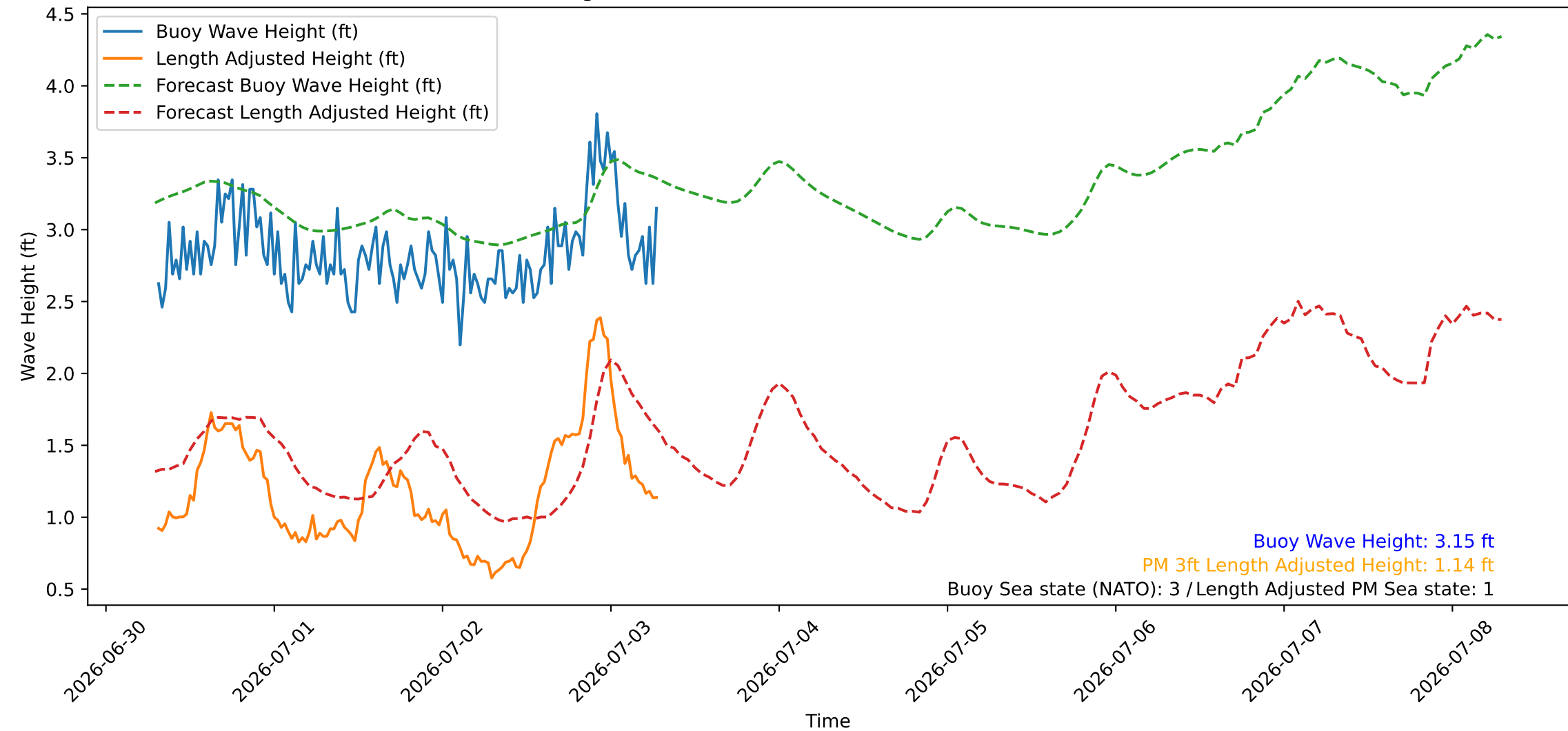
Wave Heights over Time for Red Beach at 2026-07-03 07:20:47
