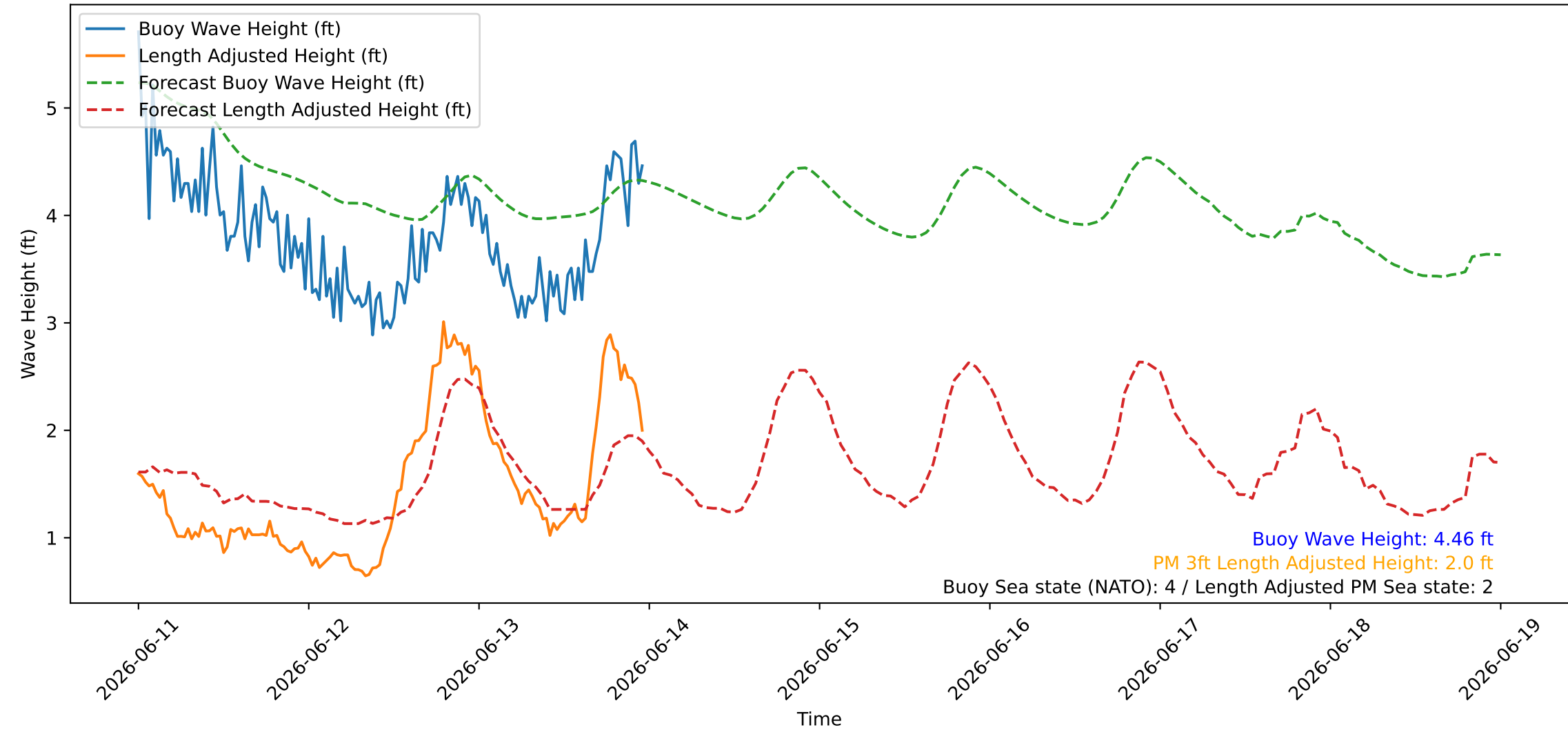
Wave Heights over Time for Green Beach at 2026-06-13 23:51:11
