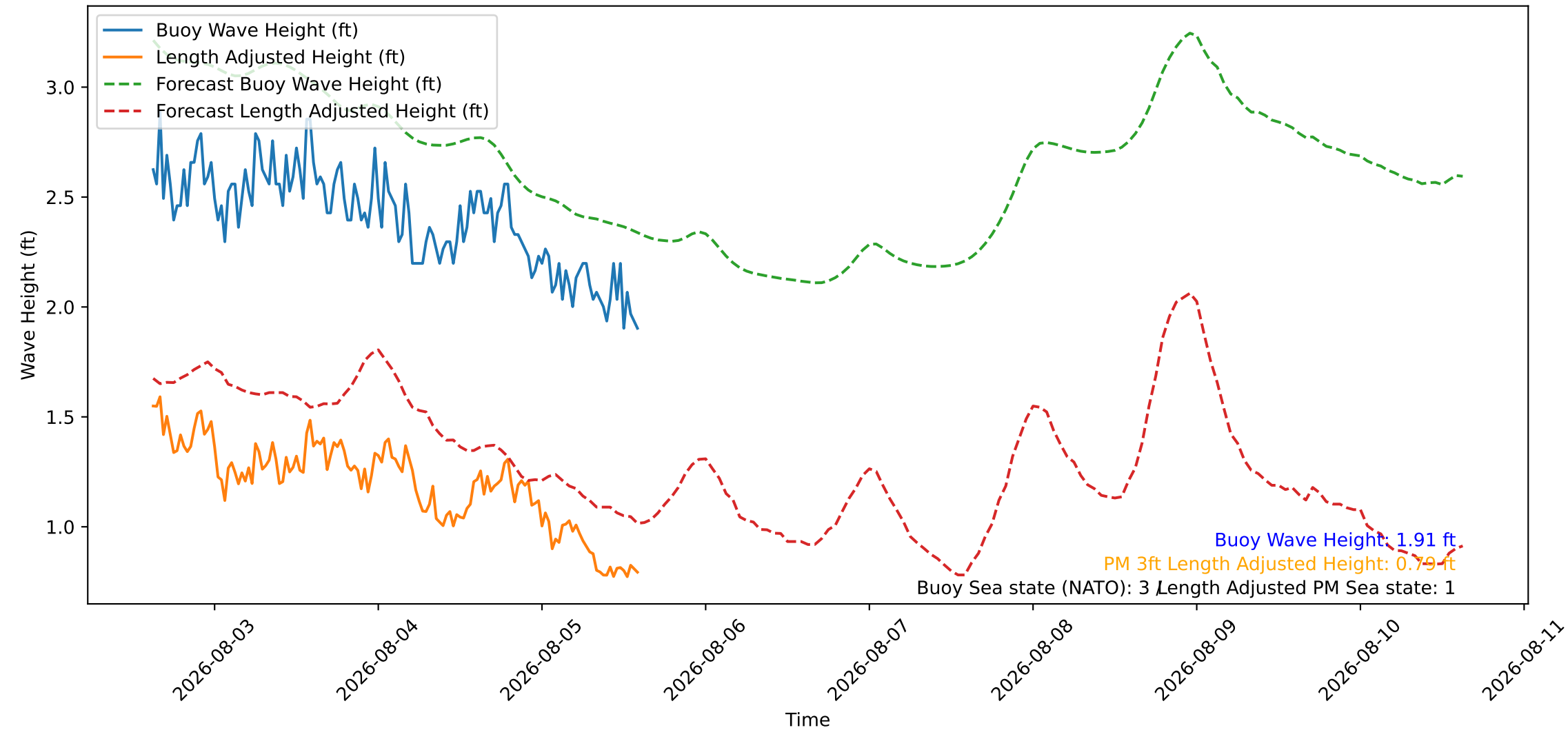
Wave Heights over Time for Oceanside Harbor at 2026-08-05 15:00:26
