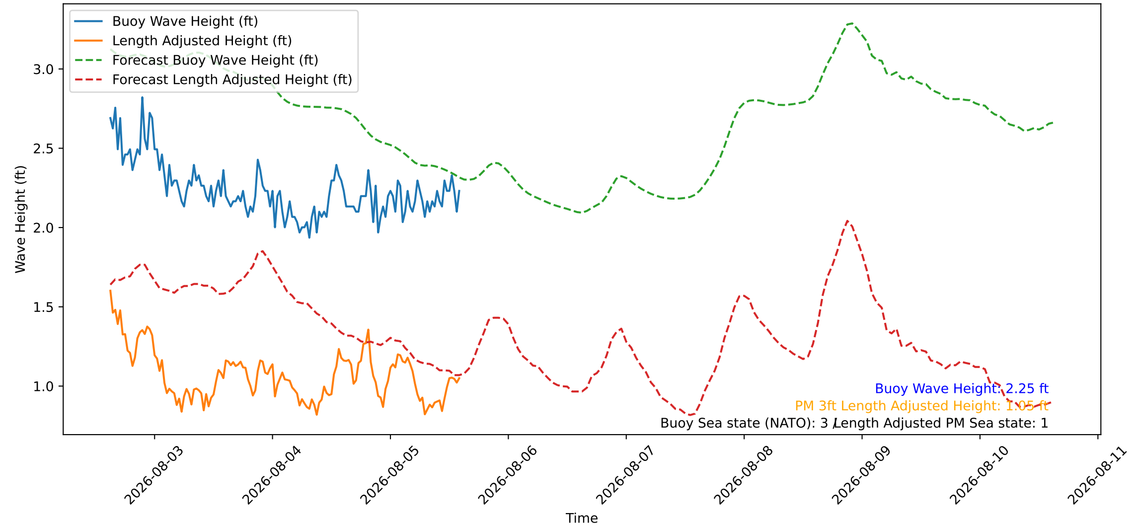
Wave Heights over Time for Green Beach at 2026-08-05 15:01:08
