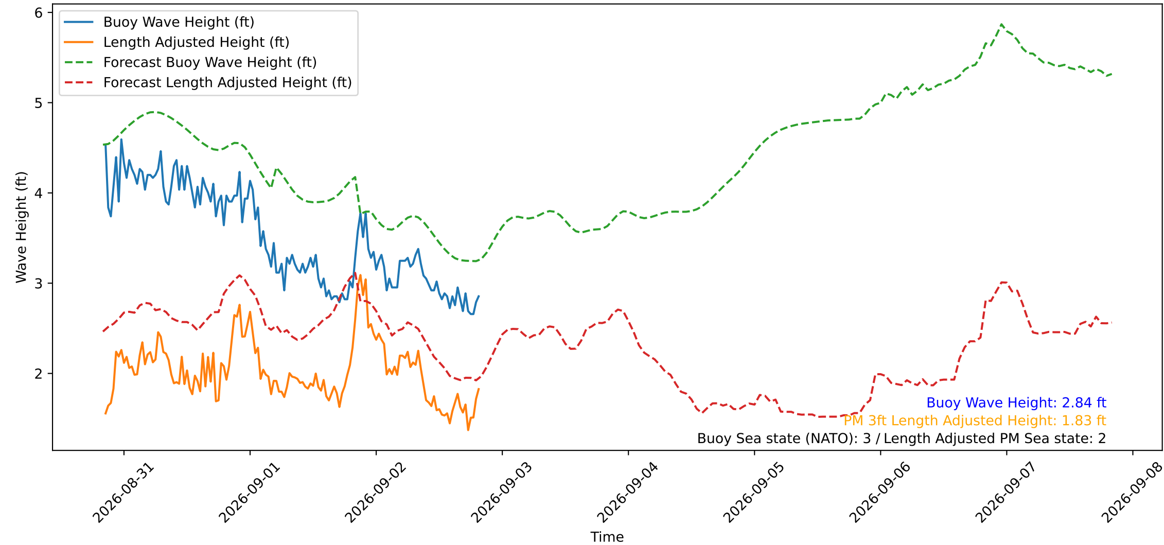
Wave Heights over Time for Green Beach at 2026-09-02 20:21:16
