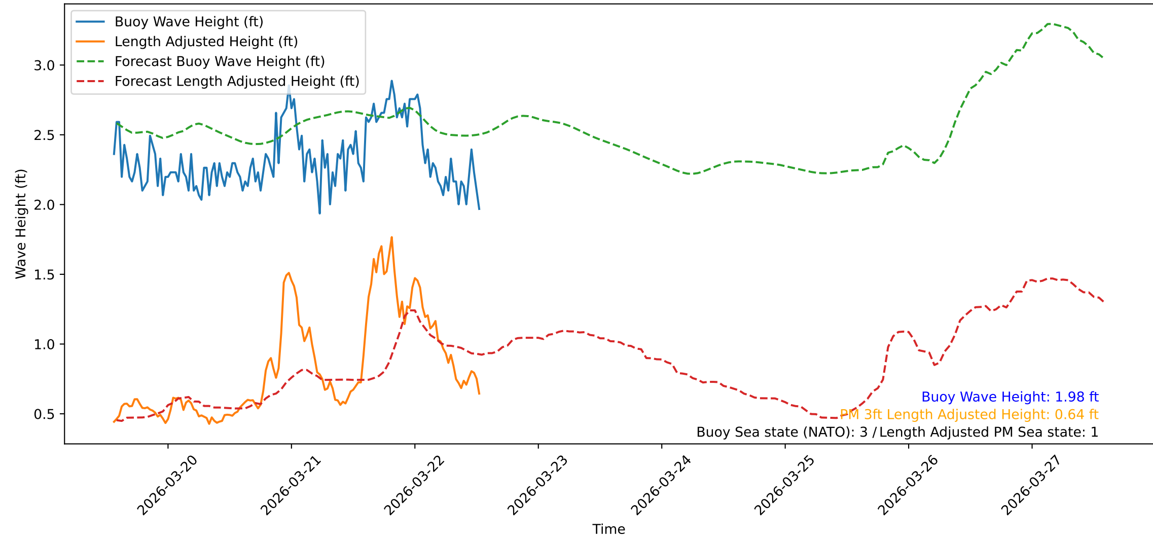
Wave Heights over Time for Green Beach at 2026-03-22 13:31:09
