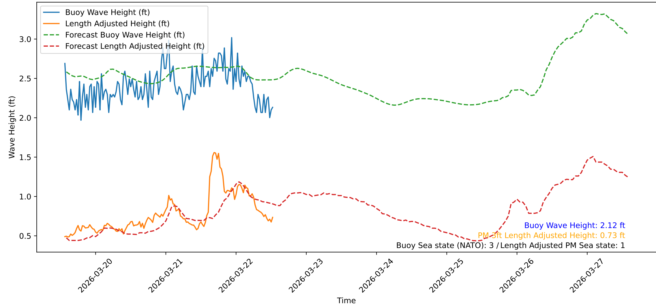
Wave Heights over Time for Oceanside Harbor at 2026-03-22 13:30:31
