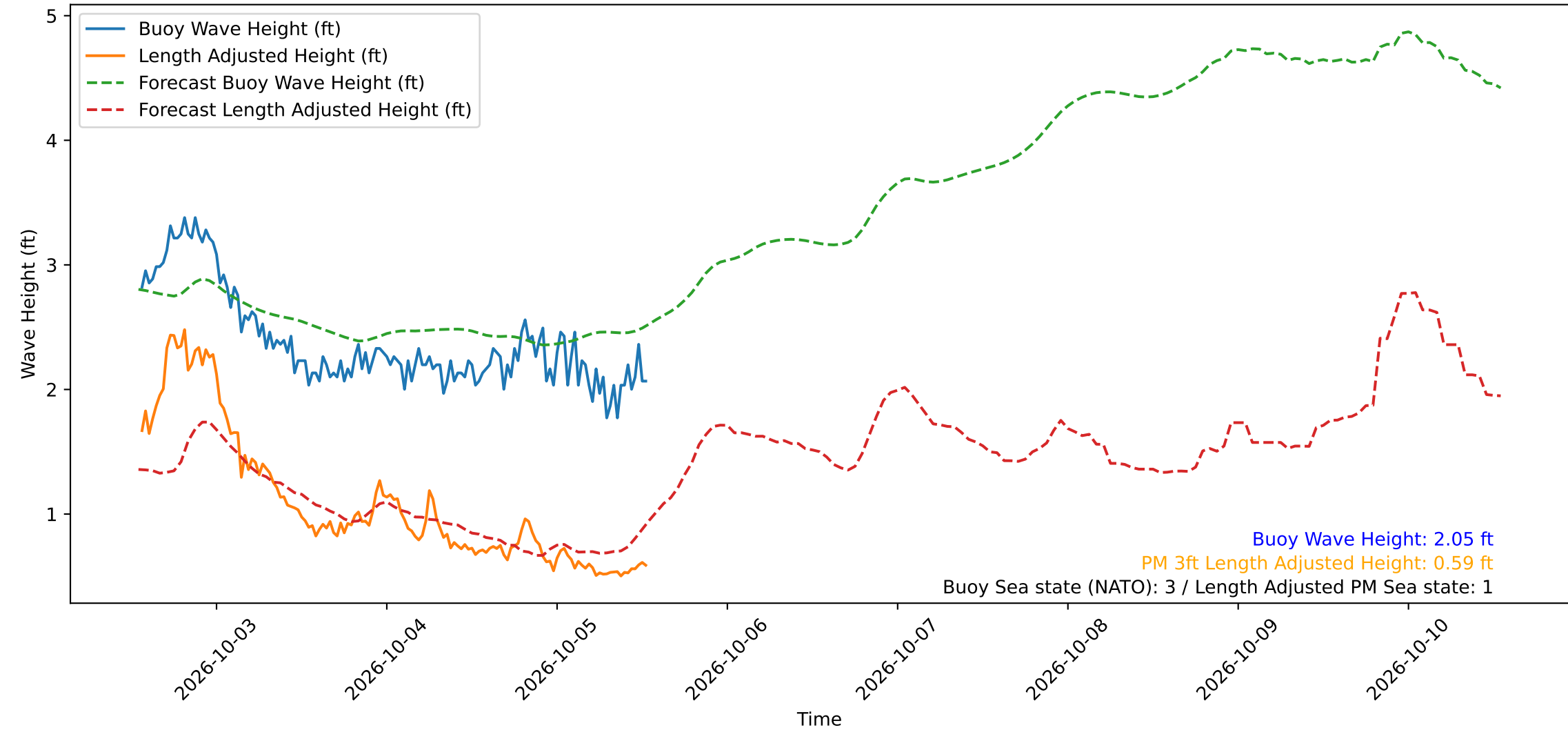
Wave Heights over Time for Green Beach at 2026-10-05 13:11:12
