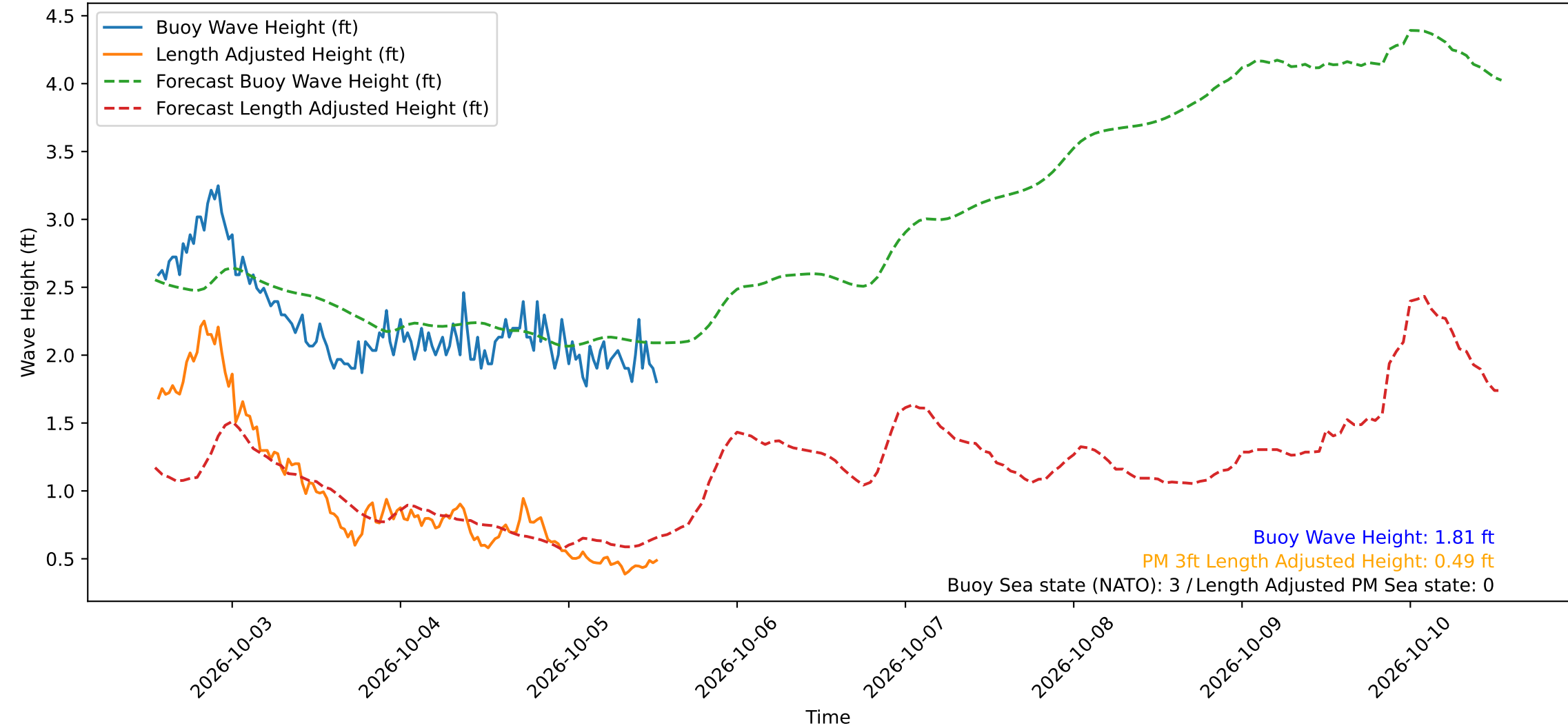
Wave Heights over Time for Red Beach at 2026-10-05 13:10:50
