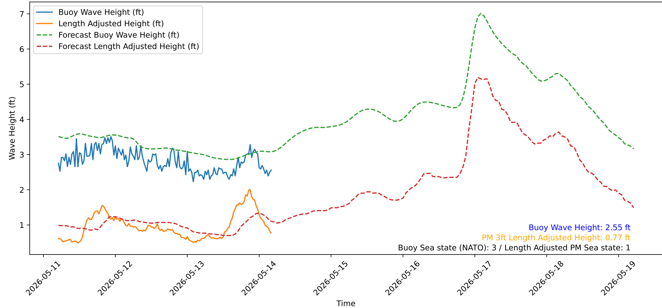
Wave Heights over Time for Green Beach at 2026-05-14 05:01:13
