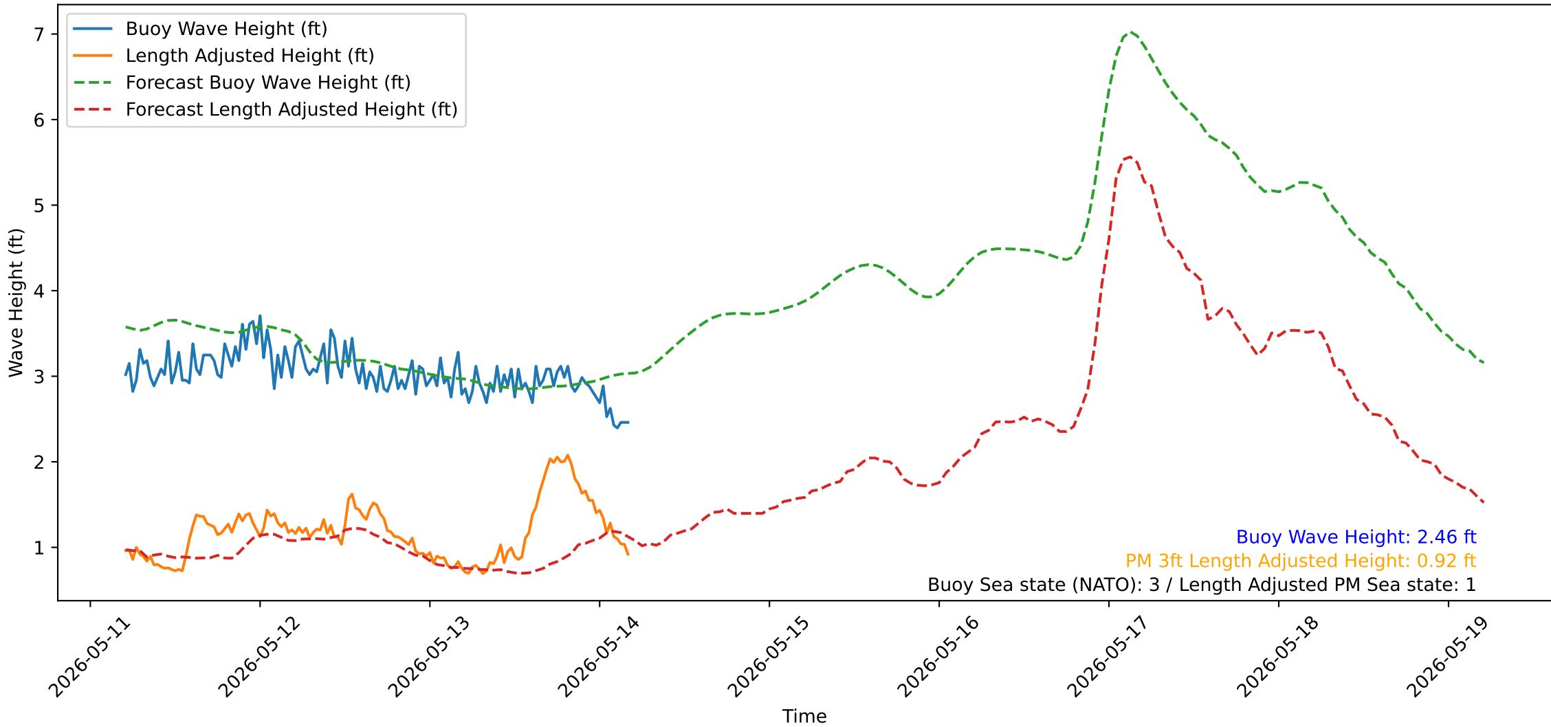
Wave Heights over Time for Oceanside Harbor at 2026-05-14 05:00:32
