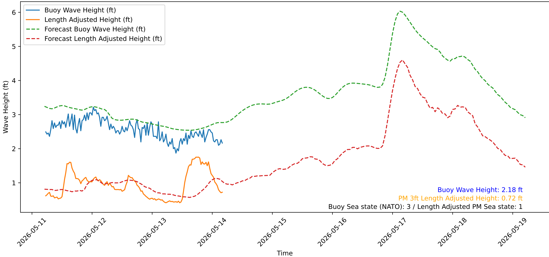
Wave Heights over Time for Red Beach at 2026-05-14 05:00:51
