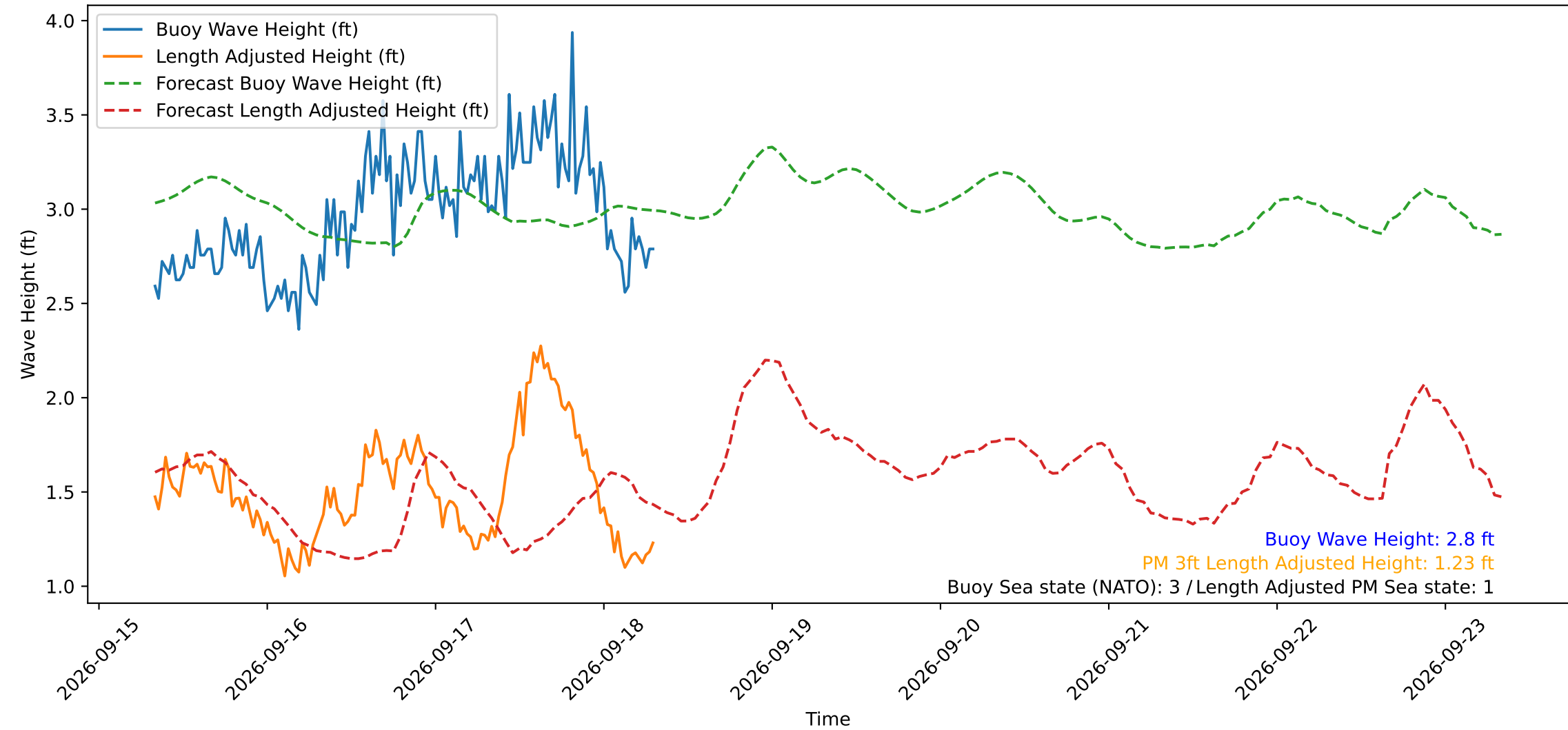
Wave Heights over Time for Oceanside Harbor at 2026-09-18 07:50:29
