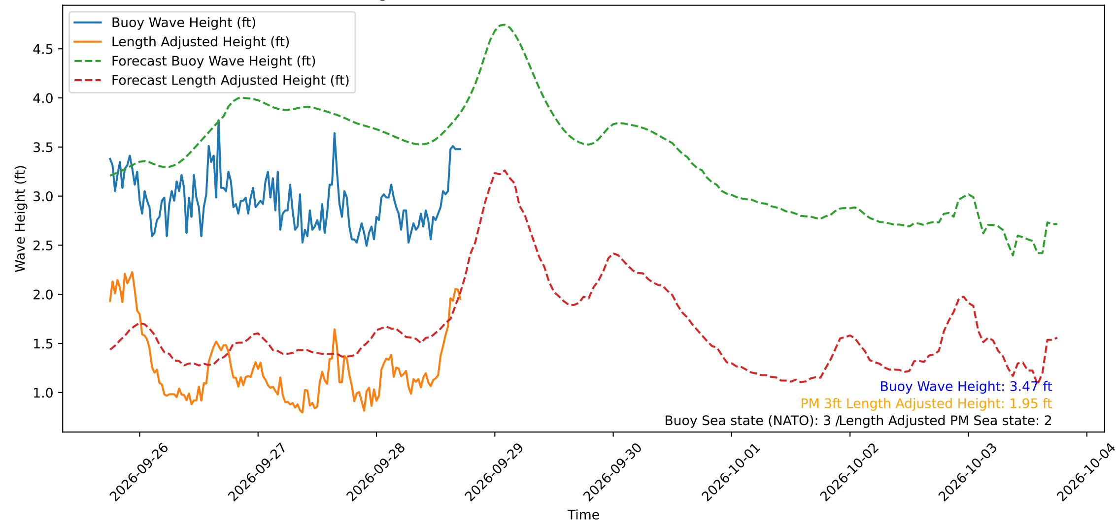
Wave Heights over Time for Oceanside Harbor at 2026-09-28 17:50:30
