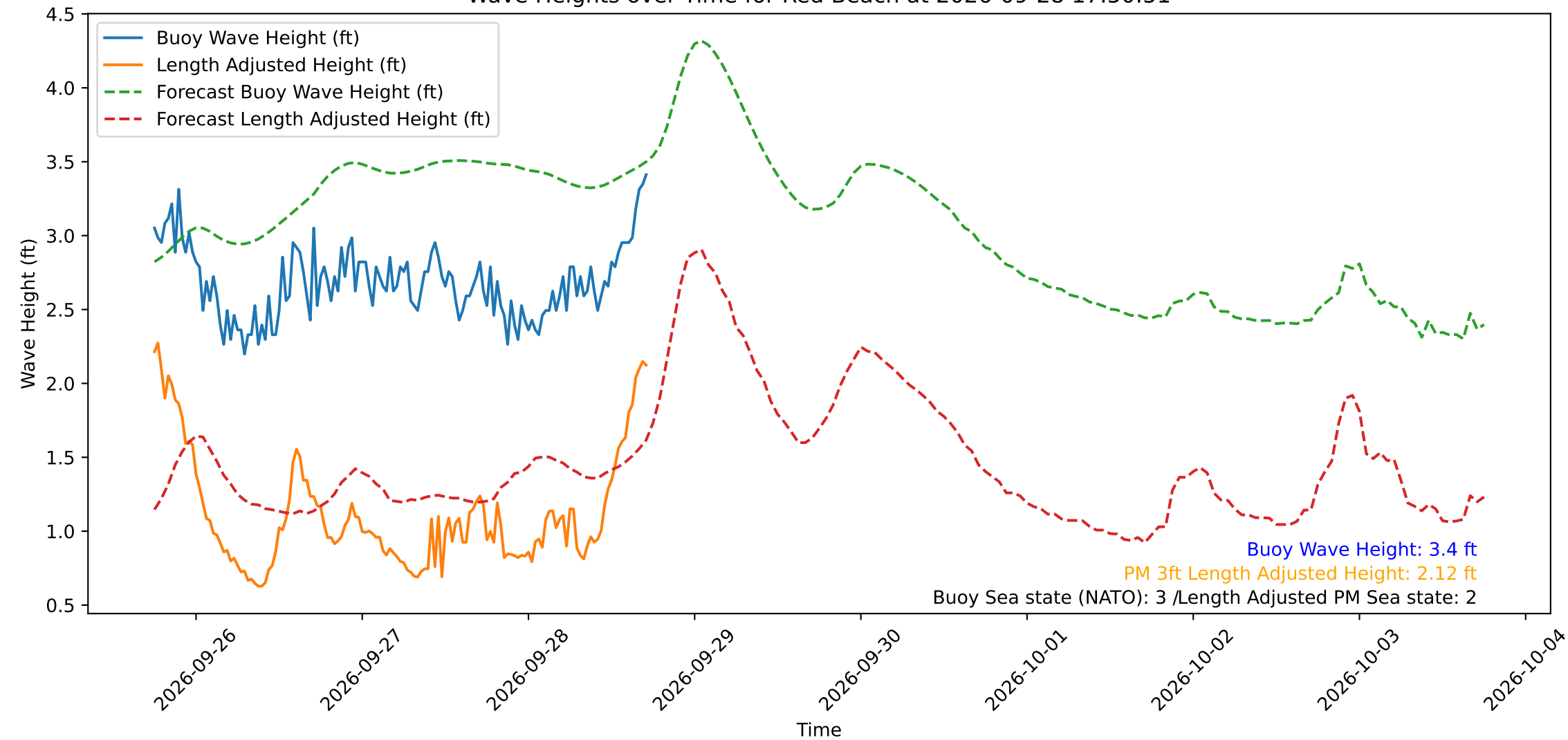
Wave Heights over Time for Red Beach at 2026-09-28 17:50:51
