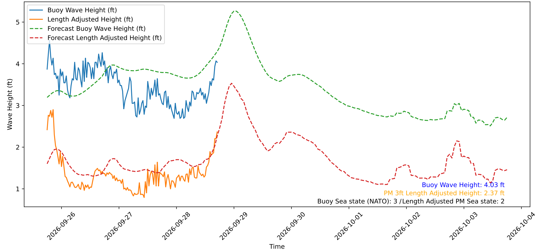
Wave Heights over Time for Green Beach at 2026-09-28 17:51:15
