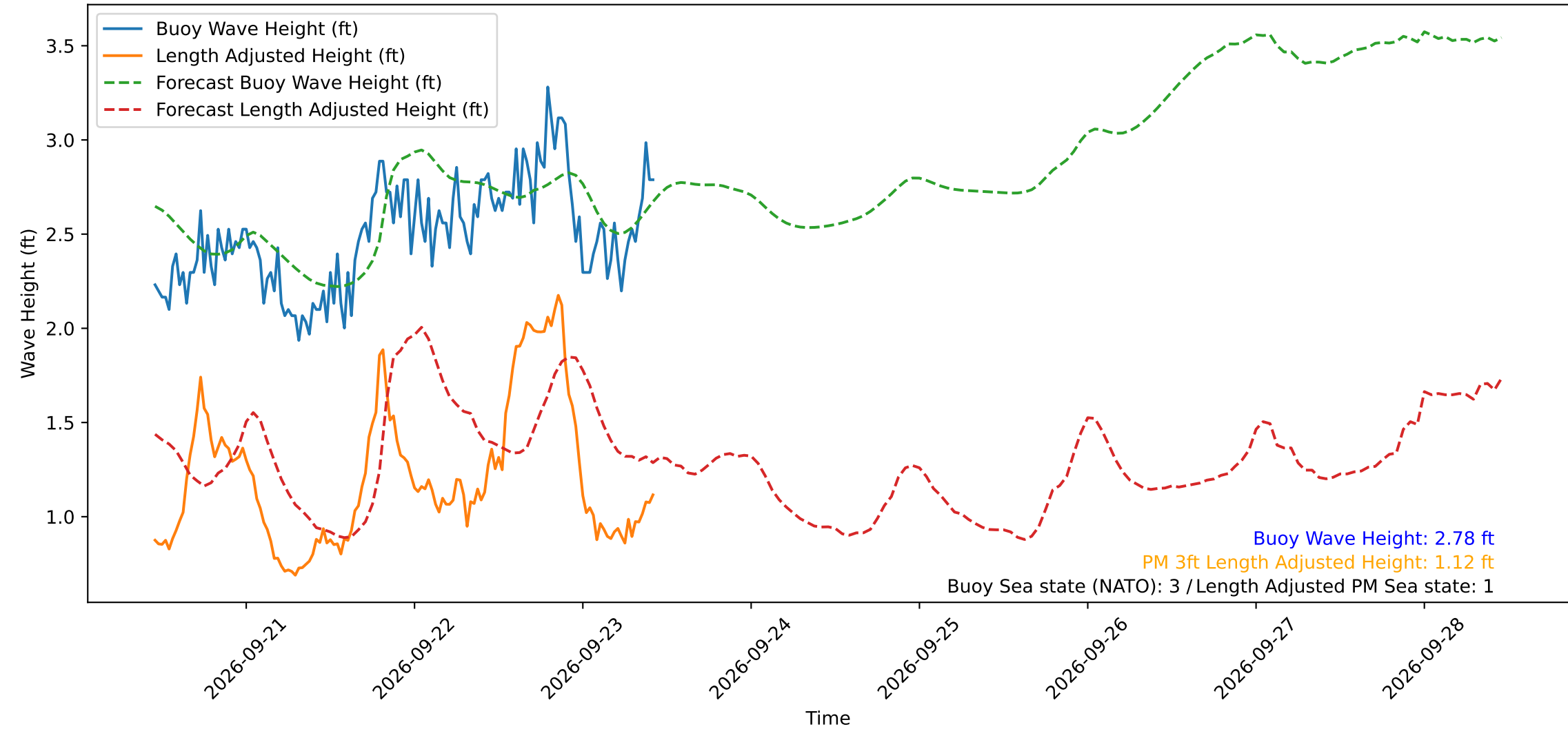
Wave Heights over Time for Red Beach at 2026-09-23 10:50:50
