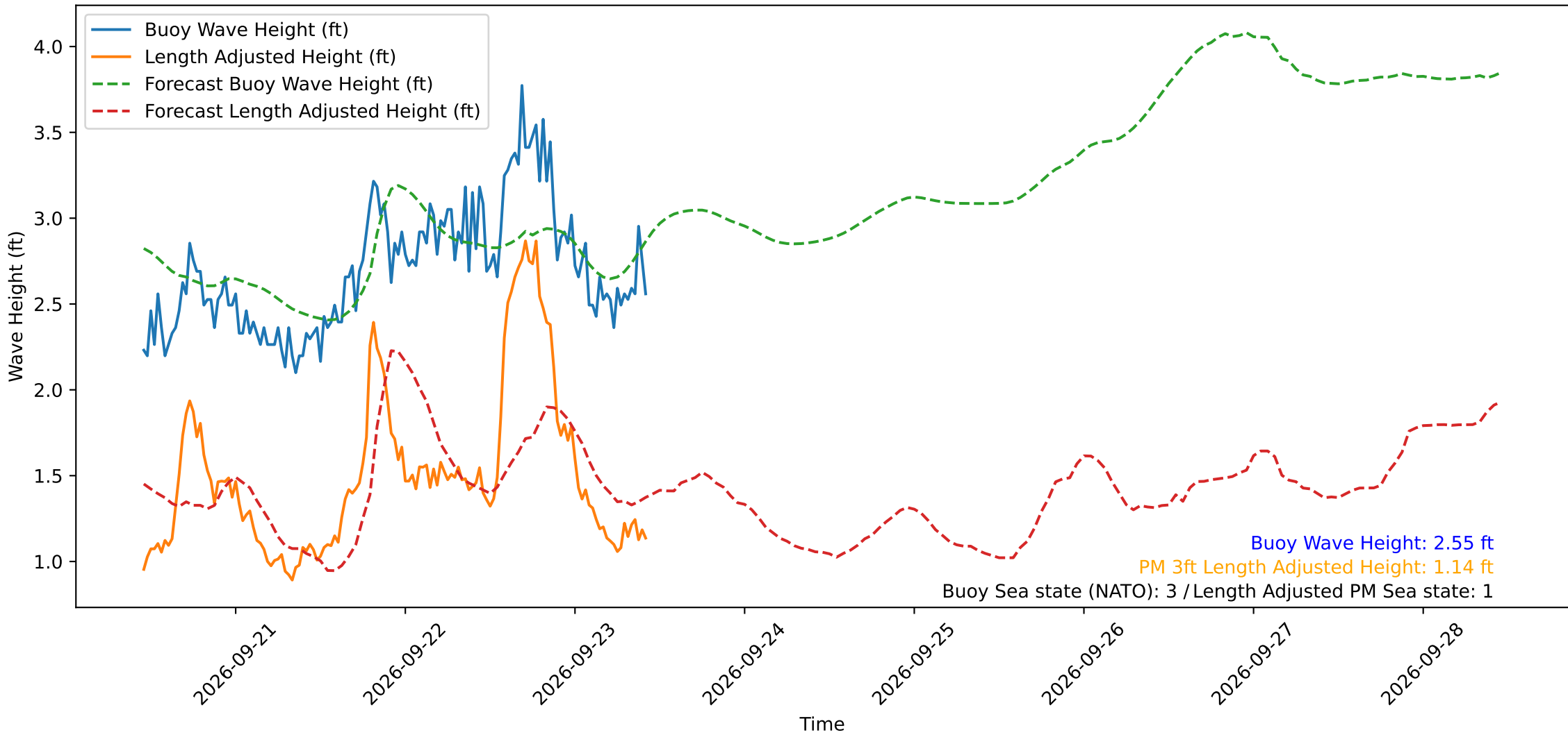
Wave Heights over Time for Oceanside Harbor at 2026-09-23 10:50:29
