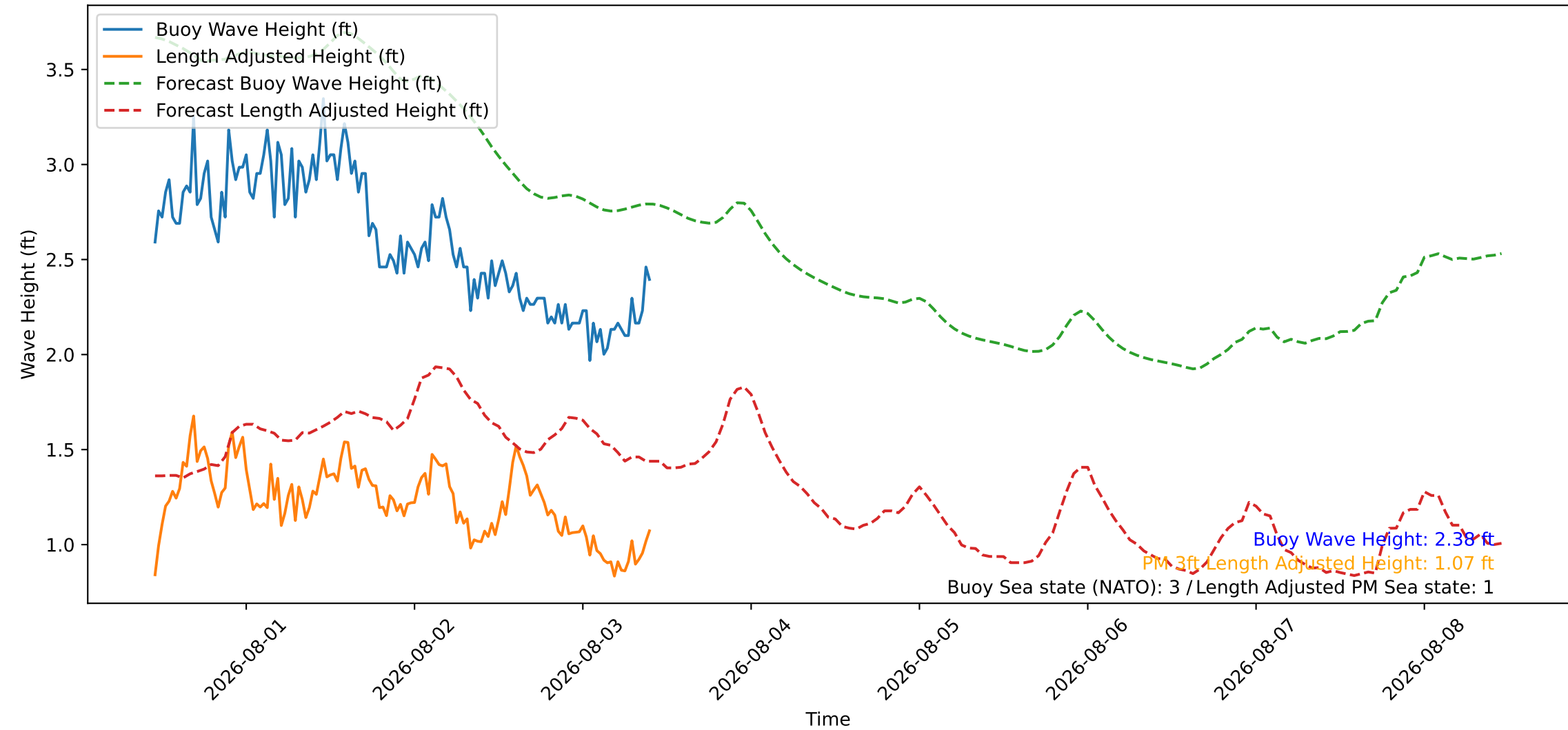
Wave Heights over Time for Red Beach at 2026-08-03 10:40:46
