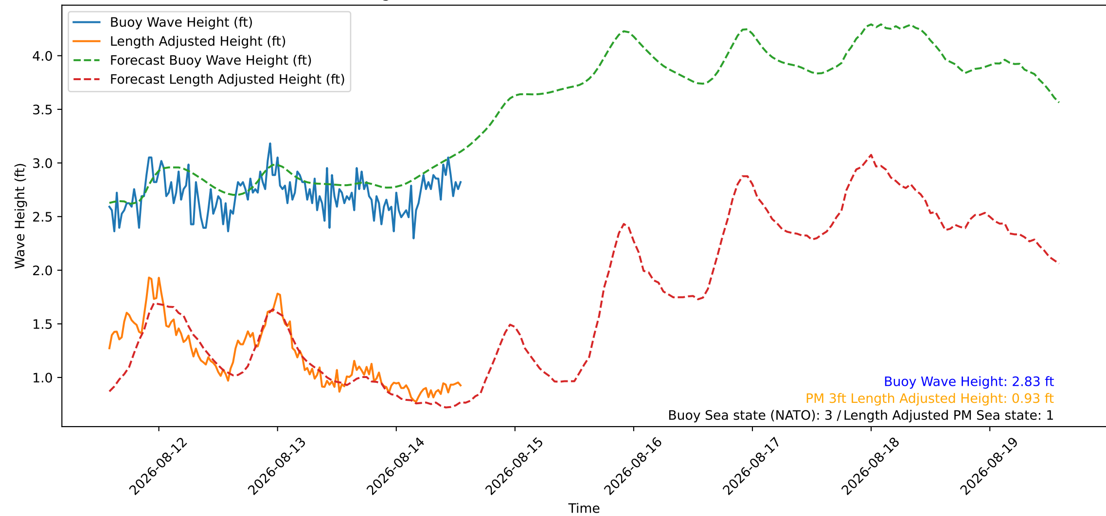
Wave Heights over Time for Oceanside Harbor at 2026-08-14 13:50:26
