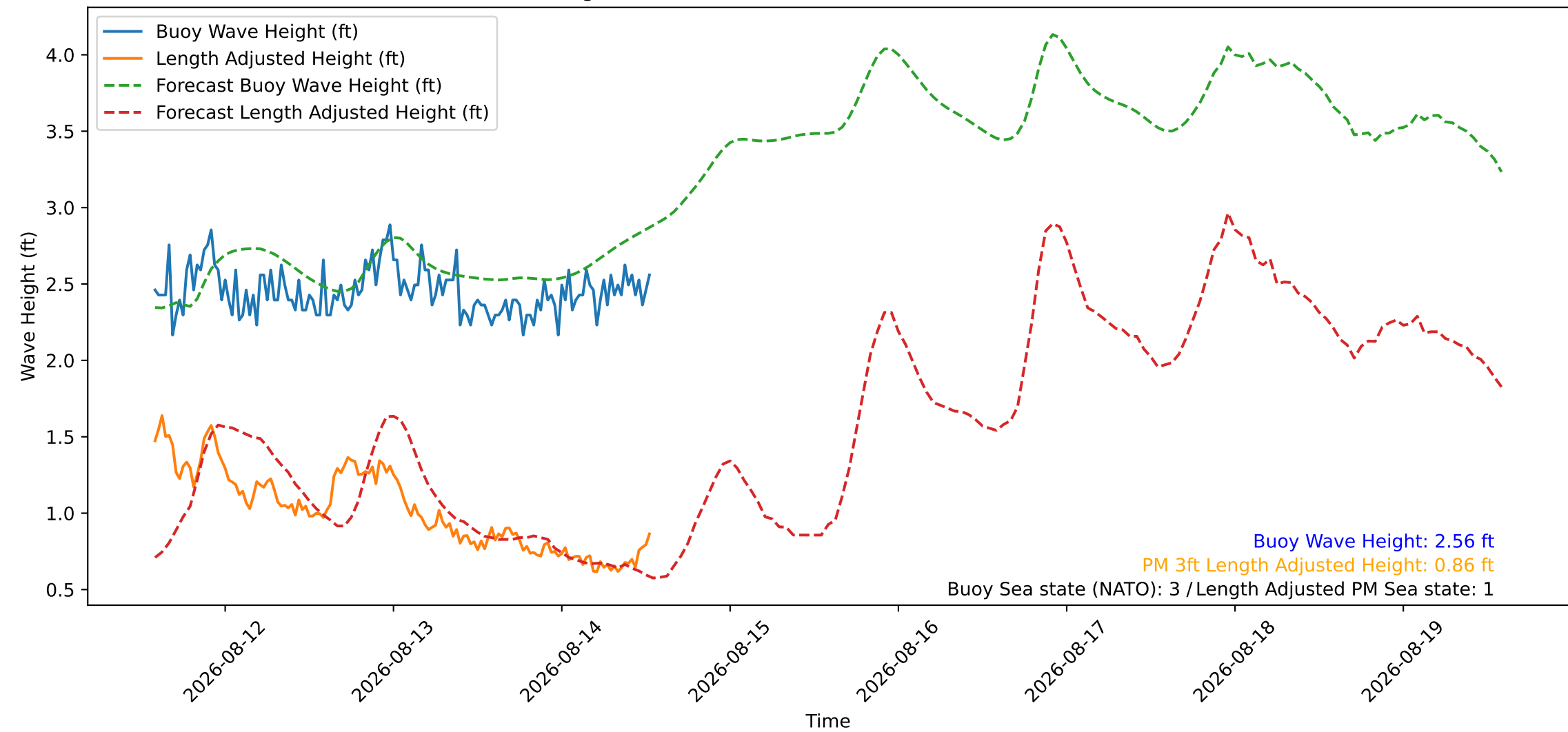
Wave Heights over Time for Red Beach at 2026-08-14 13:50:47
