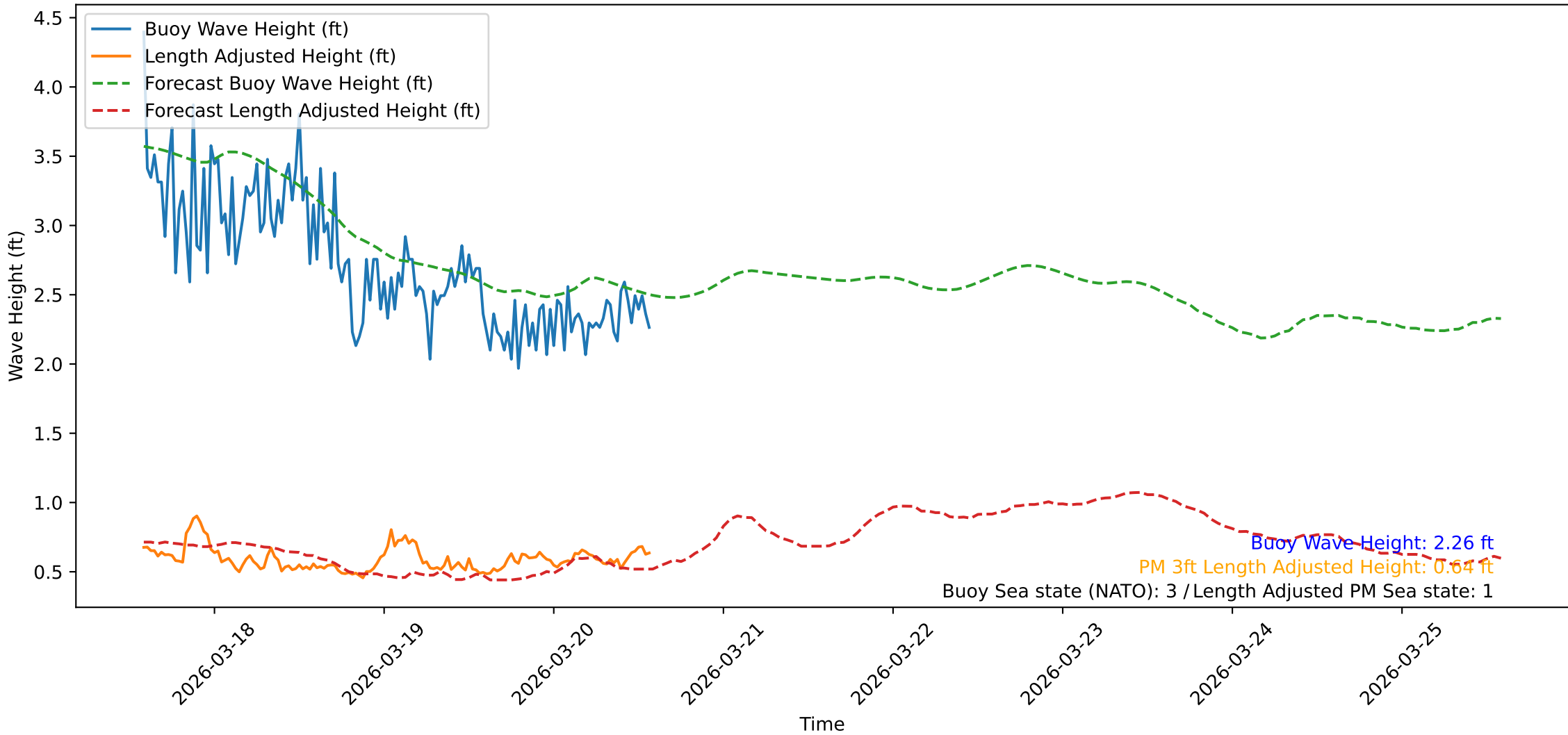
Wave Heights over Time for Oceanside Harbor at 2026-03-20 14:00:32
