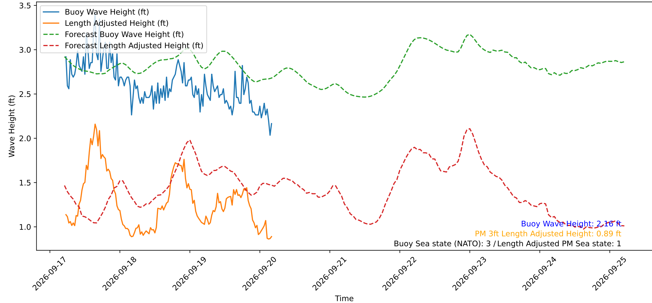
Wave Heights over Time for Red Beach at 2026-09-20 05:00:48
