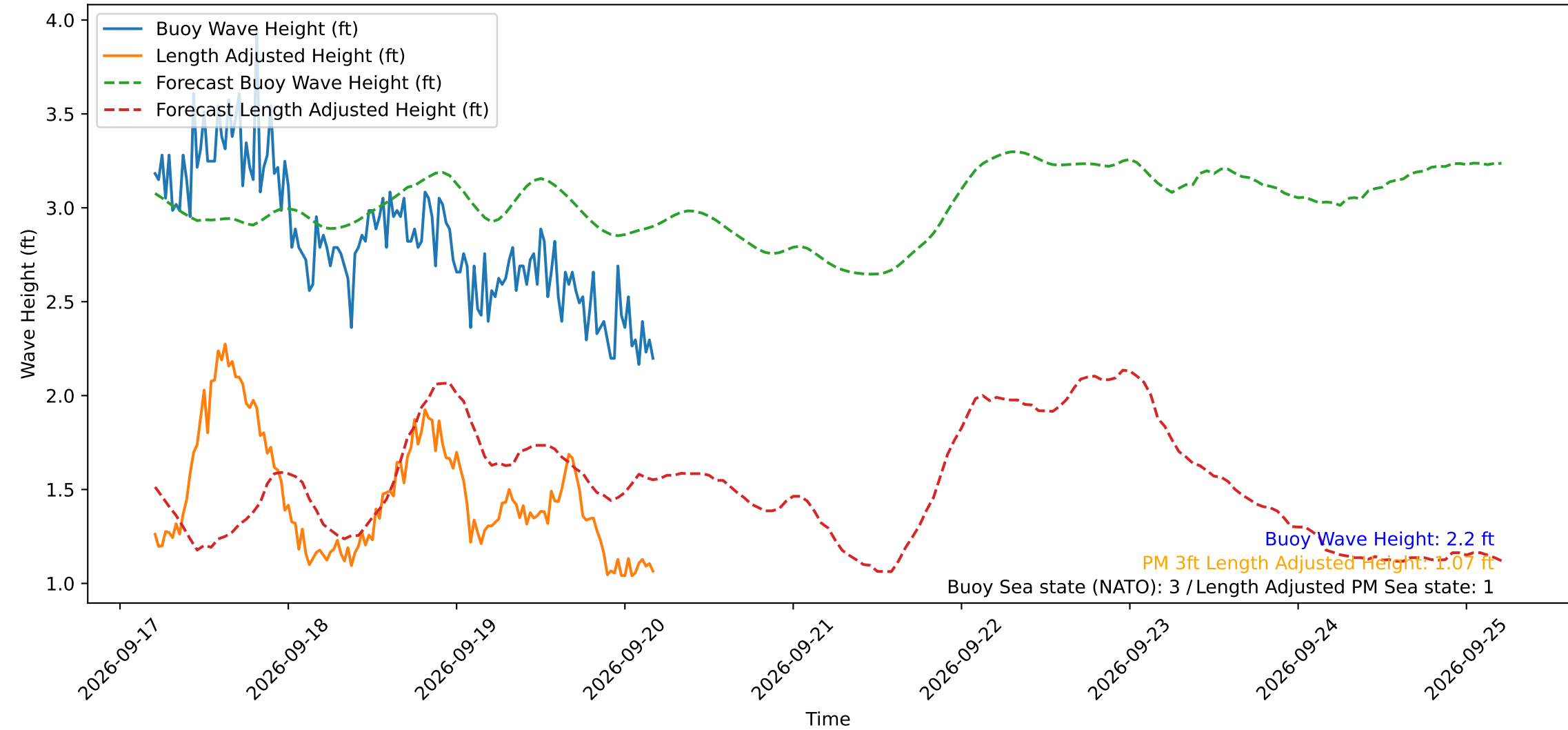
Wave Heights over Time for Oceanside Harbor at 2026-09-20 05:00:29
