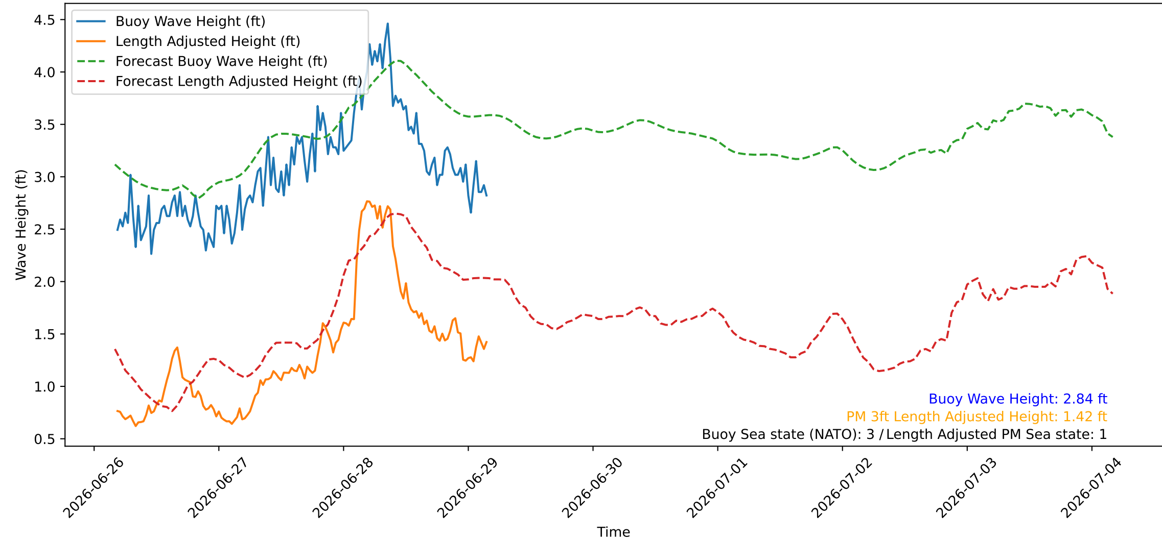
Wave Heights over Time for Red Beach at 2026-06-29 04:10:45
