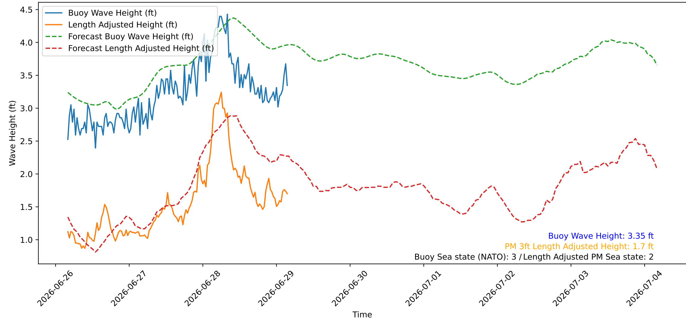
Wave Heights over Time for Oceanside Harbor at 2026-06-29 04:10:26
