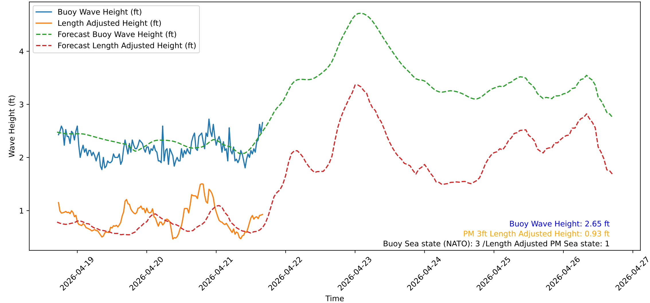
Wave Heights over Time for Red Beach at 2026-04-21 17:10:50
