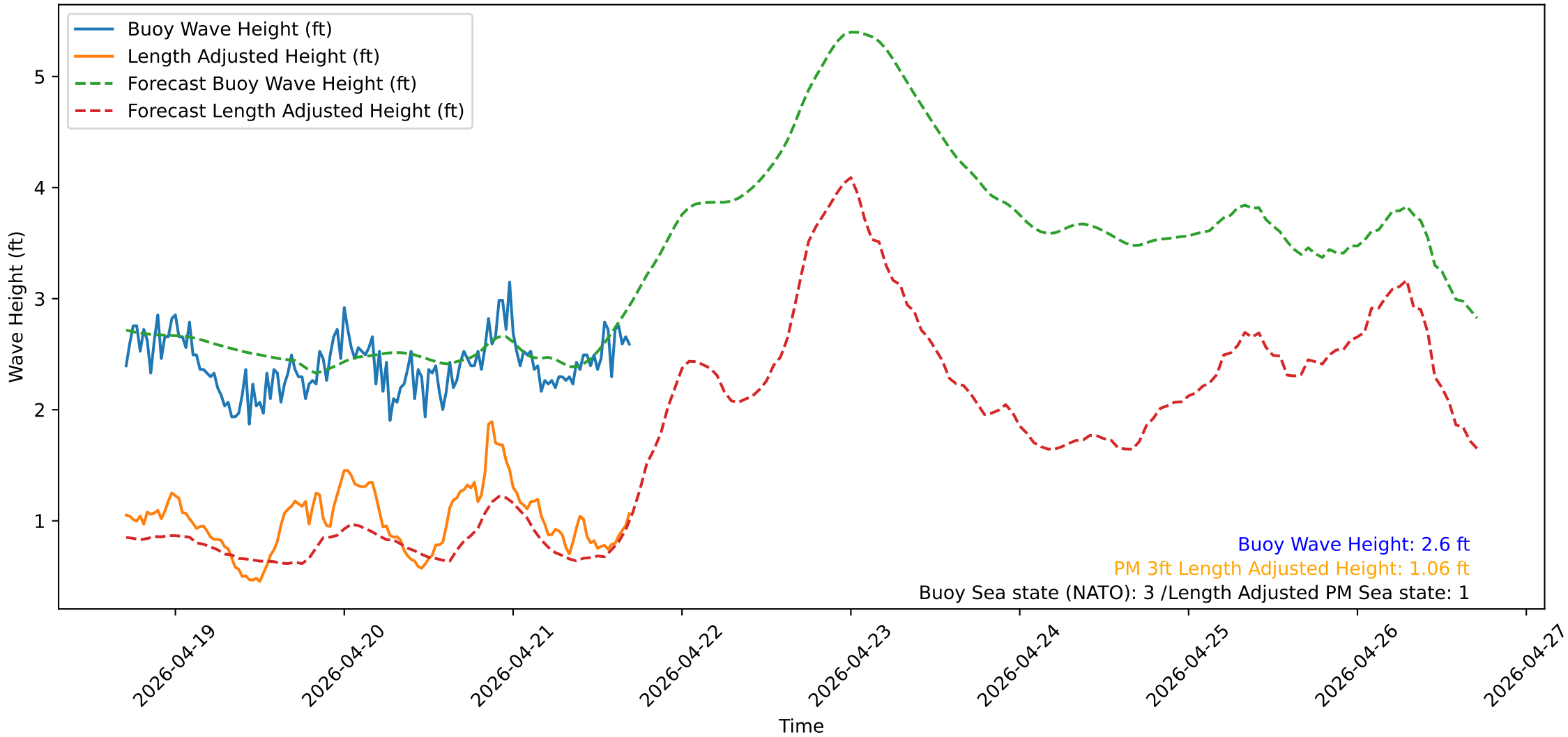
Wave Heights over Time for Green Beach at 2026-04-21 17:11:12
