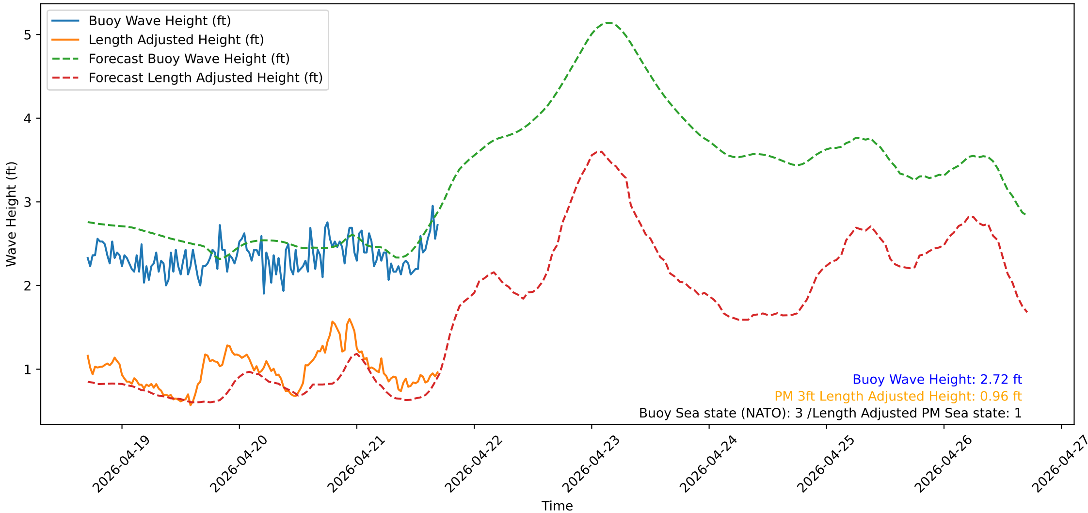
Wave Heights over Time for Oceanside Harbor at 2026-04-21 17:10:31
