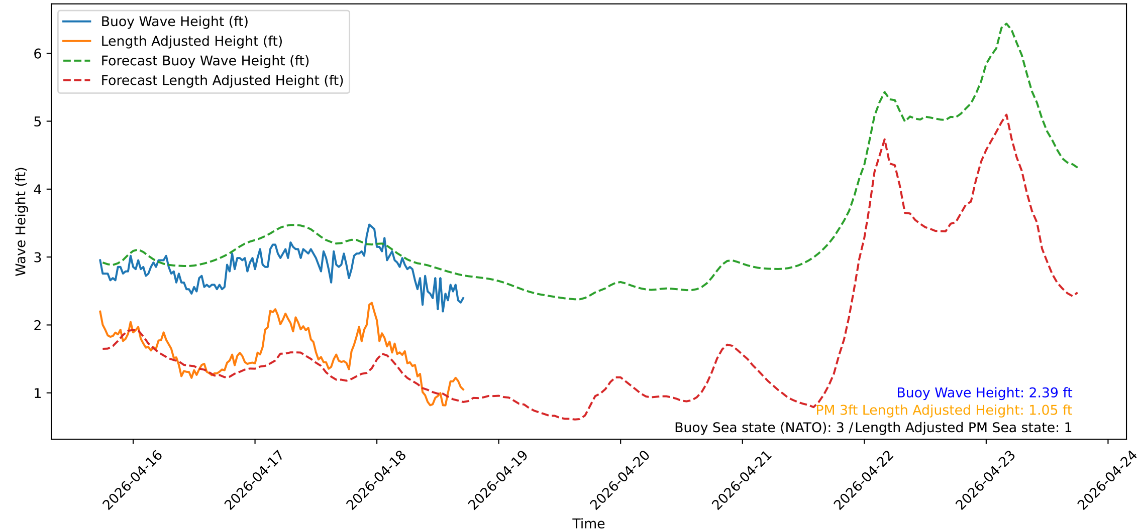
Wave Heights over Time for Green Beach at 2026-04-18 17:41:12
