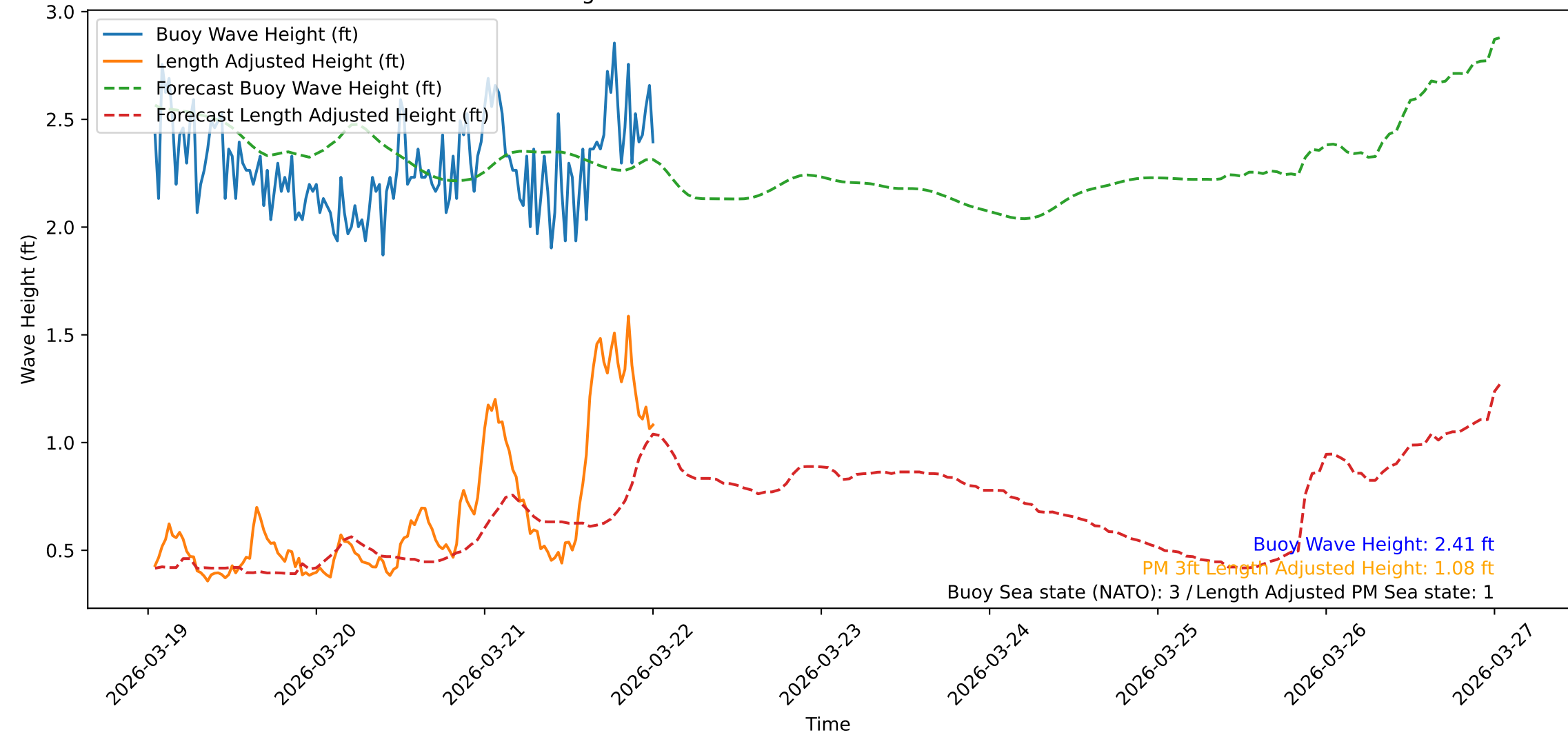
Wave Heights over Time for Red Beach at 2026-03-22 00:40:48
