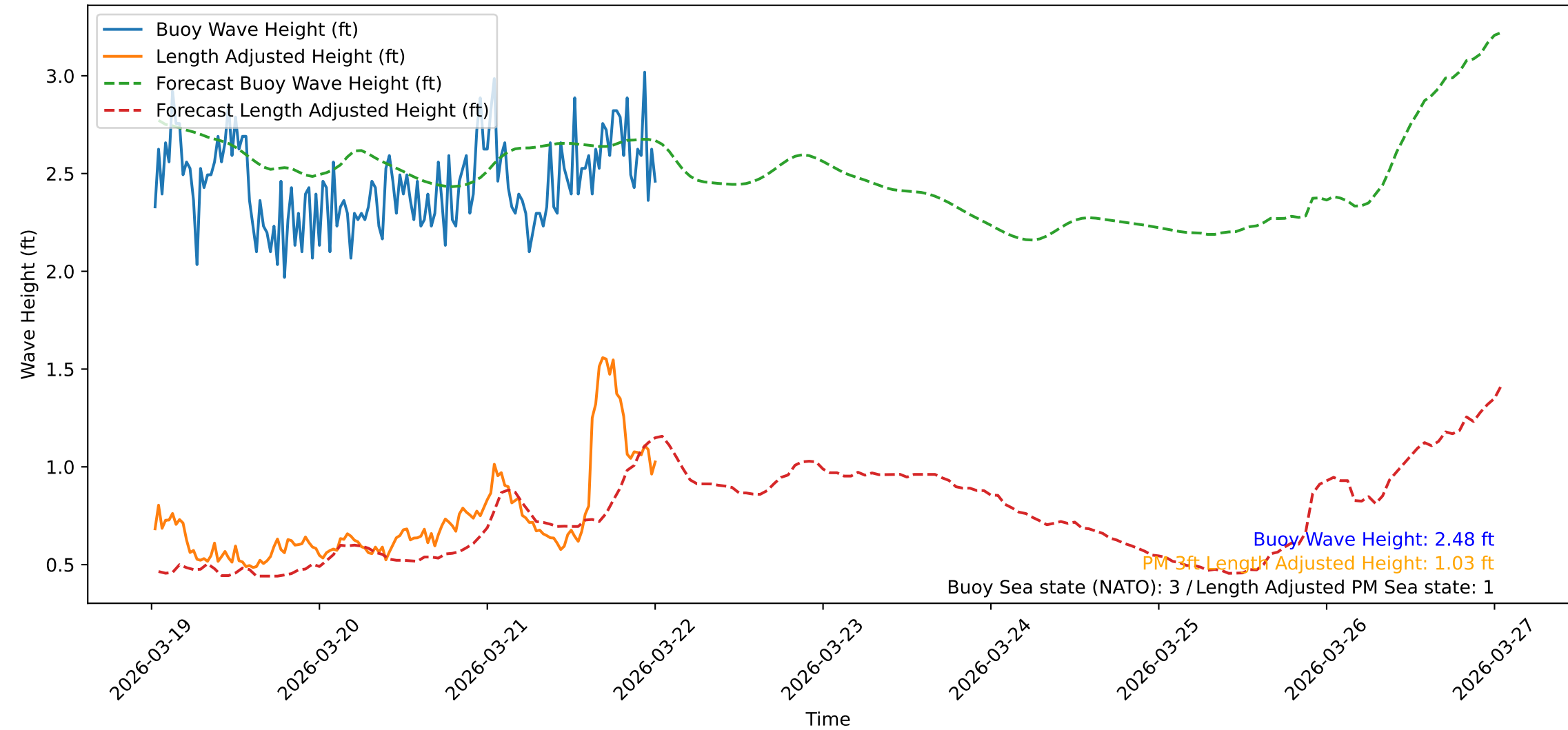
Wave Heights over Time for Oceanside Harbor at 2026-03-22 00:40:32
