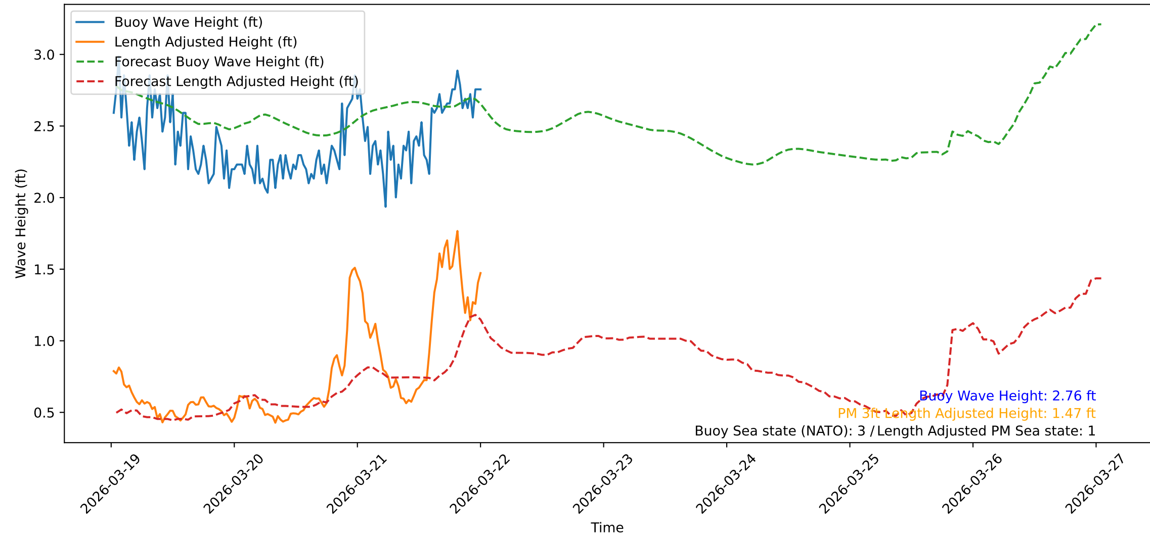
Wave Heights over Time for Green Beach at 2026-03-22 00:41:10
