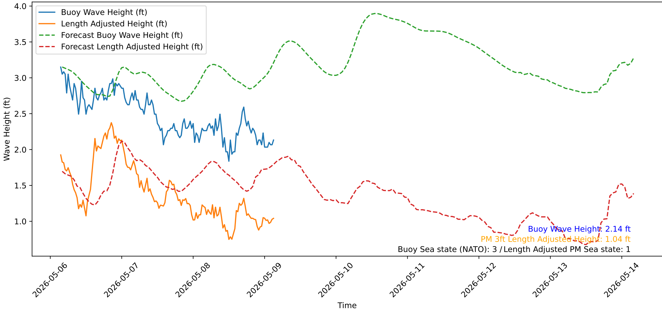
Wave Heights over Time for Green Beach at 2026-05-09 03:41:13
