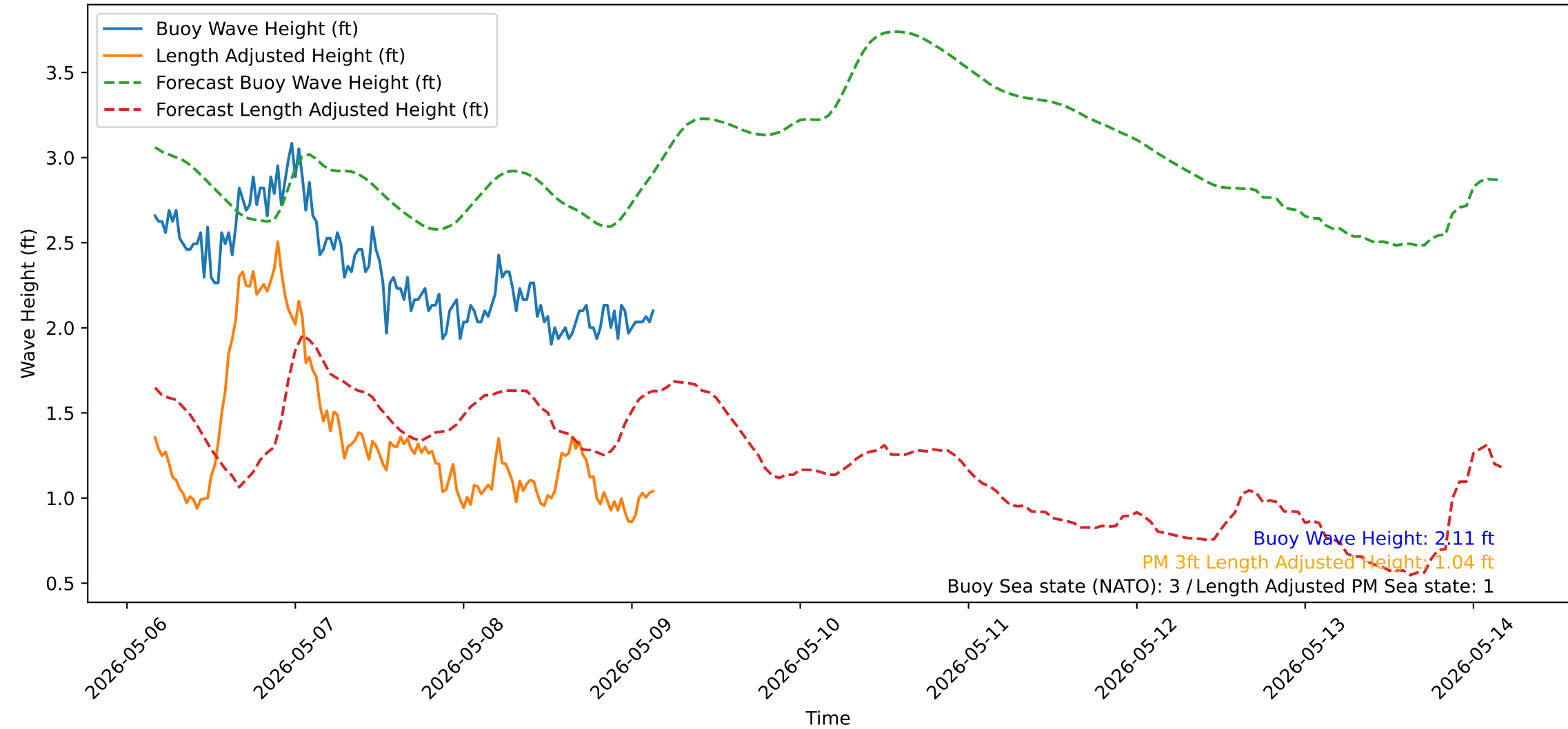
Wave Heights over Time for Red Beach at 2026-05-09 03:40:51
