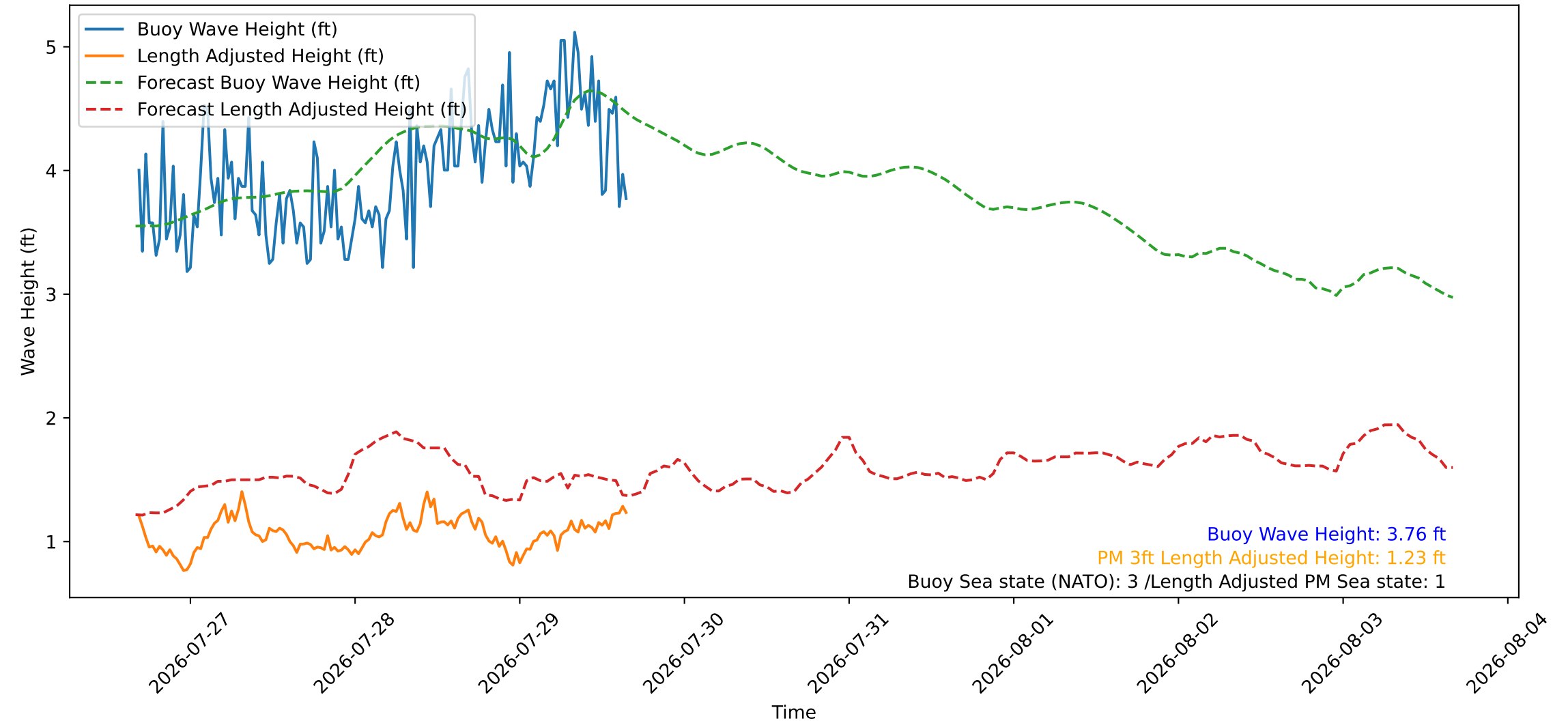
Wave Heights over Time for Red Beach at 2026-07-29 16:20:47
