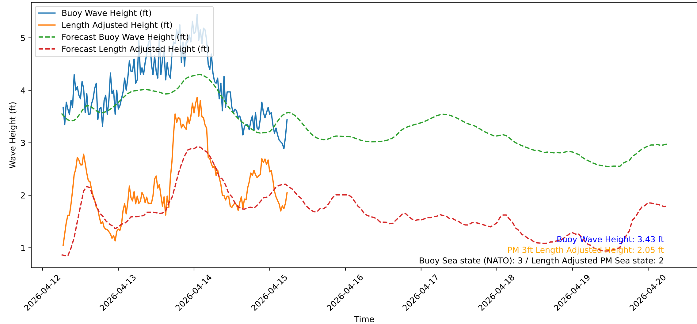
Wave Heights over Time for Oceanside Harbor at 2026-04-15 06:20:31
