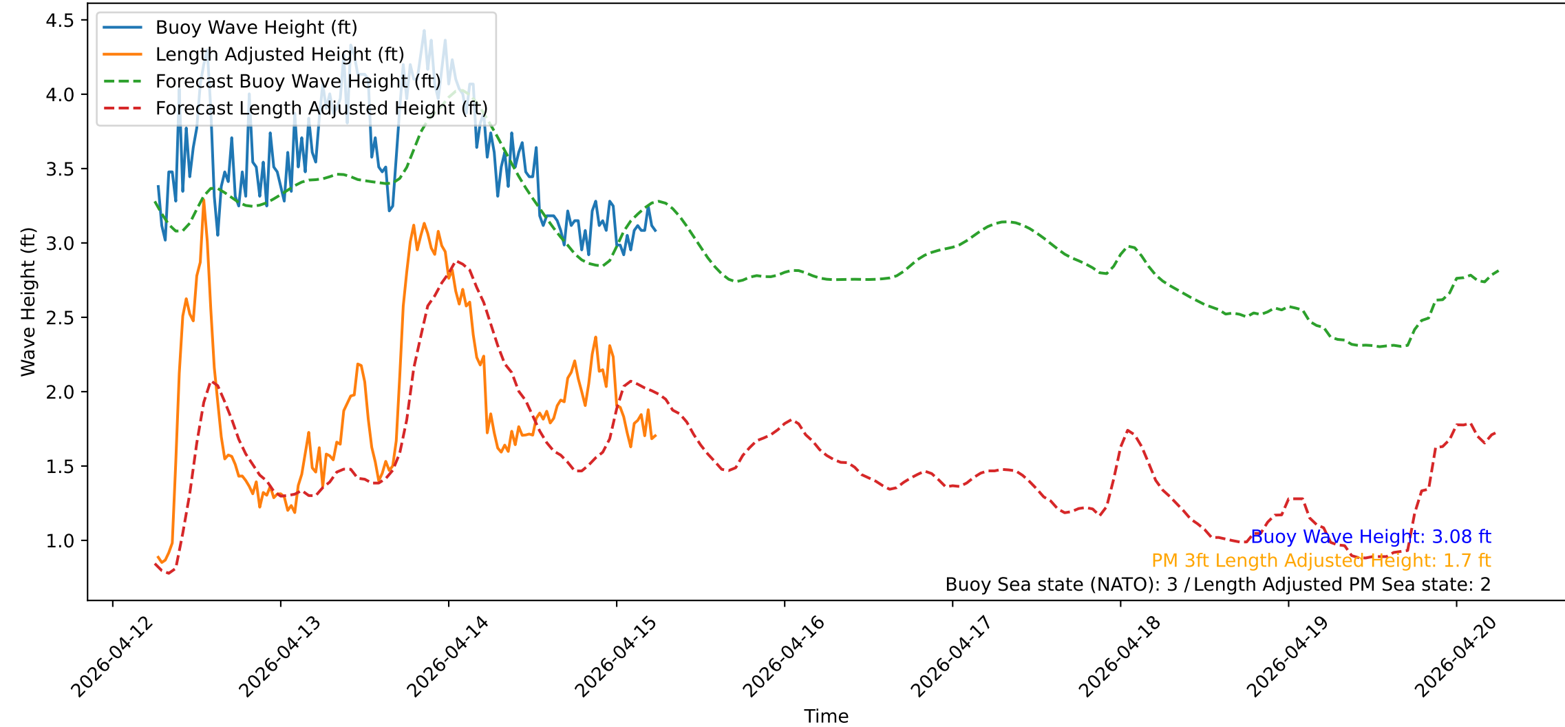
Wave Heights over Time for Red Beach at 2026-04-15 06:20:51
