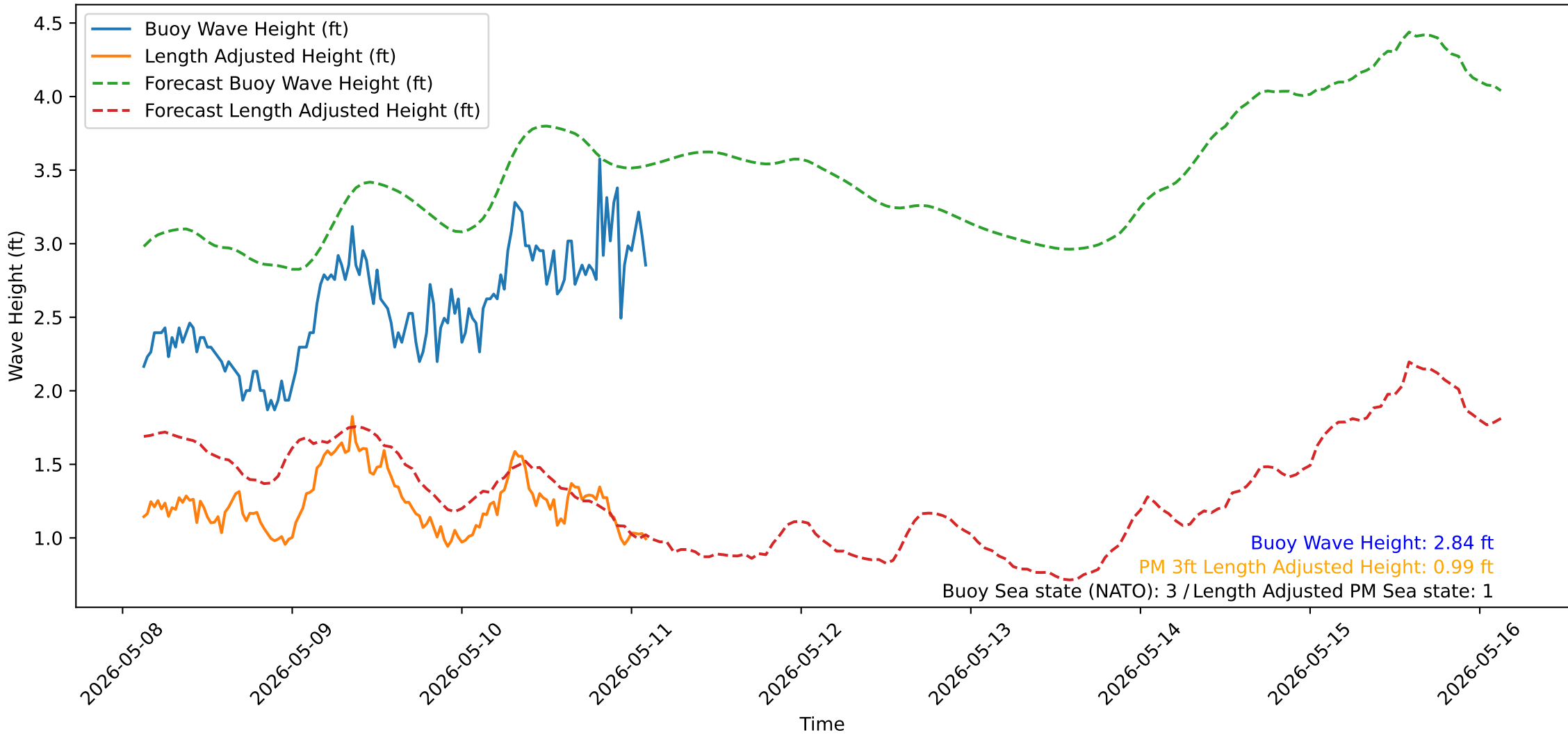
Wave Heights over Time for Oceanside Harbor at 2026-05-11 02:50:31
