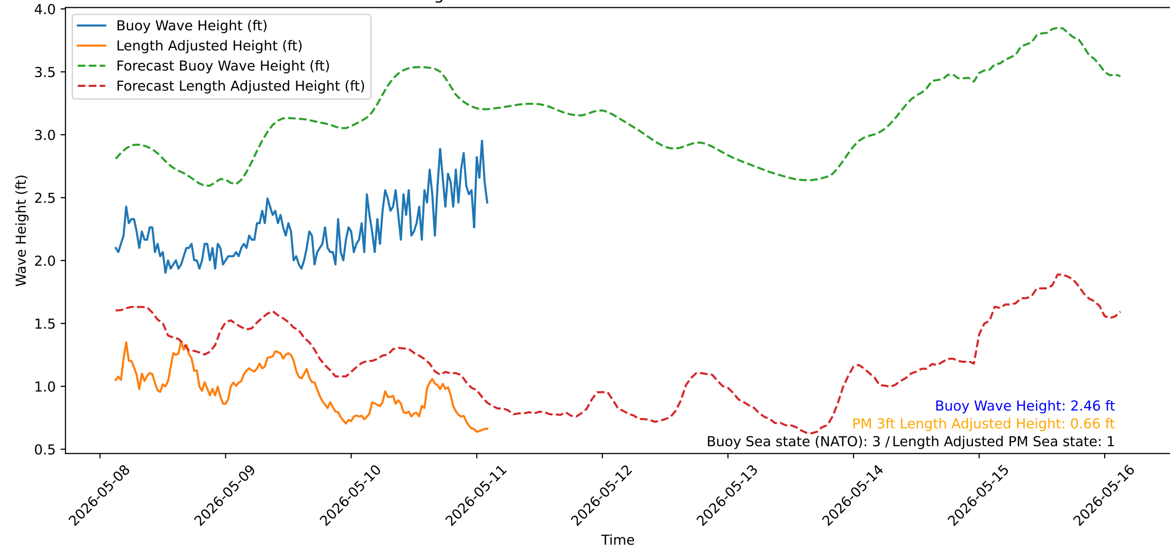
Wave Heights over Time for Red Beach at 2026-05-11 02:50:50
