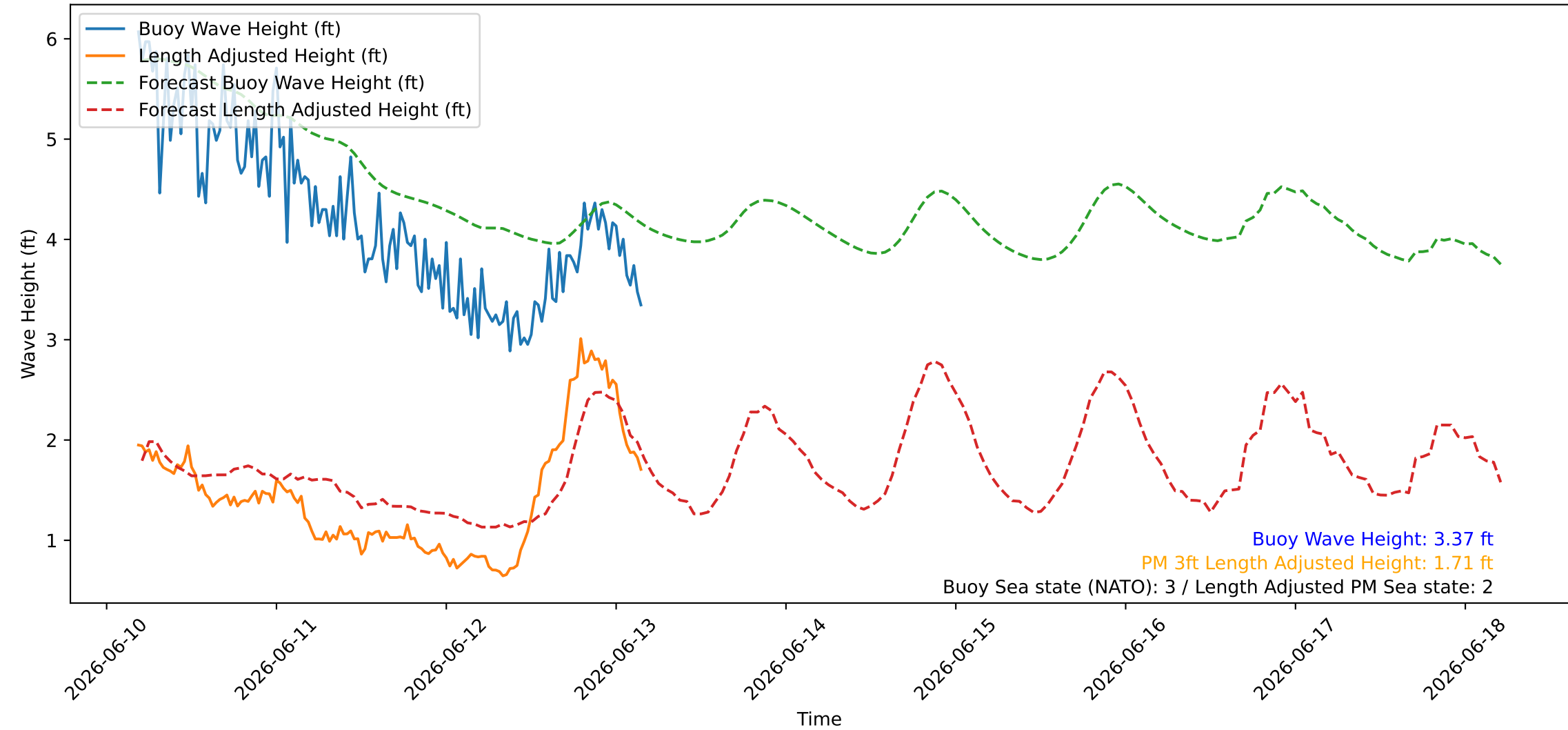
Wave Heights over Time for Green Beach at 2026-06-13 04:41:08
