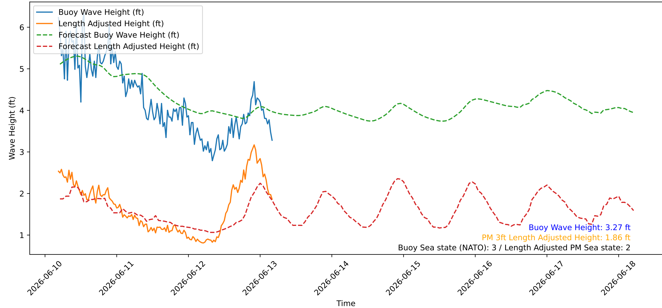
Wave Heights over Time for Oceanside Harbor at 2026-06-13 04:40:26
