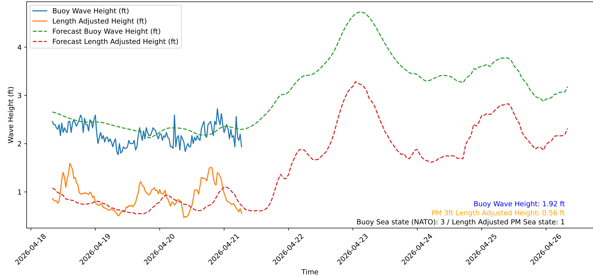
Wave Heights over Time for Red Beach at 2026-04-21 07:30:52
