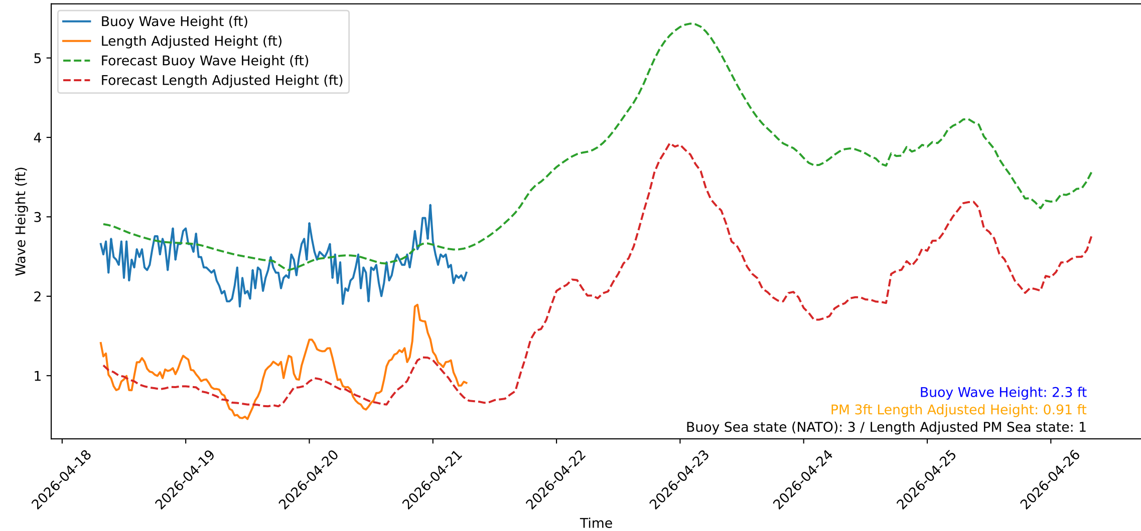
Wave Heights over Time for Green Beach at 2026-04-21 07:31:14
