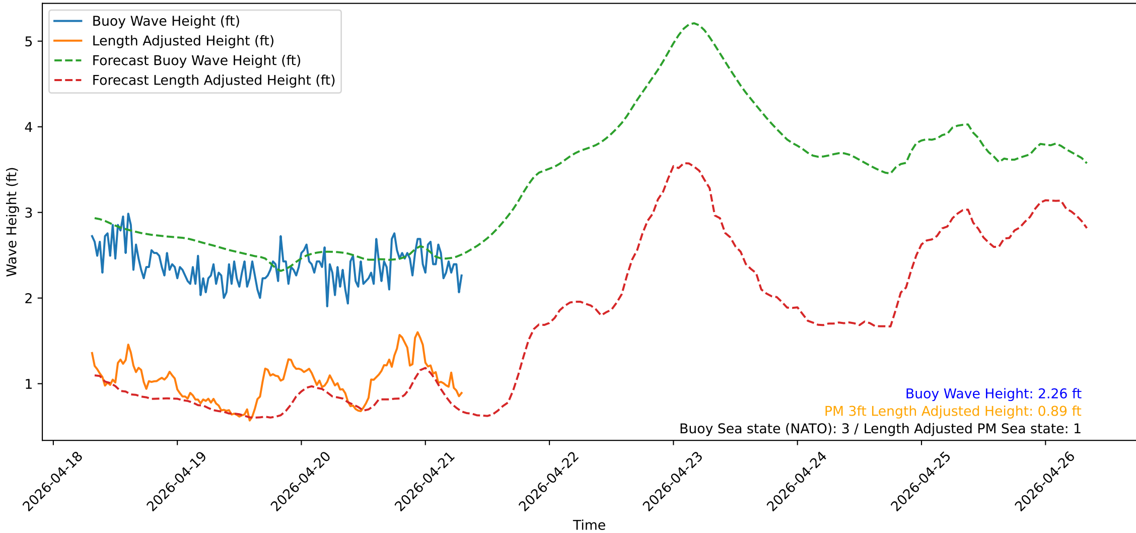
Wave Heights over Time for Oceanside Harbor at 2026-04-21 07:30:32
