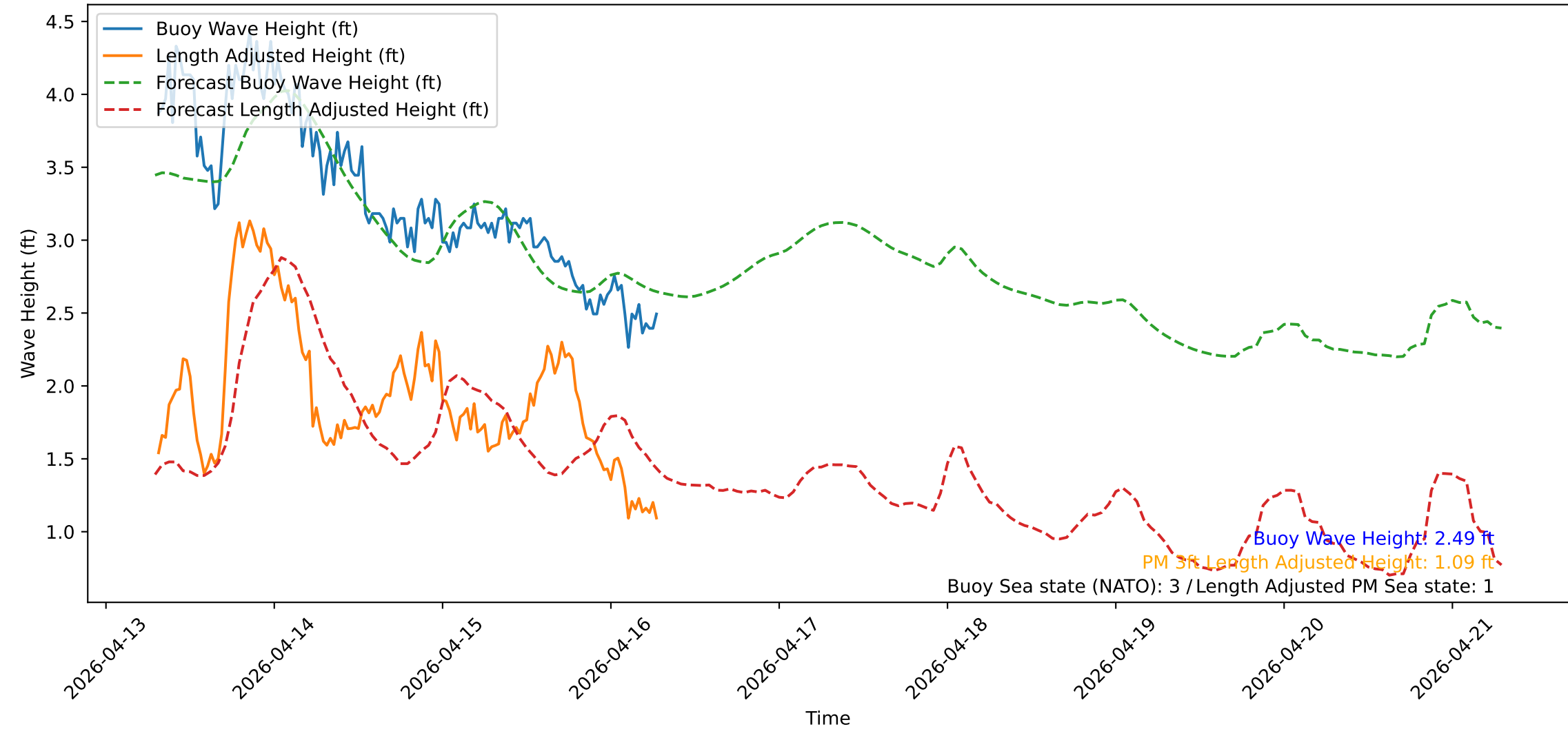
Wave Heights over Time for Red Beach at 2026-04-16 07:20:51
