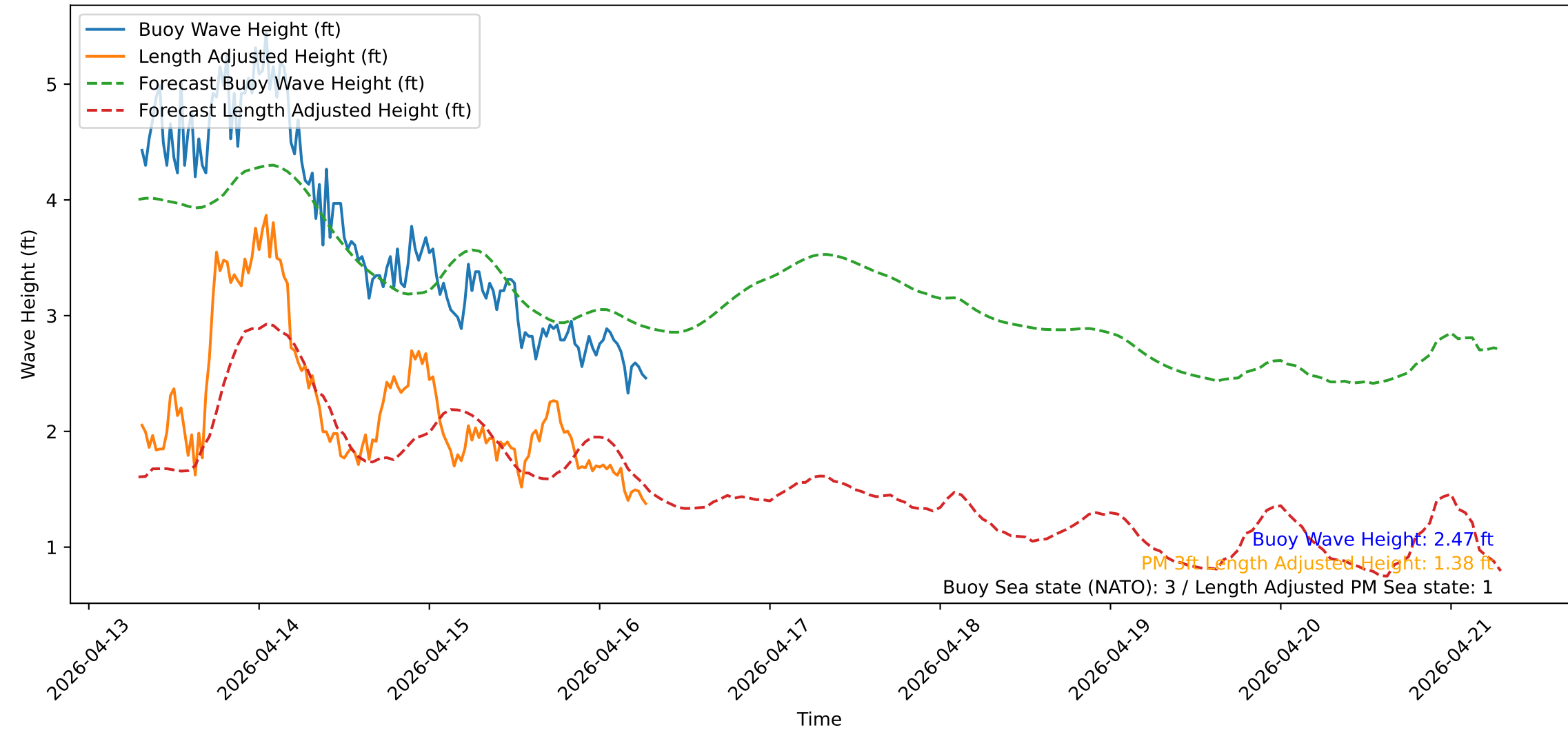
Wave Heights over Time for Oceanside Harbor at 2026-04-16 07:20:31
