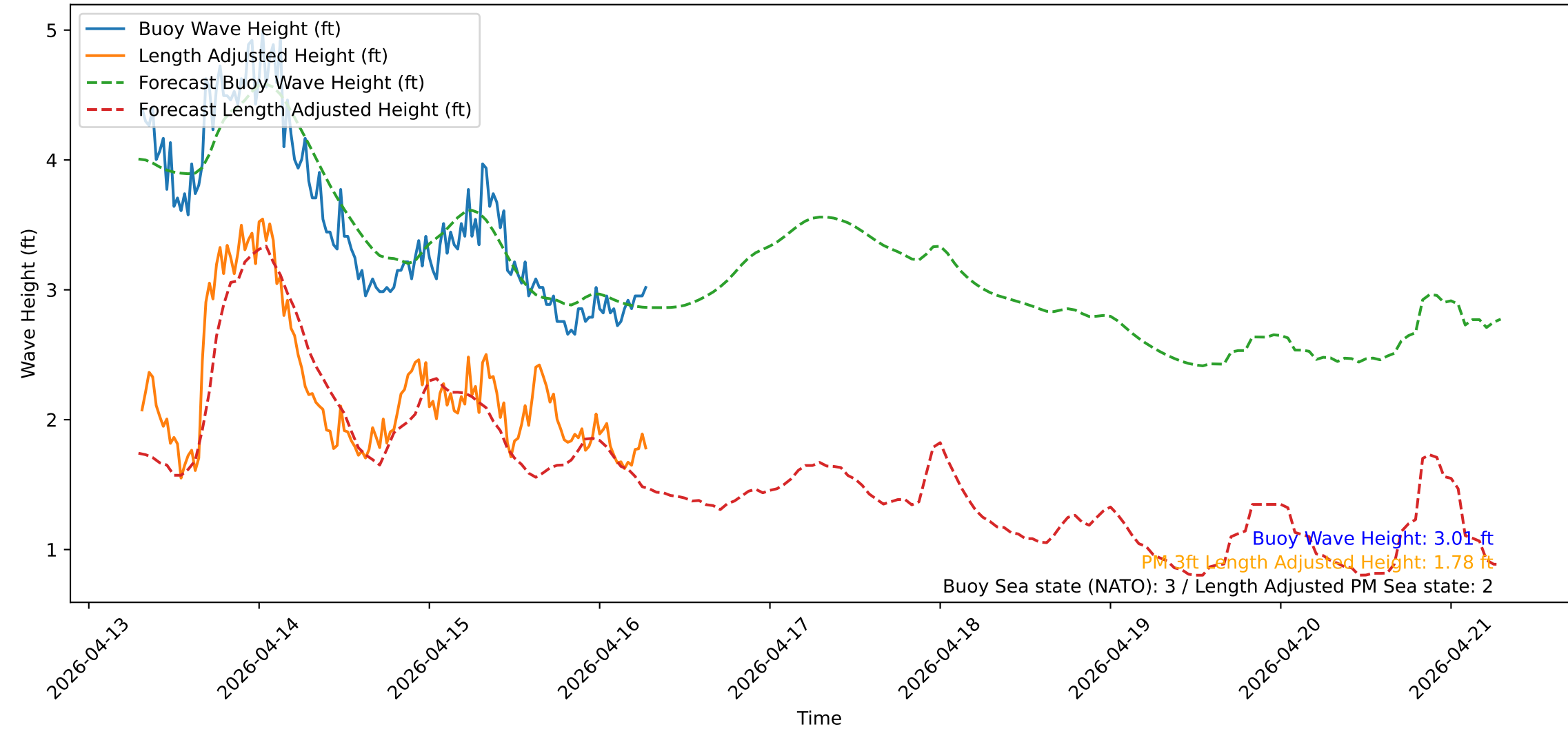
Wave Heights over Time for Green Beach at 2026-04-16 07:21:15
