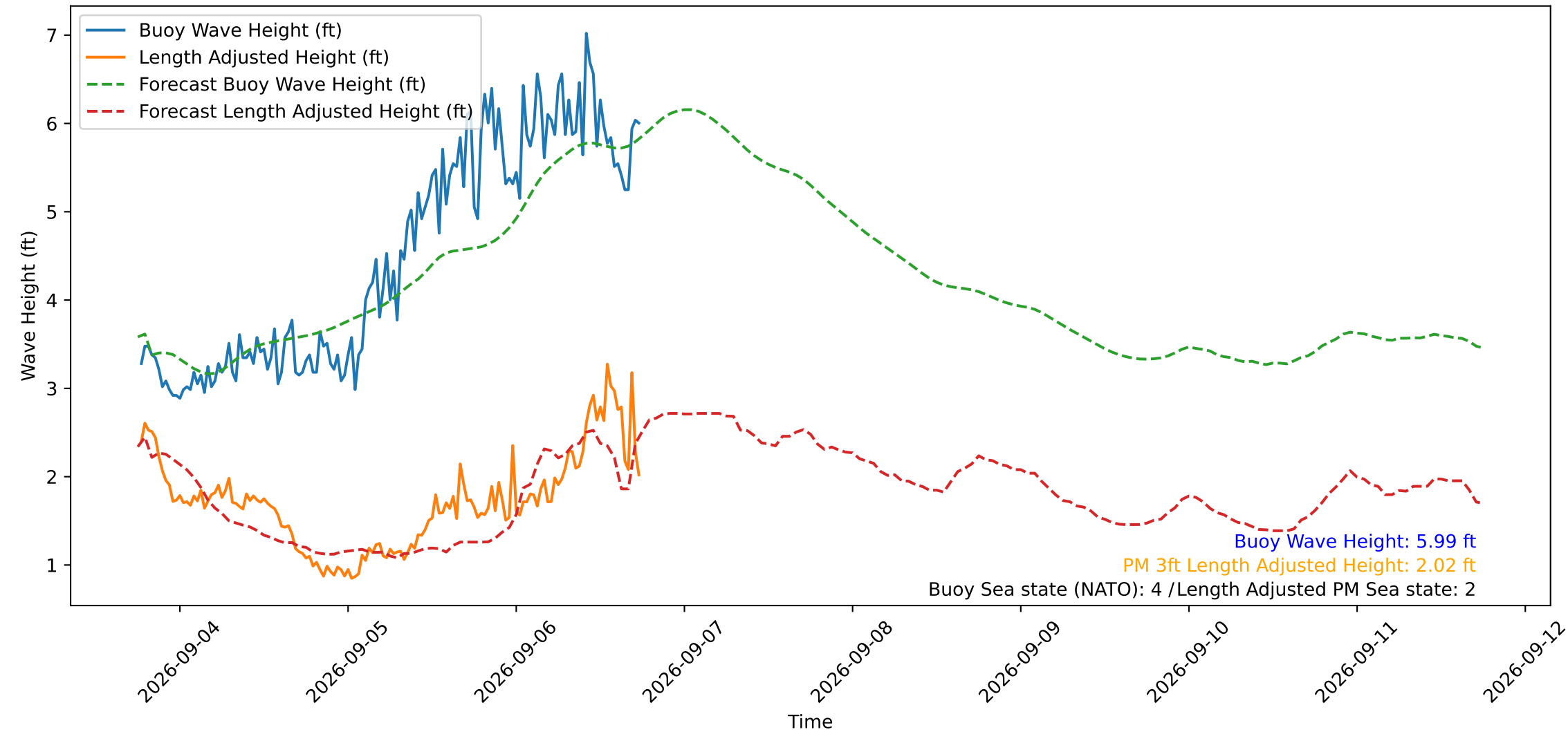
Wave Heights over Time for Oceanside Harbor at 2026-09-06 18:20:29
