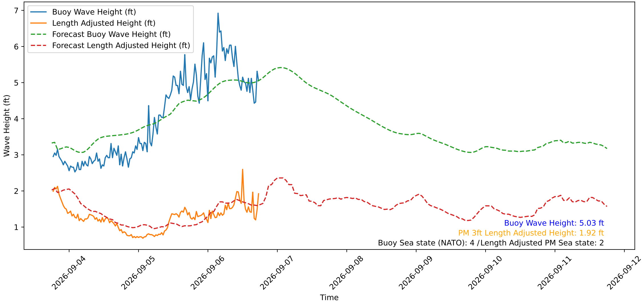
Wave Heights over Time for Red Beach at 2026-09-06 18:20:50
